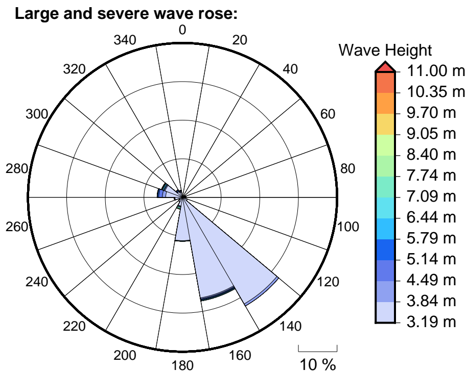
Figure 6 Large, severe and extreme wave roses for Fugro Wave Buoy 2
