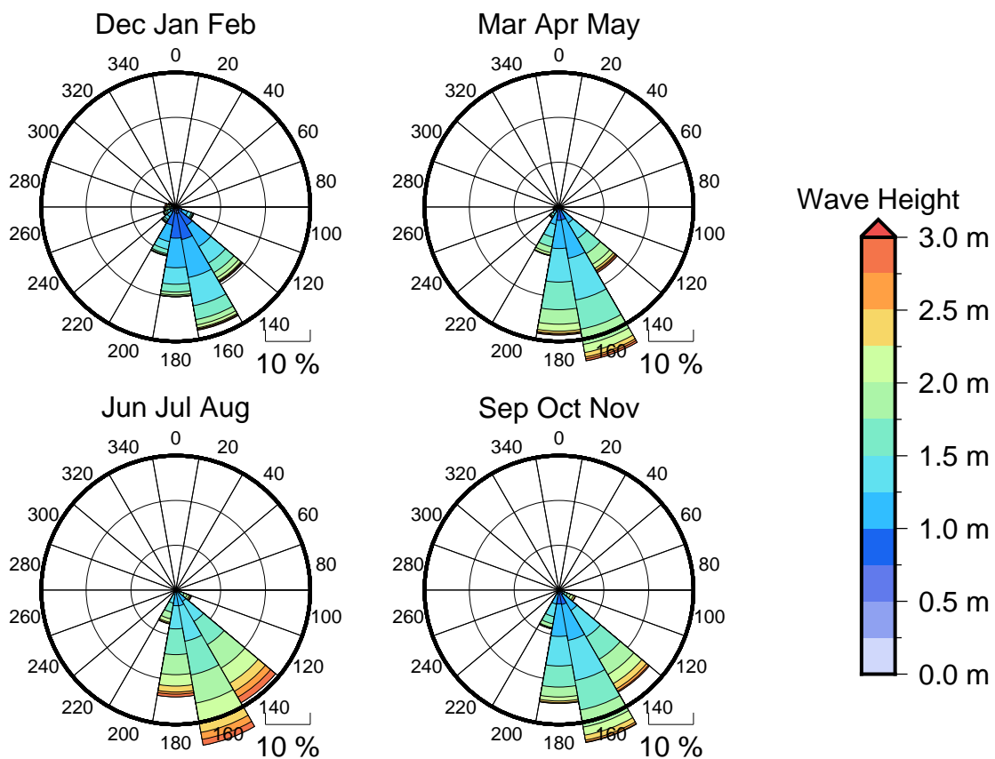
Figure 3 Seasonal wave roses for Fugro Wave Buoy 2
