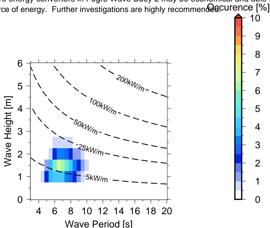
Figure 10 Occurences of sea states in Fugro Wave Buoy 2 .
