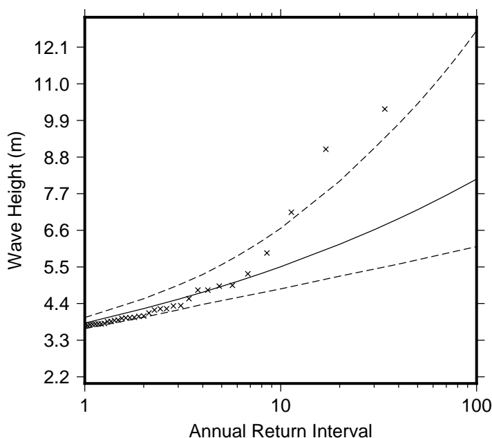
Figure 9 Extreme wave distribution for Fugro Wave Buoy 2. The crosses represents the wave events that occurred since 1979. The plain line is the statistical distribution that best fit the past wave events. The dotted line show the upper and lower high confidence of the fit, there is a 95% chance that the fitted distribution lie between the two dashed lines.
