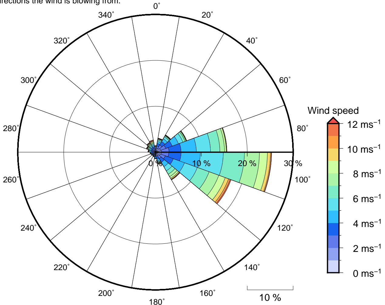
Figure 11 Annual wind rose for Fugro Wave Buoy 2. Note that directions are where the wind is coming from.
