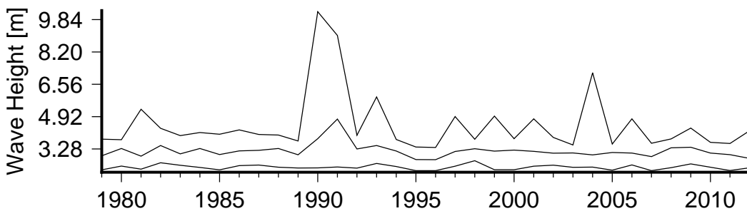
Figure 8 Annual variation in large waves (90th percentile)(lower curve), severe waves (99th percentile) (middle curve) and the largest wave(upper curve) in Fugro Wave Buoy 2.
