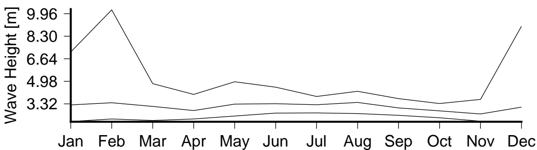
Figure 7 Monthly variation in large waves (90th percentile)(lower curve), severe waves (99th percentile) (middle curve) and the largest wave(upper curve) in Fugro Wave Buoy 2.
