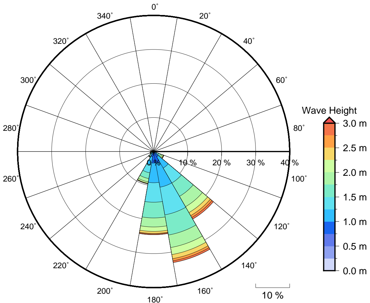
Figure 2 Annual wave rose for Fugro Wave Buoy 2. Note that direction are where the wave are coming from.
