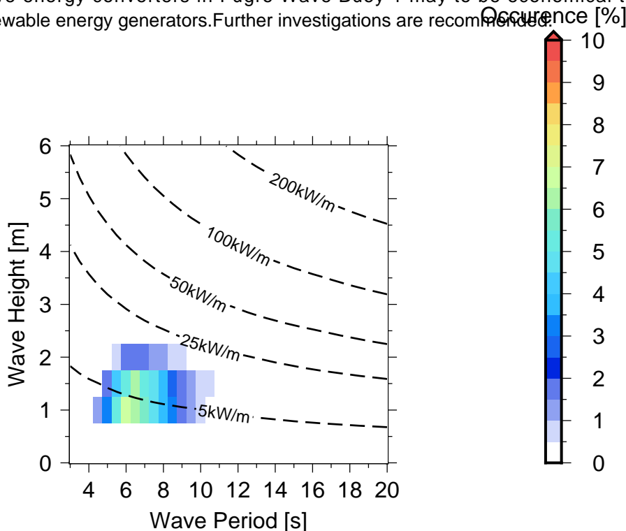
Figure 10 Occurences of sea states in Fugro Wave Buoy 1 .
