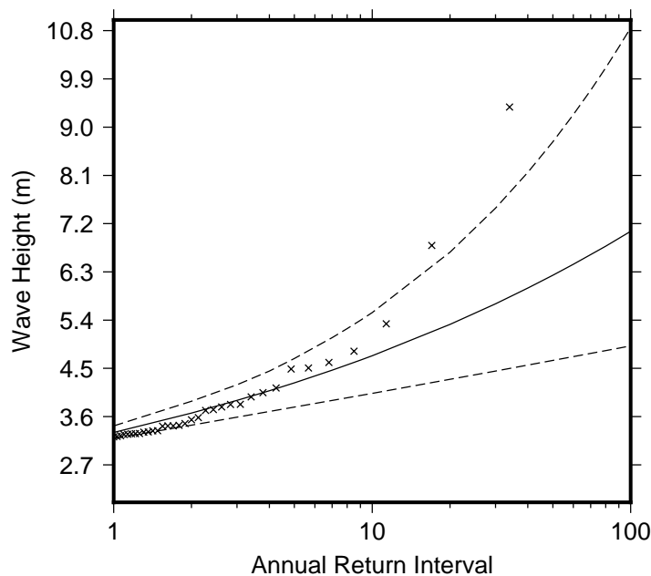
Figure 9 Extreme wave distribution for Fugro Wave Buoy 1. The crosses represents the wave events that occurred since 1979. The plain line is the statistical distribution that best fit the past wave events. The dotted line show the upper and lower high confidence of the fit, there is a 95% chance that the fitted distribution lie between the two dashed lines.
