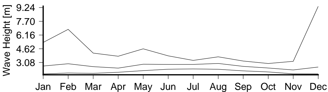
Figure 7 Monthly variation in large waves (90th percentile)(lower curve), severe waves (99th percentile) (middle curve) and the largest wave(upper curve) in Fugro Wave Buoy 1.
