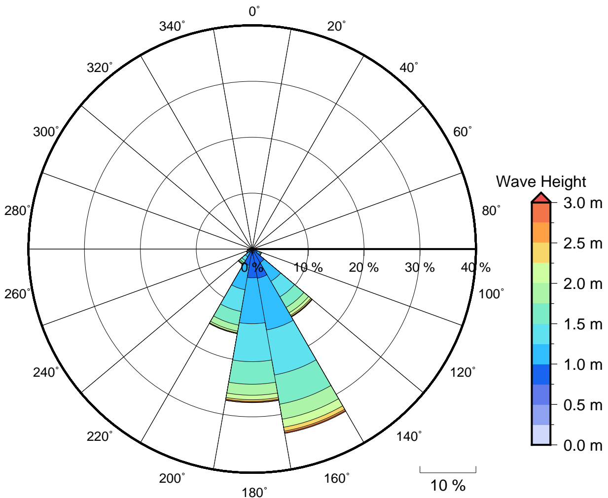
Figure 2 Annual wave rose for Fugro Wave Buoy 1. Note that direction are where the wave are coming from.
