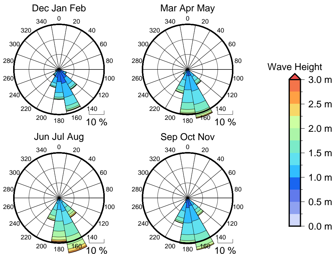
Figure 3 Seasonal wave roses for Fugro Wave Buoy 1
