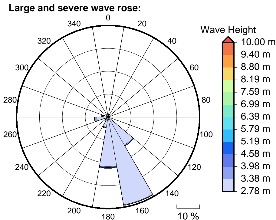
Figure 6 Large, severe and extreme wave roses for Fugro Wave Buoy 1
