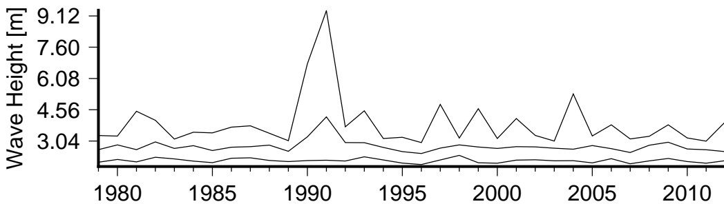
Figure 8 Annual variation in large waves (90th percentile)(lower curve), severe waves (99th percentile) (middle curve) and the largest wave(upper curve) in Fugro Wave Buoy 1.
