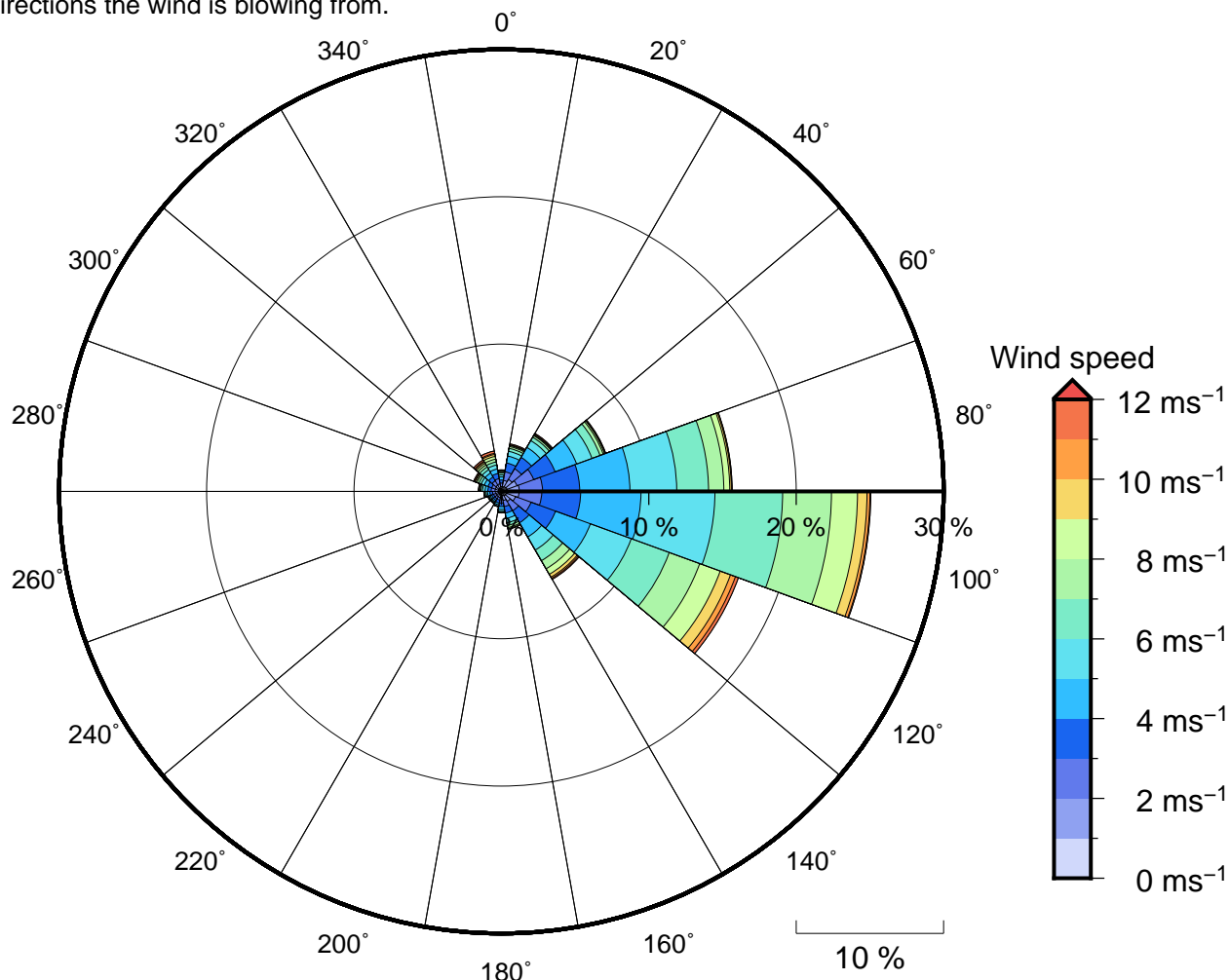
Figure 11 Annual wind rose for Fugro Wave Buoy 1. Note that directions are where the wind is coming from.
