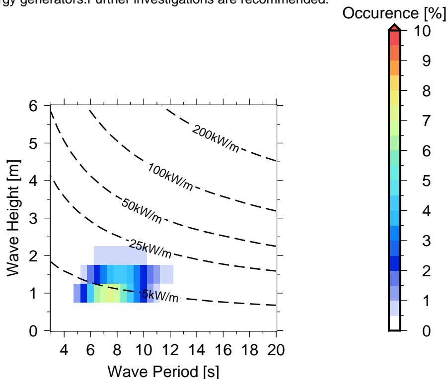
Figure 10 Occurences of sea states in Cape Mulinu'u .
