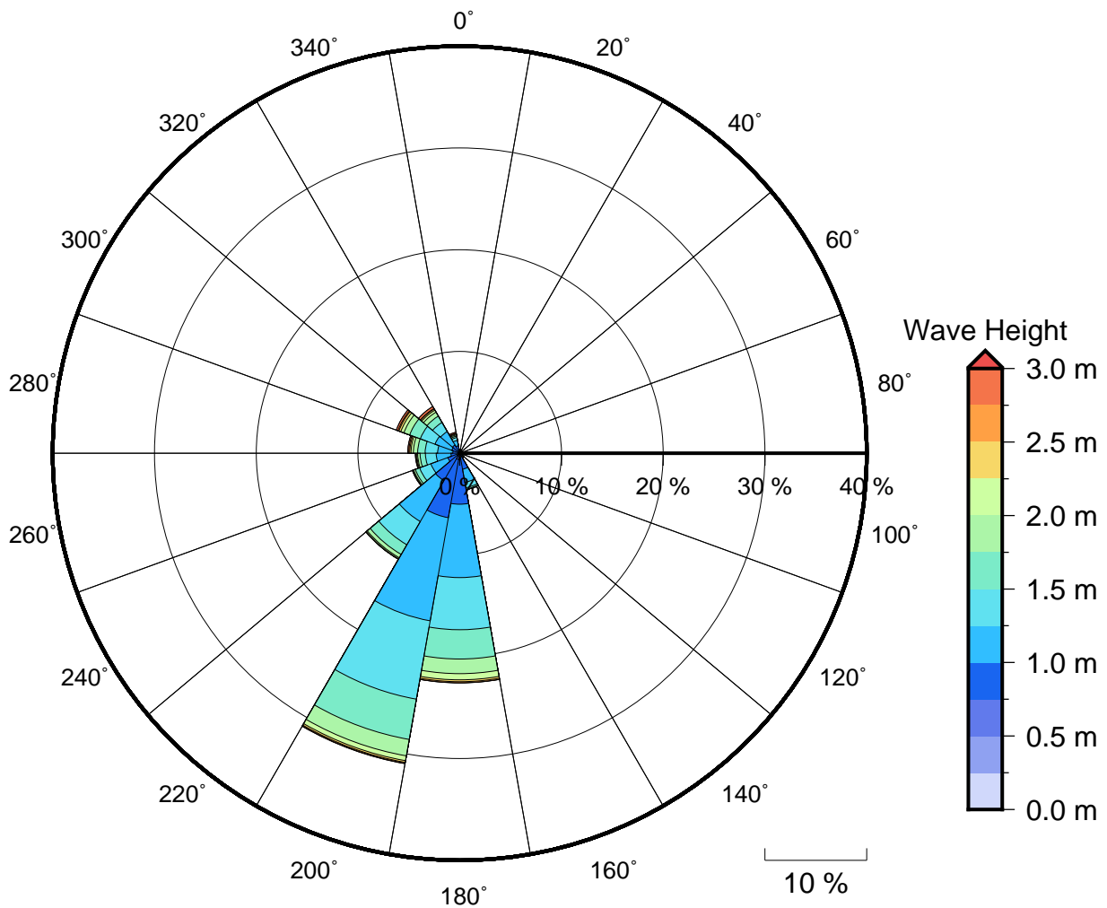
Figure 2 Annual wave rose for Cape Mulinu'u. Note that direction are where the wave are coming from .
