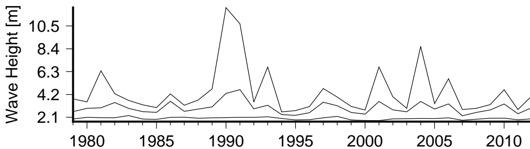
Figure 8 Annual variation in large waves (90th percentile)(lower curve), severe waves (99th percentile) (middle curve) and the largest wave(upper curve) in Cape Mulinu'u.
