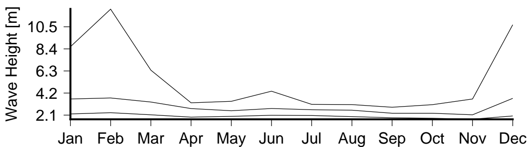
Figure 7 Monthly variation in large waves (90th percentile)(lower curve), severe waves (99th percentile) (middle curve) and the largest wave(upper curve) in Cape Mulinu'u.
