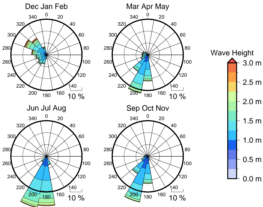
Figure 3 Seasonal wave roses for Cape Mulinu'u
