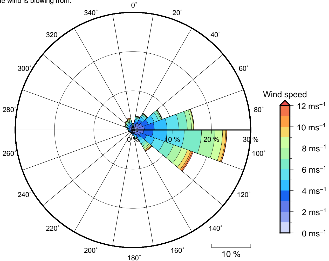
Figure 11 Annual wind rose for Cape Mulinu'u. Note that directions are where the wind is coming from.
