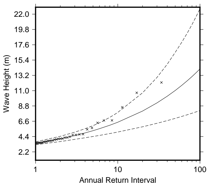
Figure 9 Extreme wave distribution for Cape Mulinu'u. The crosses represents the wave events that occurred since 1979. The plain line is the statistical distribution that best fit the past wave events. The dotted line show the upper and lower high confidence of the fit, there is a 95% chance that the fitted distribution lie between the two dashed lines.
