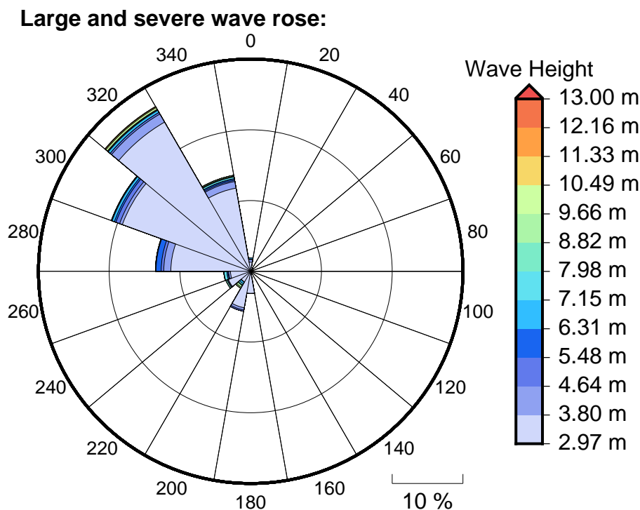
Figure 6 Large, severe and extreme wave roses for Cape Mulinu'u
