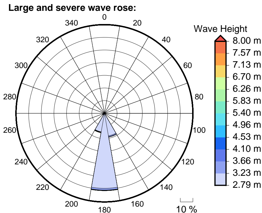
Figure 6 Large, severe and extreme wave roses for Satupaitea
