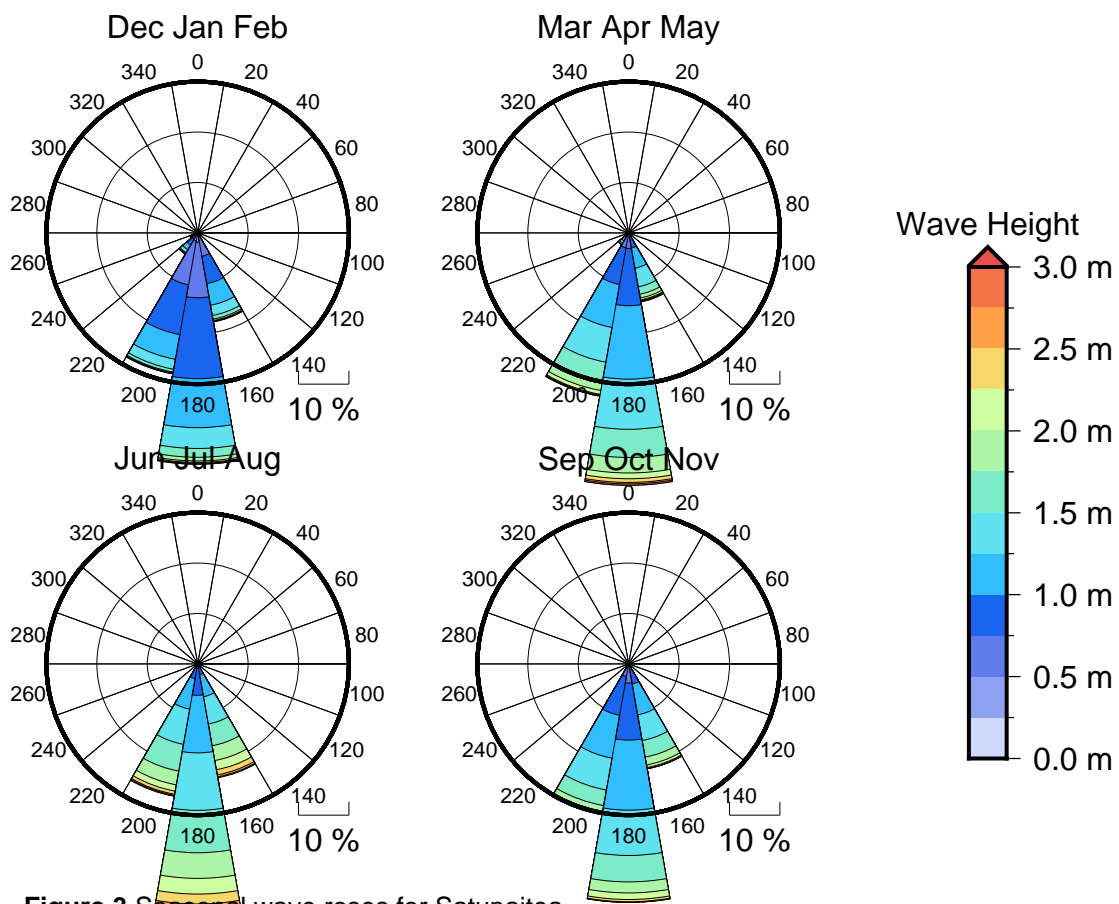
Figure 3 Seasonal wave roses for Satupaitea
