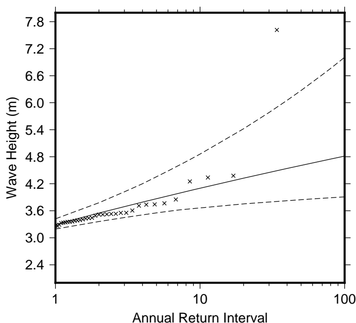
Figure 9 Extreme wave distribution for Satupaitea. The crosses represents the wave events that occurred since 1979. The plain line is the statistical distribution that best fit the past wave events. The dotted line show the upper and lower high confidence of the fit, there is a 95% chance that the fitted distribution lie between the two dashed lines.
