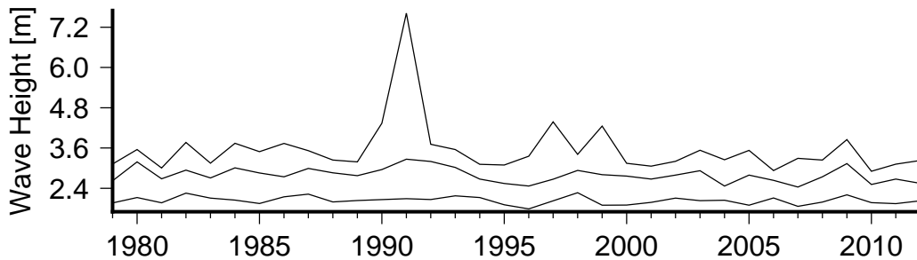
Figure 8 Annual variation in large waves (90th percentile)(lower curve), severe waves (99th percentile) (middle curve) and the largest wave(upper curve) in Satupaitea.
