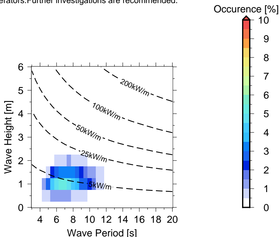
Figure 10 Occurrences of sea states in Satupaitea .
