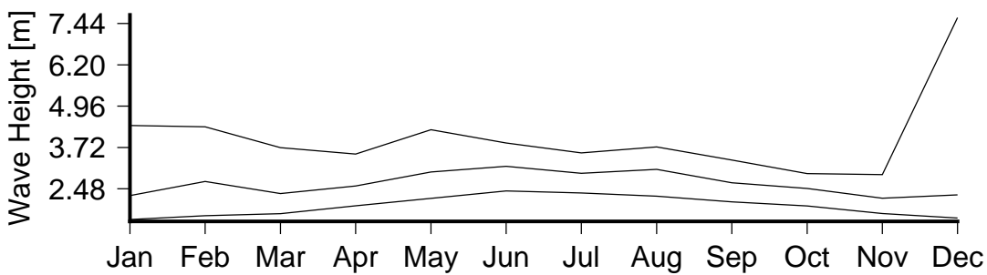
Figure 7 Monthly variation in large waves (90th percentile)(lower curve), severe waves (99th percentile) (middle curve) and the largest wave(upper curve) in Satupaitea.
