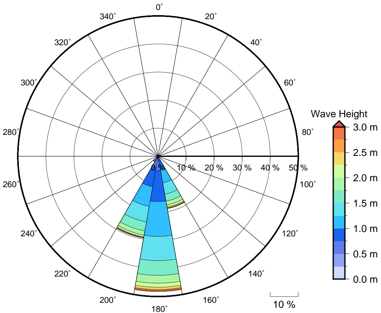
Figure 2 Annual wave rose for Satupaitea. Note that direction are where the wave are coming from.
