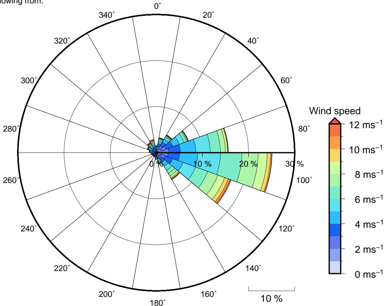
Figure 11 Annual wind rose for Satupaitea. Note that directions are where the wind is coming from.
