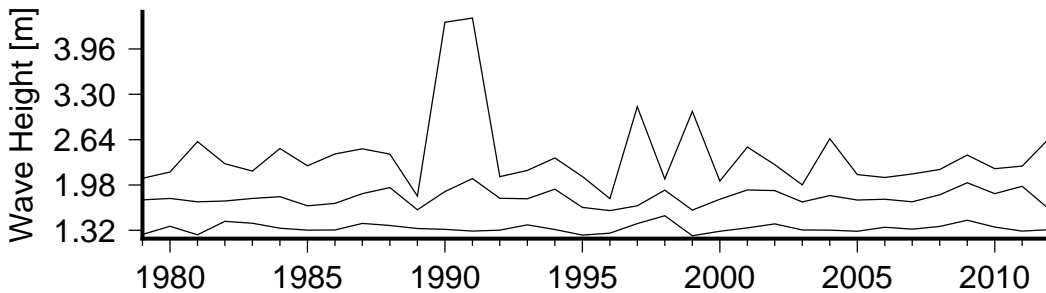
Figure 8 Annual variation in large waves (90th percentile)(lower curve), severe waves (99th percentile) (middle curve) and the largest wave(upper curve) in Salelologa Passage.
