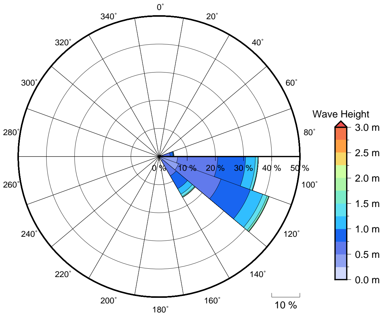
Figure 2 Annual wave rose for Salelologa Passage. Note that direction are where the wave are coming from.
