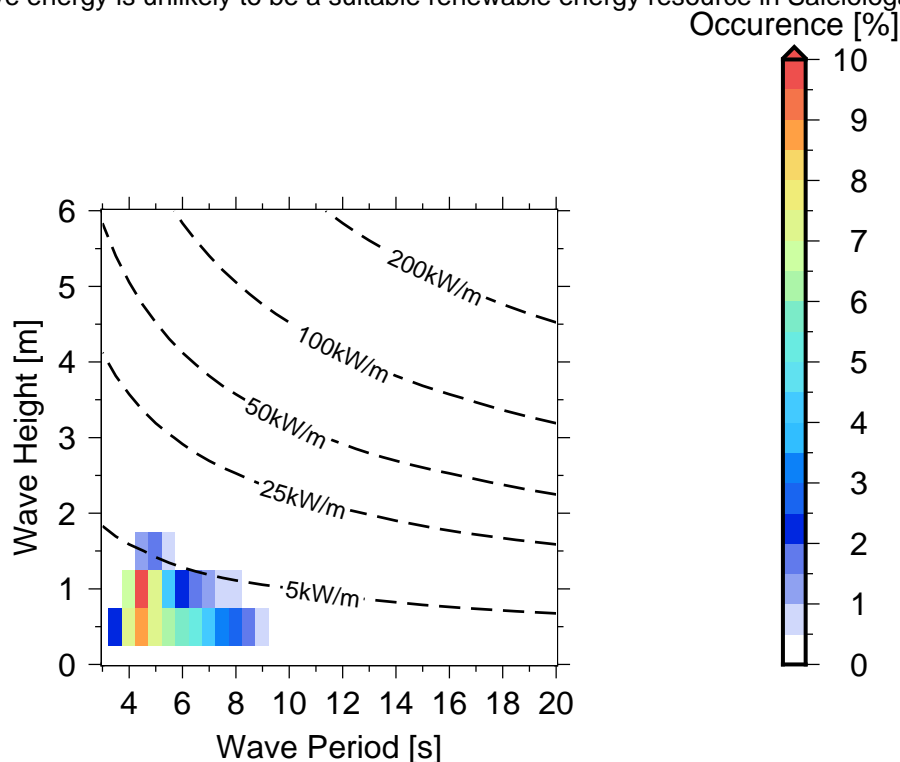
Figure 10 Occurrences of sea states in Salelologa Passage .
