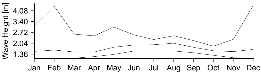
Figure 7 Monthly variation in large waves (90th percentile)(lower curve), severe waves (99th percentile) (middle curve) and the largest wave(upper curve) in Salelologa Passage.
