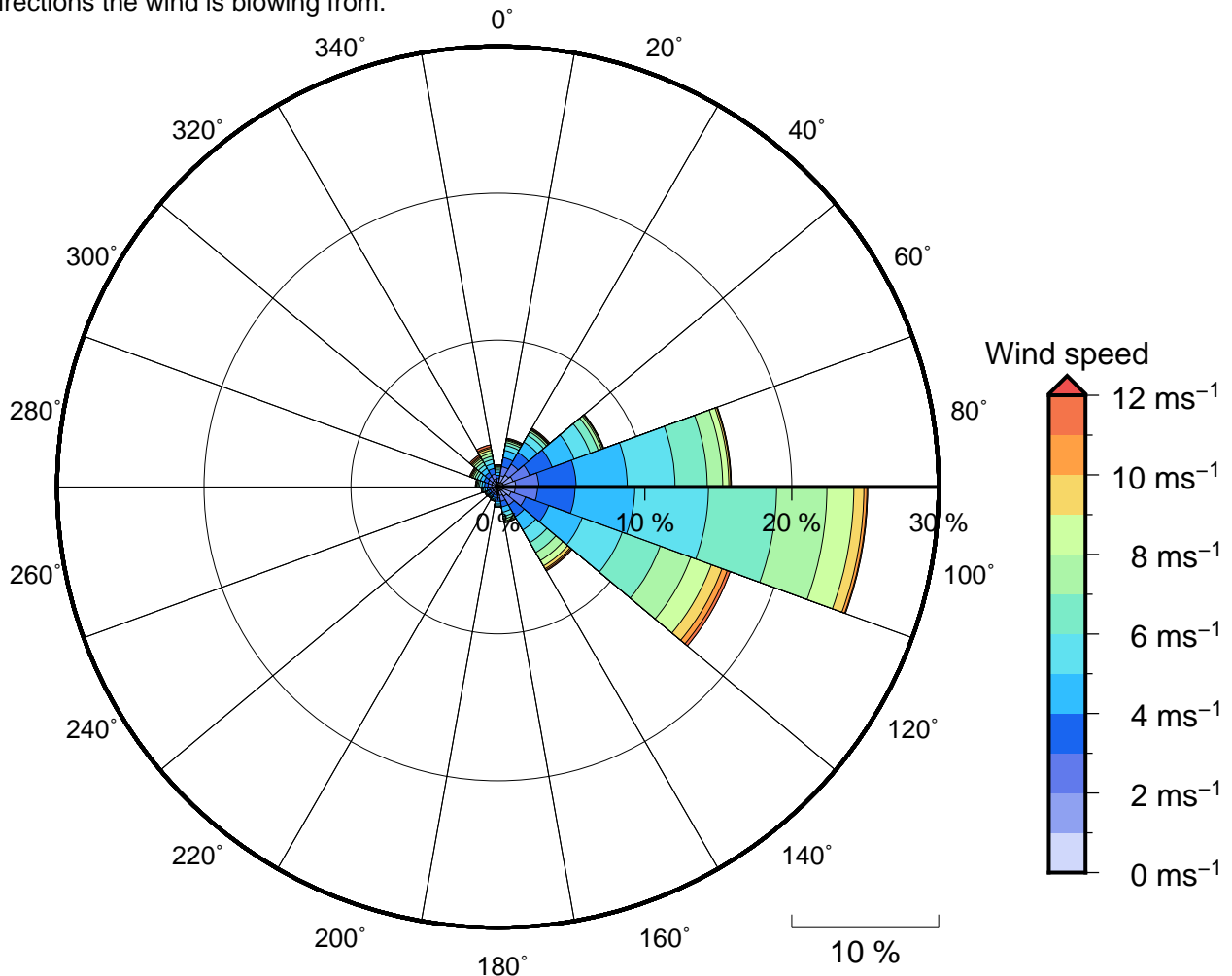
Figure 11 Annual wind rose for Salelologa Passage. Note that directions are where the wind is coming from.
