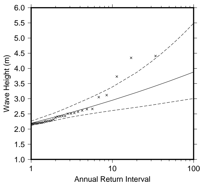
Figure 9 Extreme wave distribution for Salelologa Passage. The crosses represents the wave events that occurred since 1979. The plain line is the statistical distribution that best fit the past wave events. The dotted line show the upper and lower high confidence of the fit, there is a 95% chance that the fitted distribution lie between the two dashed lines.
