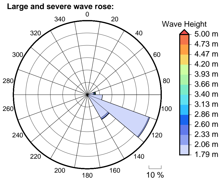
Figure 6 Large, severe and extreme wave roses for Salelologa Passage
