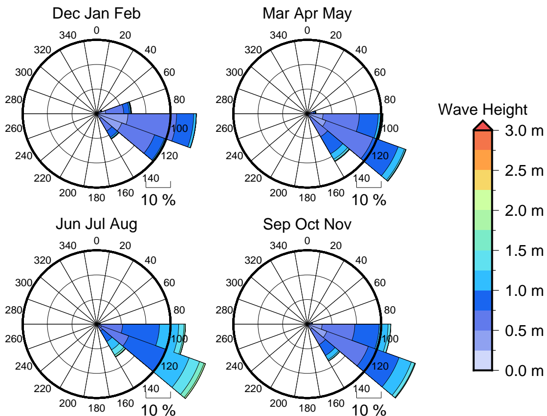
Figure 3 Seasonal wave roses for Salelologa Passage
