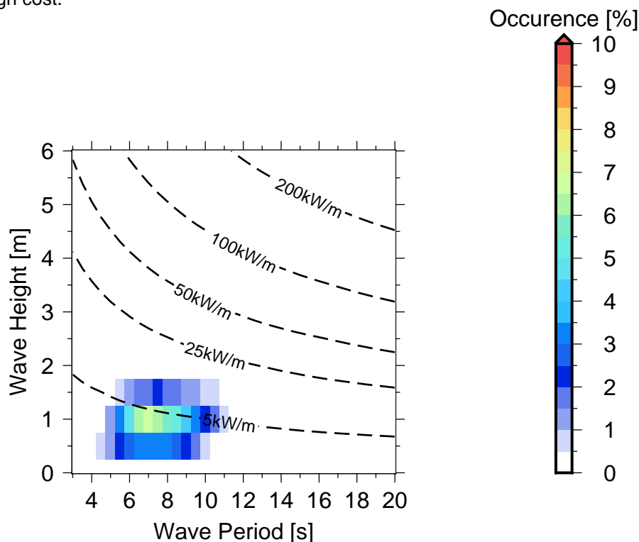
Figure 10 Occurrences of sea states in Salani .
