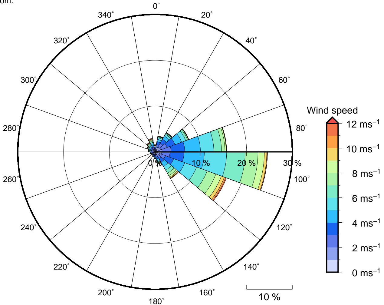
Figure 11 Annual wind rose for Salani. Note that directions are where the wind is coming from .
