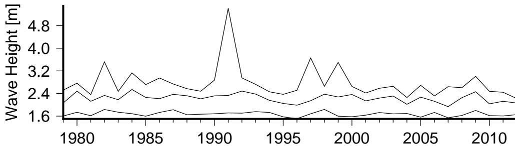
Figure 8 Annual variation in large waves (90th percentile)(lower curve), severe waves (99th percentile) (middle curve) and the largest wave(upper curve) in Salani.
