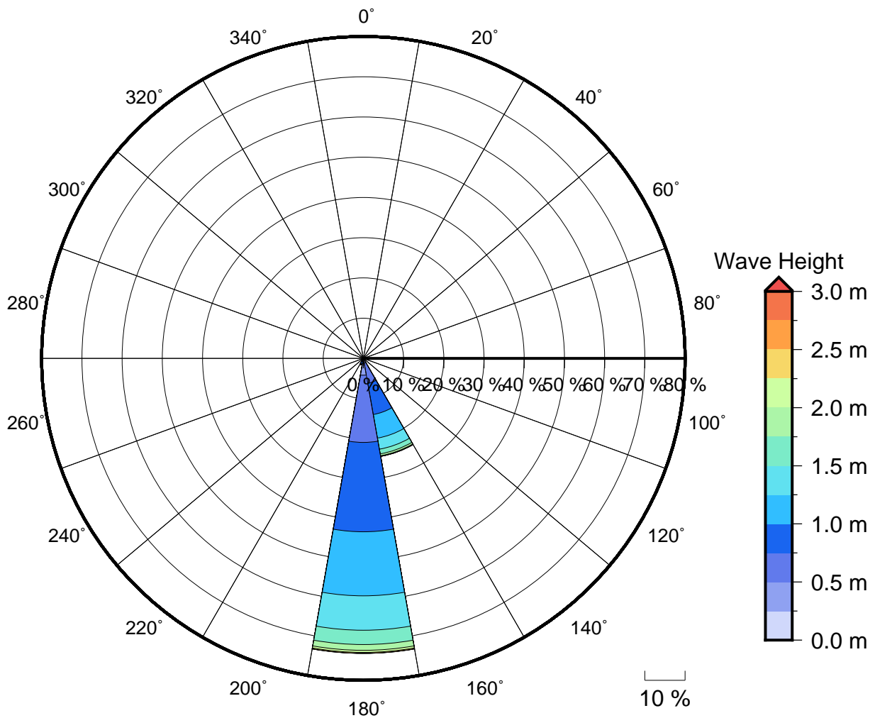
Figure 2 Annual wave rose for Salani. Note that direction are where the wave are coming from.
