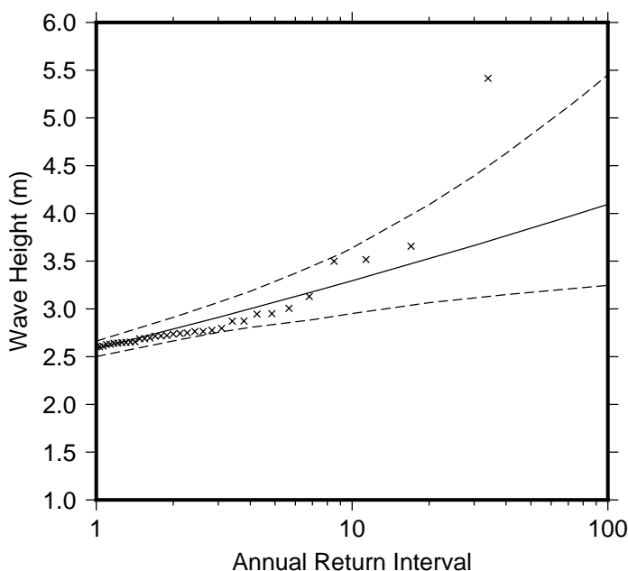
Figure 9 Extreme wave distribution for Salani. The crosses represents the wave events that occurred since 1979. The plain line is the statistical distribution that best fit the past wave events. The dotted line show the upper and lower high confidence of the fit, there is a 95% chance that the fitted distribution lie between the two dashed lines.
