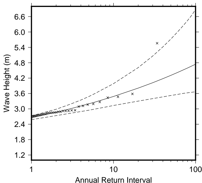
Figure 9 Extreme wave distribution for Safata Bay. The crosses represents the wave events that occurred since 1979. The plain line is the statistical distribution that best fit the past wave events. The dotted line show the upper and lower high confidence of the fit, there is a 95% chance that the fitted distribution lie between the two dashed lines.
