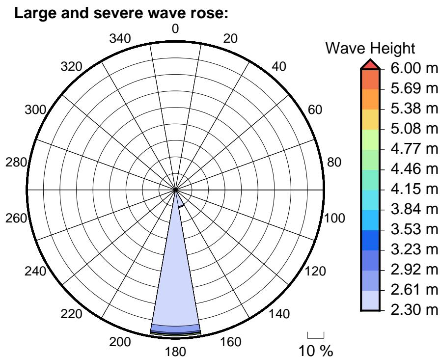
Figure 6 Large, severe and extreme wave roses for Safata Bay
