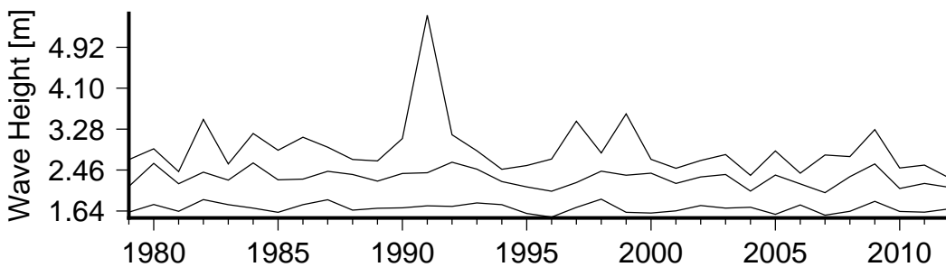
Figure 8 Annual variation in large waves (90th percentile)(lower curve), severe waves (99th percentile) (middle curve) and the largest wave(upper curve) in Safata Bay.
