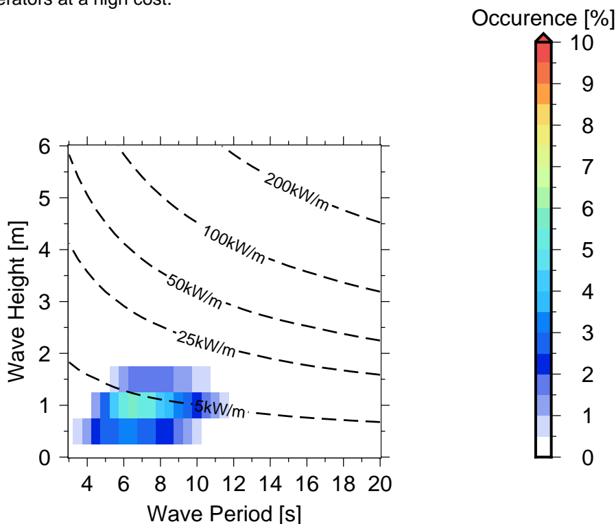
Figure 10 Occurences of sea states in Safata Bay .
