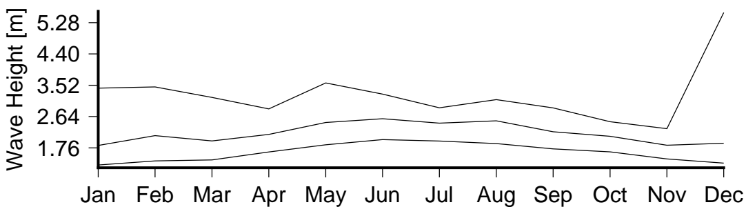
Figure 7 Monthly variation in large waves (90th percentile)(lower curve), severe waves (99th percentile) (middle curve) and the largest wave(upper curve) in Safata Bay.
