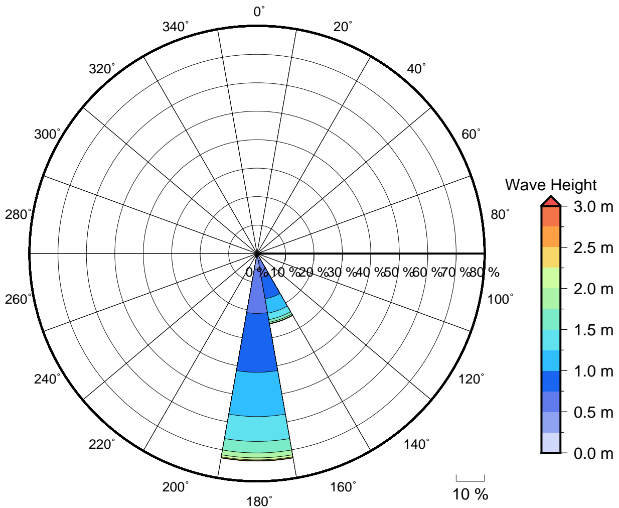
Figure 2 Annual wave rose for Safata Bay. Note that direction are where the wave are coming from.
