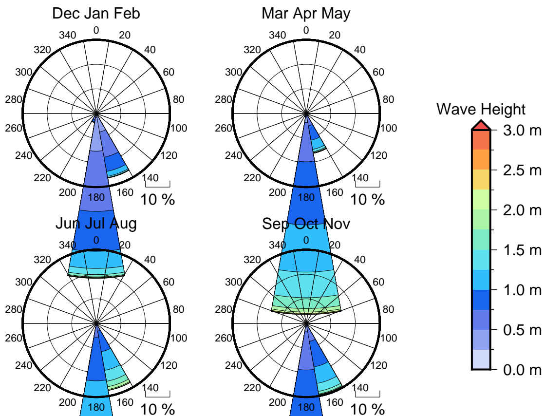
Figure 3 Seasonal wave roses for Safata Bay
