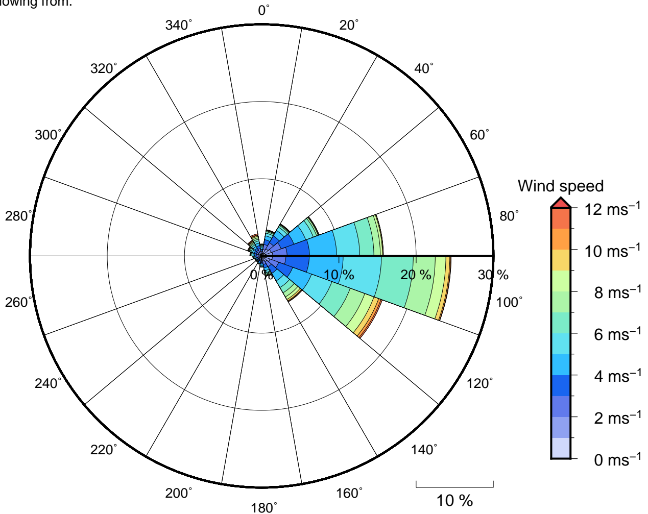
Figure 11 Annual wind rose for Safata Bay. Note that directions are where the wind is coming from.
