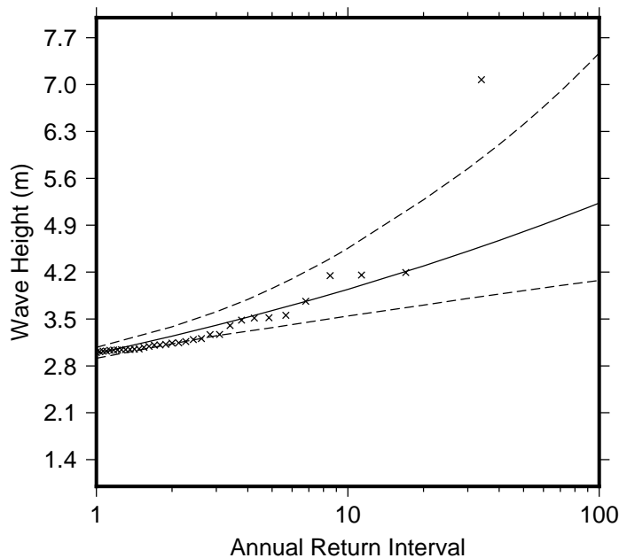
Figure 9 Extreme wave distribution for Nu'usafe'e Bay. The crosses represents the wave events that occurred since 1979. The plain line is the statistical distribution that best fit the past wave events. The dotted line show the upper and lower high confidence of the fit, there is a 95% chance that the fitted distribution lie between the two dashed lines.
