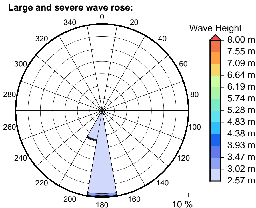
Figure 6 Large, severe and extreme wave roses for Nu'usafe'e Bay
