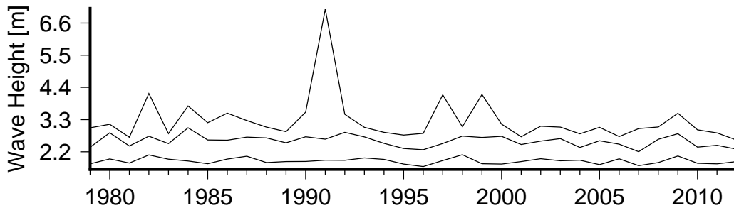
Figure 8 Annual variation in large waves (90th percentile)(lower curve), severe waves (99th percentile) (middle curve) and the largest wave(upper curve) in Nu'usafe'e Bay.
