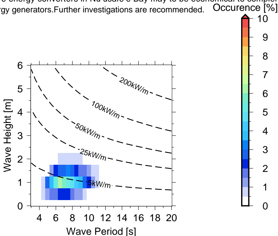
Figure 10 Occurences of sea states in Nu'usafe'e Bay .
