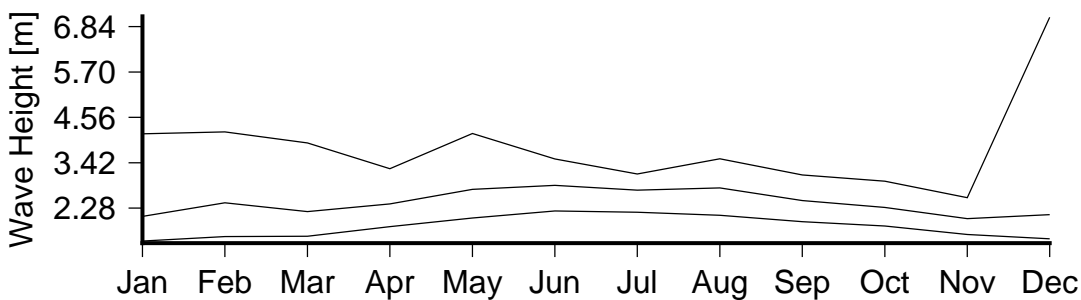
Figure 7 Monthly variation in large waves (90th percentile)(lower curve), severe waves (99th percentile) (middle curve) and the largest wave(upper curve) in Nu'usafe'e Bay.
