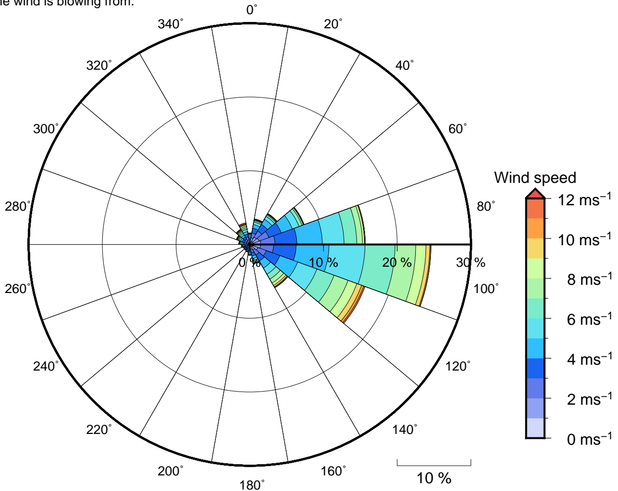
Figure 11 Annual wind rose for Nu'usafe'e Bay. Note that directions are where the wind is coming from.
