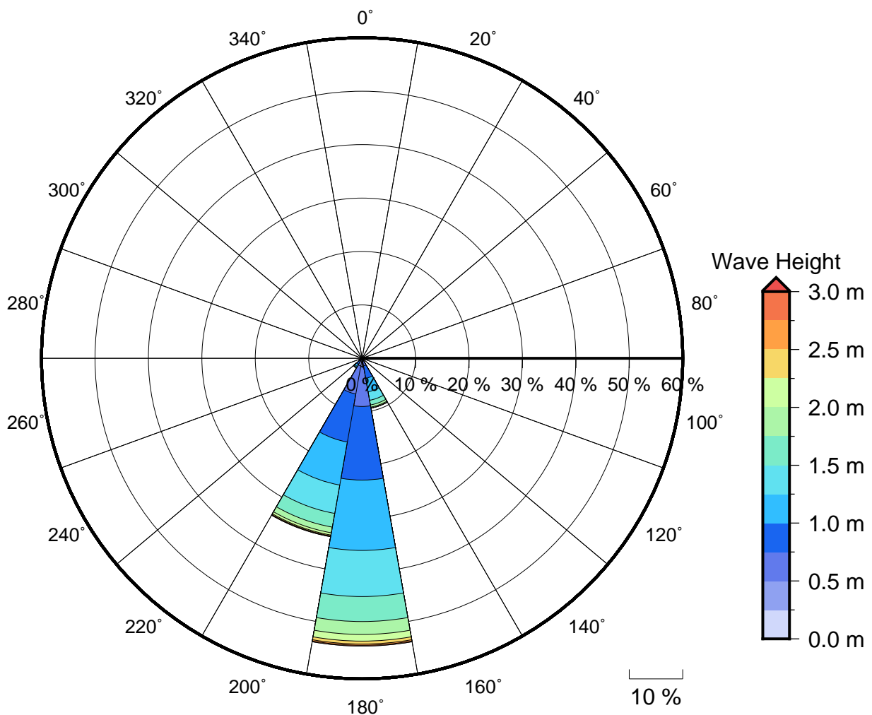
Figure 2 Annual wave rose for Nu'usafe'e Bay. Note that direction are where the wave are coming from .
