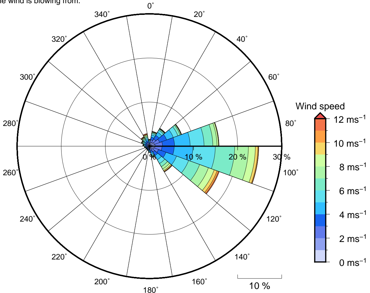
Figure 11 Annual wind rose for Mulifanua Warf. Note that directions are where the wind is coming from.
