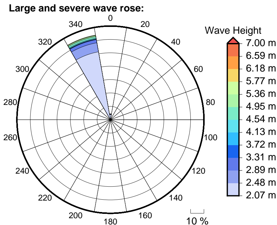
Figure 6 Large, severe and extreme wave roses for Mulifanua Warf
