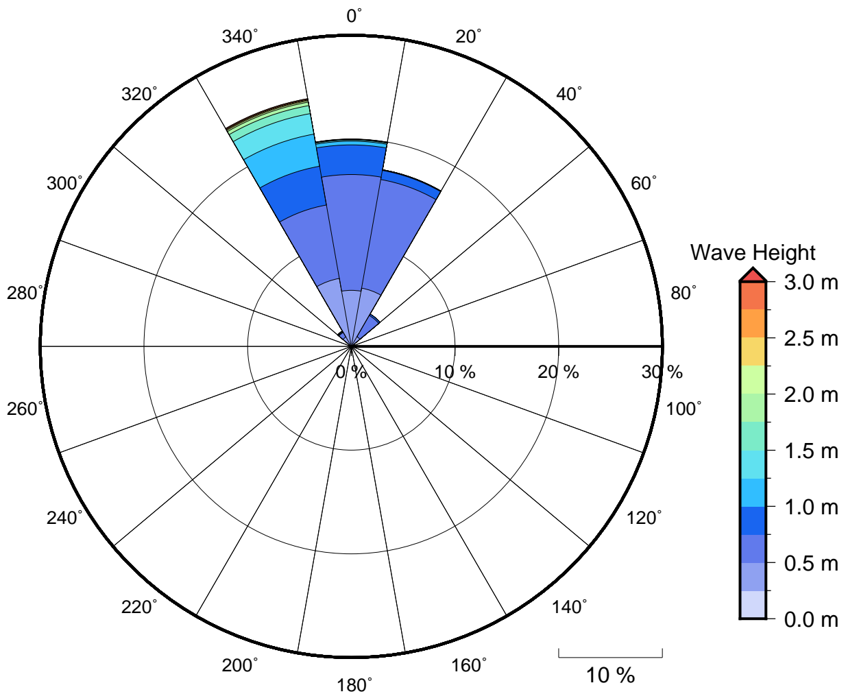
Figure 2 Annual wave rose for Mulifanua Warf. Note that direction are where the wave are coming from .
