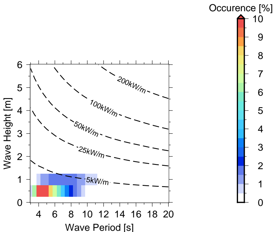
Figure 10 Occurrences of sea states in Mulifanua Warf .
