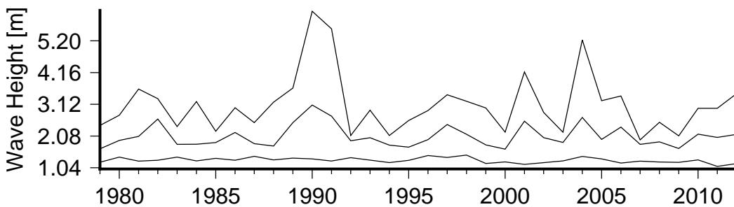
Figure 8 Annual variation in large waves (90th percentile)(lower curve), severe waves (99th percentile) (middle curve) and the largest wave(upper curve) in Mulifanua Warf.
