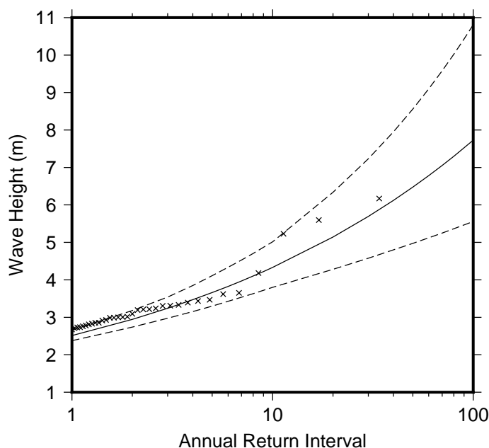
Figure 9 Extreme wave distribution for Mulifanua Warf. The crosses represents the wave events that occurred since 1979. The plain line is the statistical distribution that best fit the past wave events. The dotted line show the upper and lower high confidence of the fit, there is a 95% chance that the fitted distribution lie between the two dashed lines.
