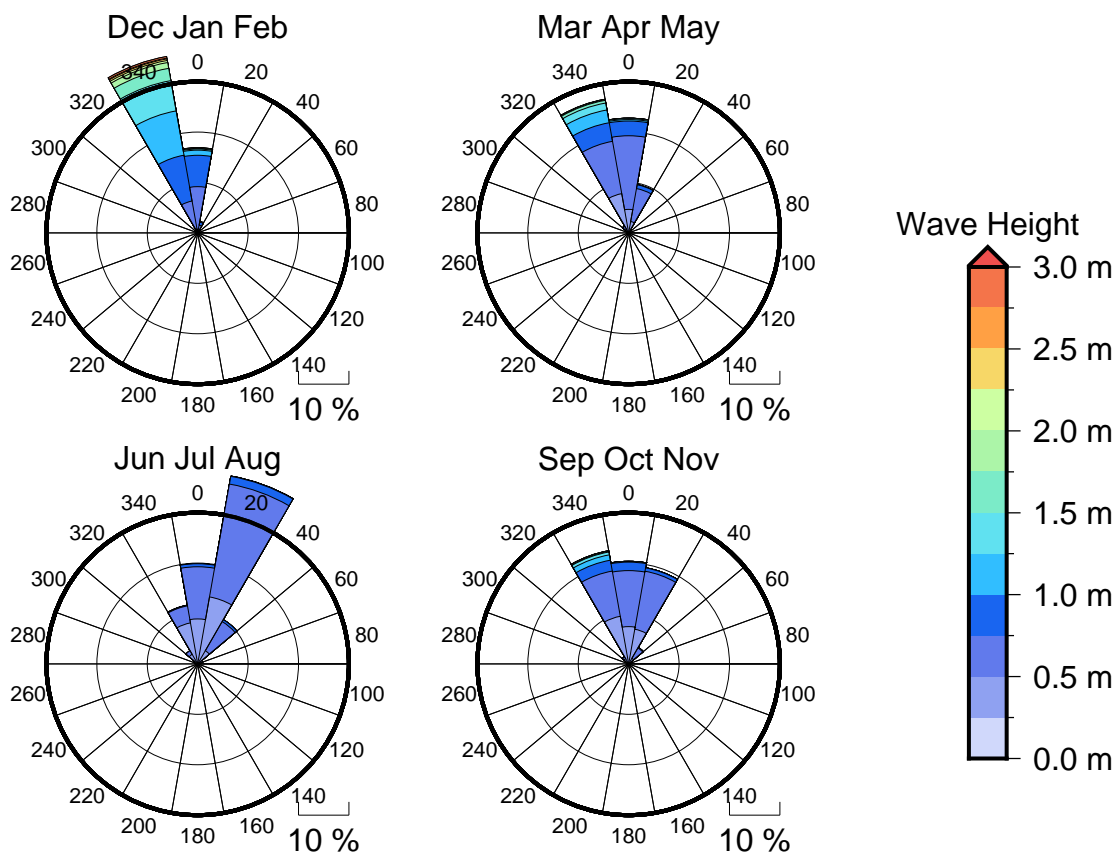
Figure 3 Seasonal wave roses for Mulifanua Warf
