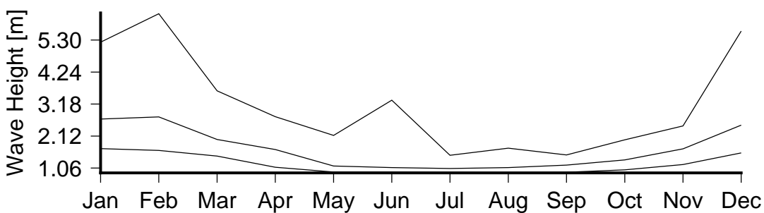
Figure 7 Monthly variation in large waves (90th percentile)(lower curve), severe waves (99th percentile) (middle curve) and the largest wave(upper curve) in Mulifanua Warf.
