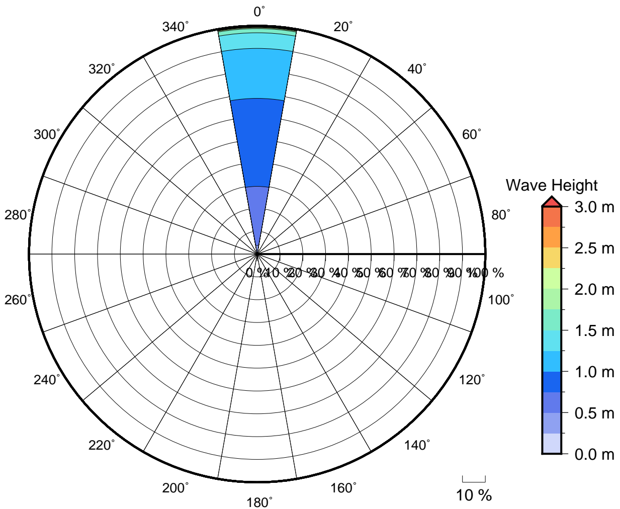
Figure 2 Annual wave rose for Faga. Note that direction are where the wave are coming from.
