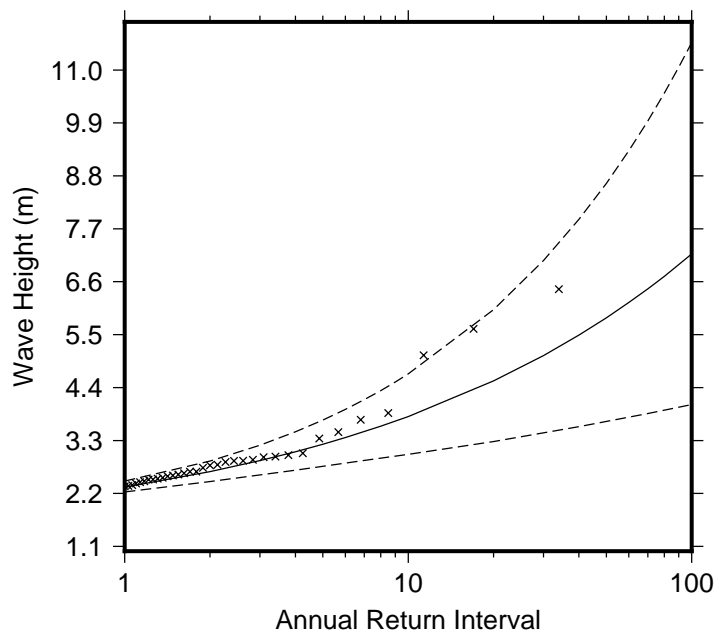
Figure 9 Extreme wave distribution for Faga. The crosses represents the wave events that occurred since 1979. The plain line is the statistical distribution that best fit the past wave events. The dotted line show the upper and lower high confidence of the fit, there is a 95% chance that the fitted distribution lie between the two dashed lines.
