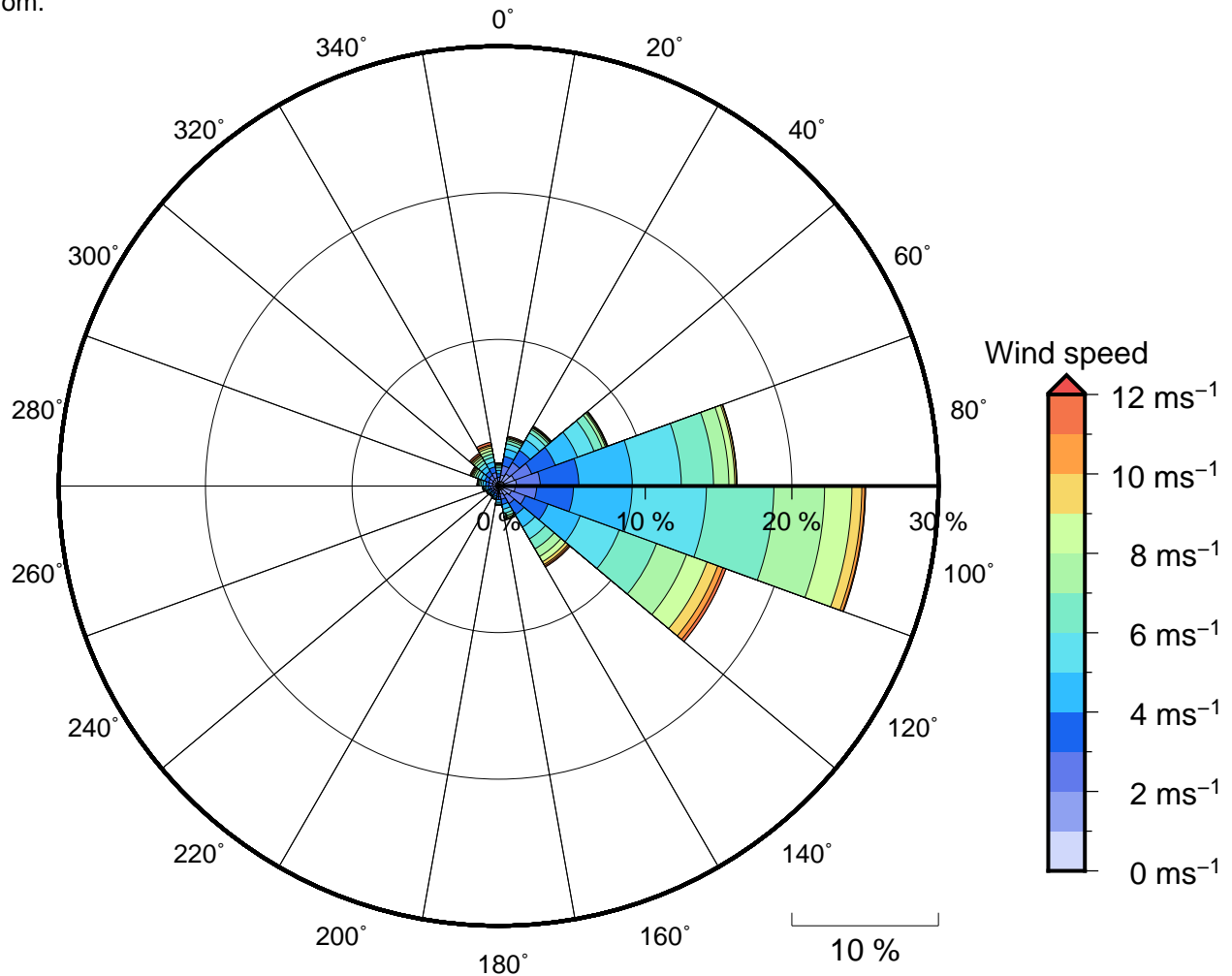
Figure 11 Annual wind rose for Faga. Note that directions are where the wind is coming from.
