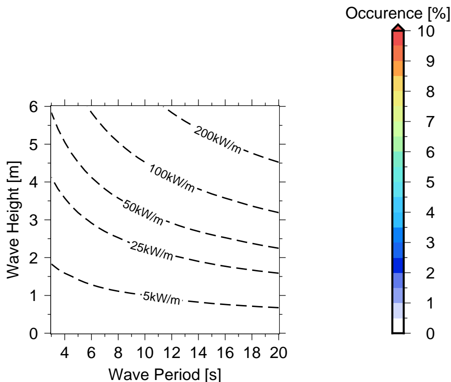
Figure 10 Occurrences of sea states in Faga .
