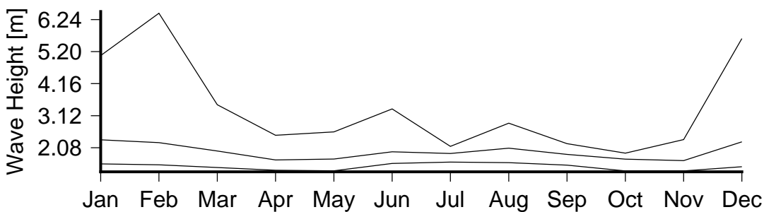
Figure 7 Monthly variation in large waves (90th percentile)(lower curve), severe waves (99th percentile) (middle curve) and the largest wave(upper curve) in Faga.
