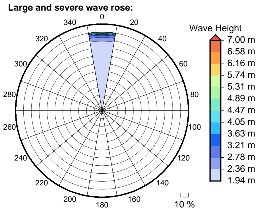
Figure 6 Large, severe and extreme wave roses for Faga
