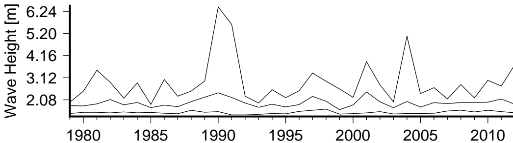
Figure 8 Annual variation in large waves (90th percentile)(lower curve), severe waves (99th percentile) (middle curve) and the largest wave(upper curve) in Faga.
