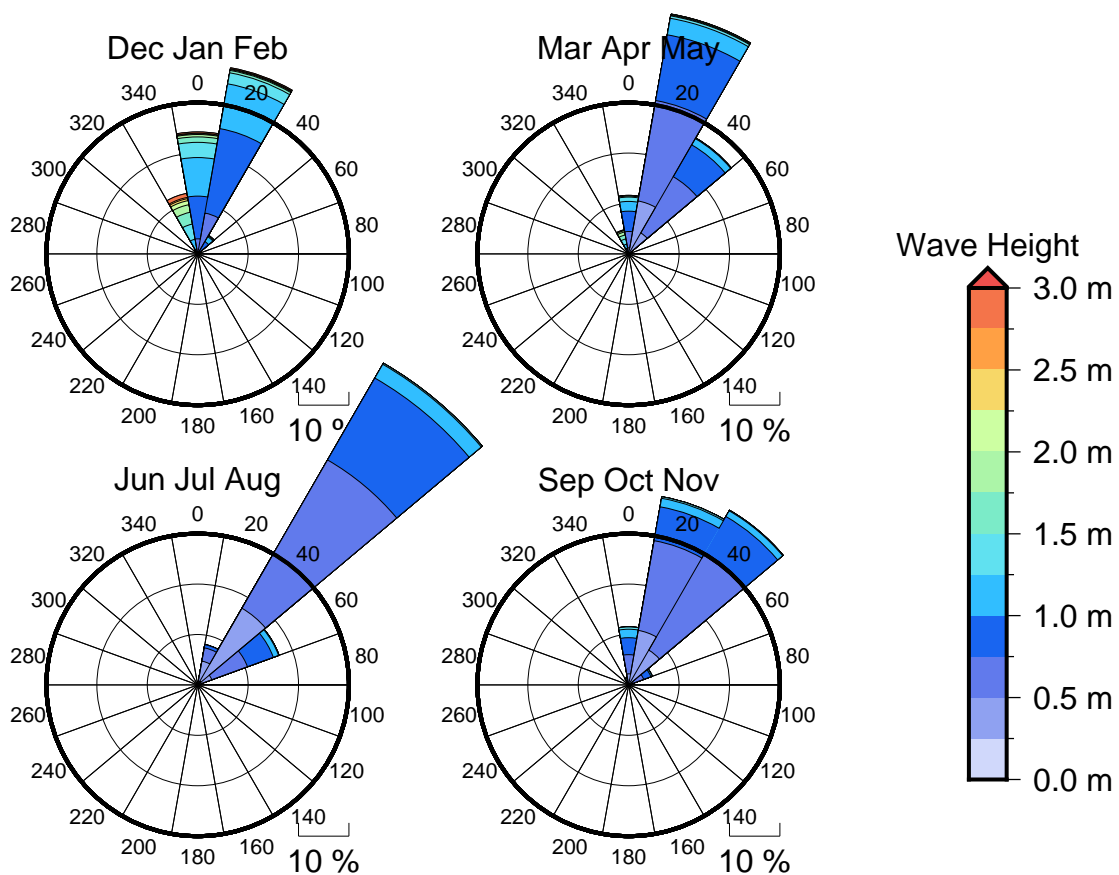
Figure 3 Seasonal wave roses for Asau Harbour Entrance
