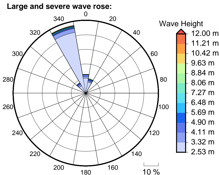
Figure 6 Large, severe and extreme wave roses for Asau Harbour Entrance
