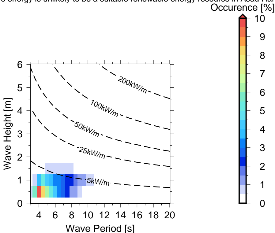
Figure 10 Occurrences of sea states in Asau Harbour Entrance .
