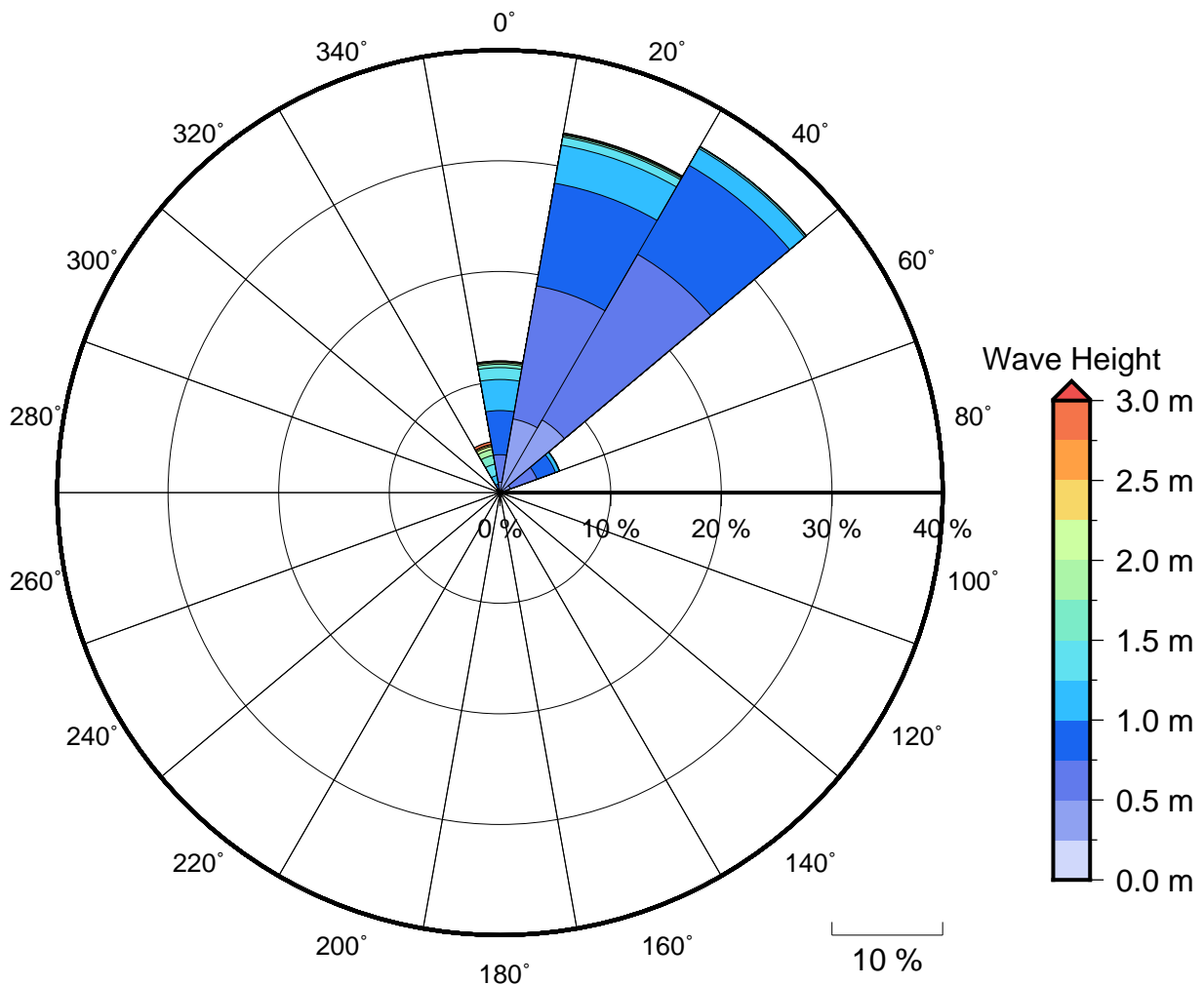
Figure 2 Annual wave rose for Asau Harbour Entrance. Note that direction are where the wave are coming from.
