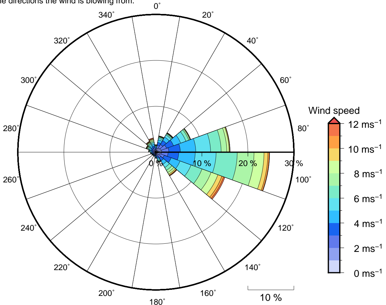
Figure 11 Annual wind rose for Asau Harbour Entrance. Note that directions are where the wind is coming from.
