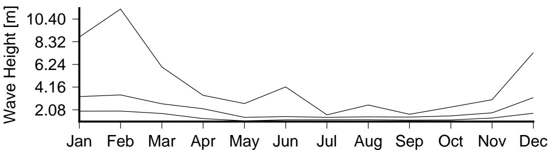
Figure 7 Monthly variation in large waves (90th percentile)(lower curve), severe waves (99th percentile) (middle curve) and the largest wave(upper curve) in Asau Harbour Entrance.
