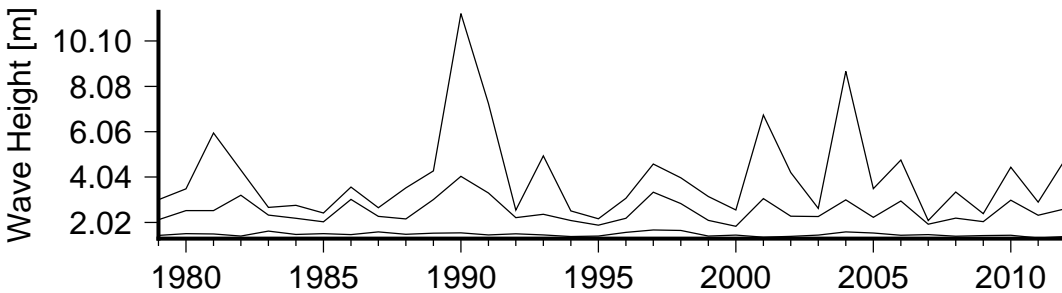
Figure 8 Annual variation in large waves (90th percentile)(lower curve), severe waves (99th percentile) (middle curve) and the largest wave(upper curve) in Asau Harbour Entrance.
