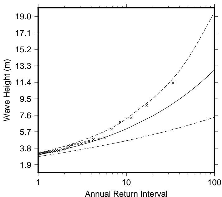
Figure 9 Extreme wave distribution for Asau Harbour Entrance. The crosses represents the wave events that occurred since 1979. The plain line is the statistical distribution that best fit the past wave events. The dotted line show the upper and lower high confidence of the fit, there is a 95% chance that the fitted distribution lie between the two dashed lines.
