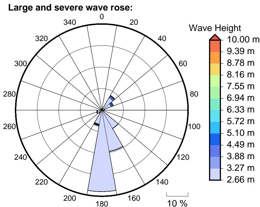
Figure 6 Large, severe and extreme wave roses for Apolima Strait
