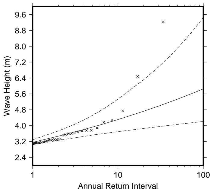
Figure 9 Extreme wave distribution for Apolima Strait. The crosses represents the wave events that occurred since 1979. The plain line is the statistical distribution that best fit the past wave events. The dotted line show the upper and lower high confidence of the fit, there is a 95% chance that the fitted distribution lie between the two dashed lines.
