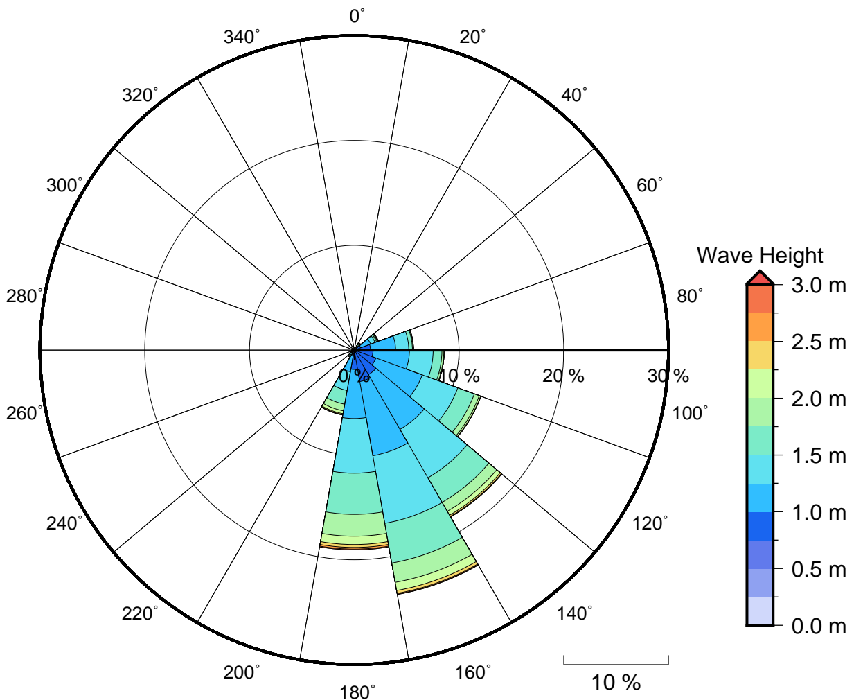
Figure 2 Annual wave rose for Apolima Strait. Note that direction are where the wave are coming from .
