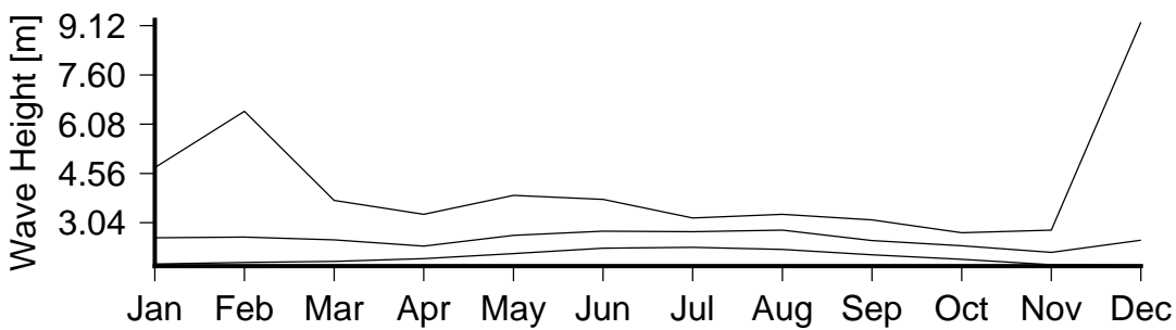
Figure 7 Monthly variation in large waves (90th percentile)(lower curve), severe waves (99th percentile) (middle curve) and the largest wave(upper curve) in Apolima Strait.
