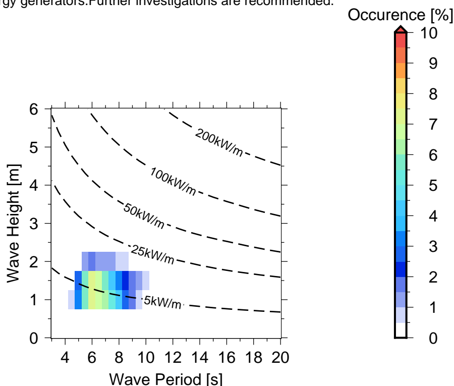
Figure 10 Occurrences of sea states in Apolima Strait .
