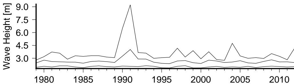
Figure 8 Annual variation in large waves (90th percentile)(lower curve), severe waves (99th percentile) (middle curve) and the largest wave(upper curve) in Apolima Strait.
