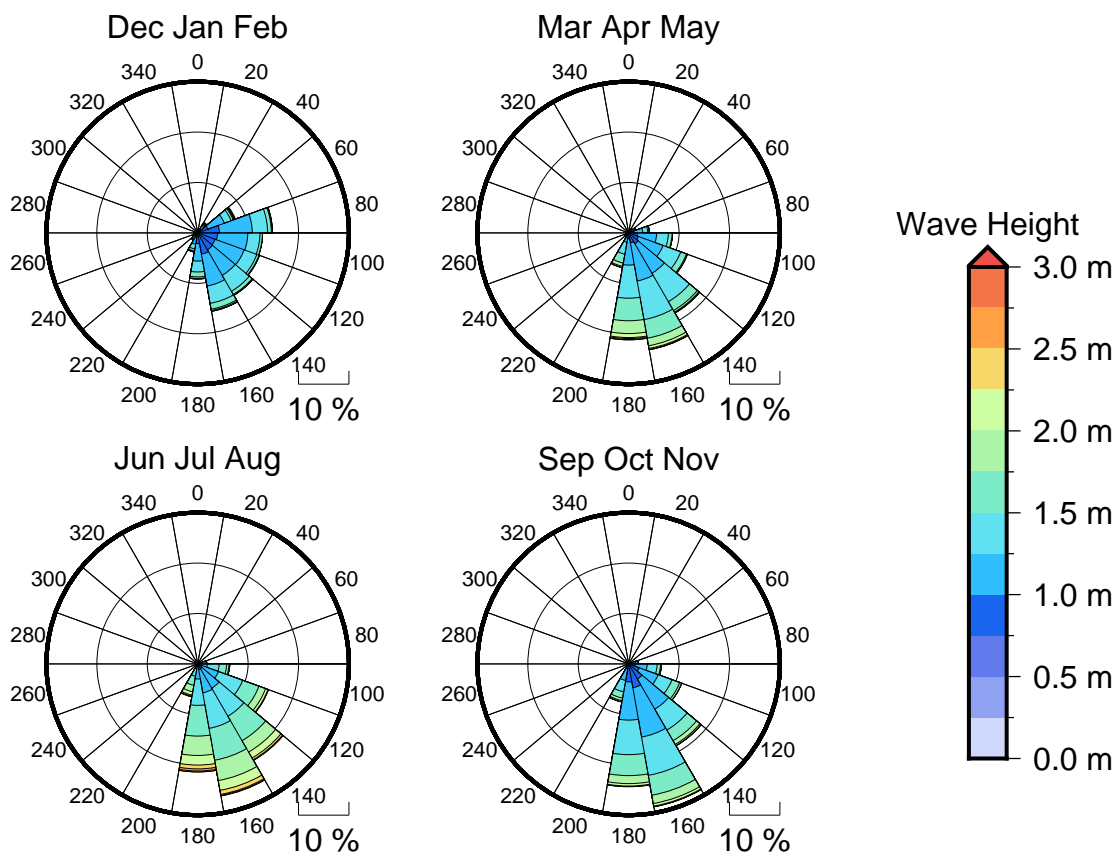
Figure 3 Seasonal wave roses for Apolima Strait
