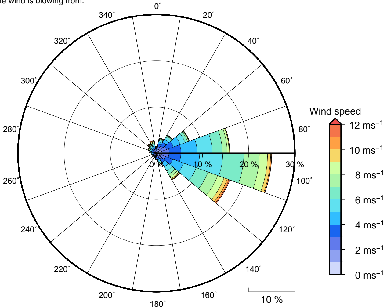
Figure 11 Annual wind rose for Apolima Strait. Note that directions are where the wind is coming from.
