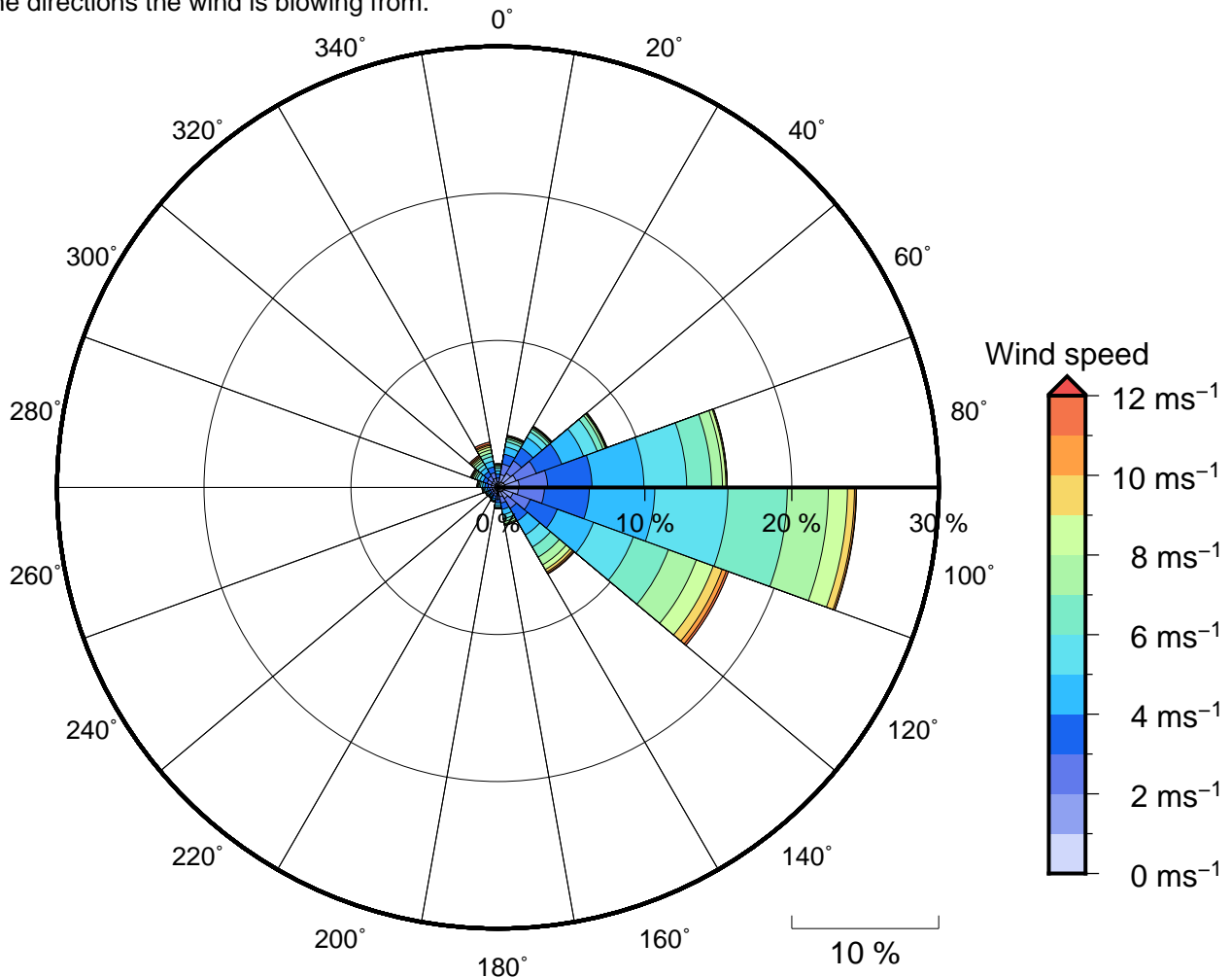
Figure 11 Annual wind rose for Apia Harbour Entrance. Note that directions are where the wind is coming from.
