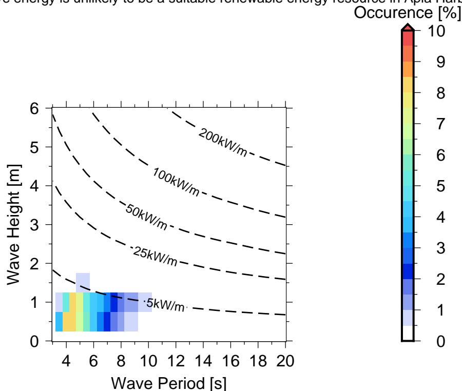
Figure 10 Occurrences of sea states in Apia Harbour Entrance .
