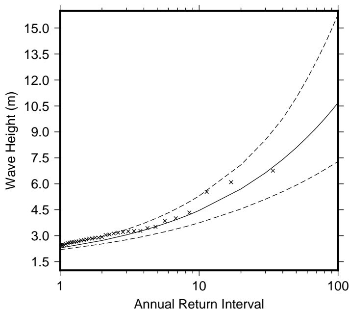
Figure 9 Extreme wave distribution for Apia Harbour Entrance. The crosses represents the wave events that occurred since 1979. The plain line is the statistical distribution that best fit the past wave events. The dotted line show the upper and lower high confidence of the fit, there is a 95% chance that the fitted distribution lie between the two dashed lines.
