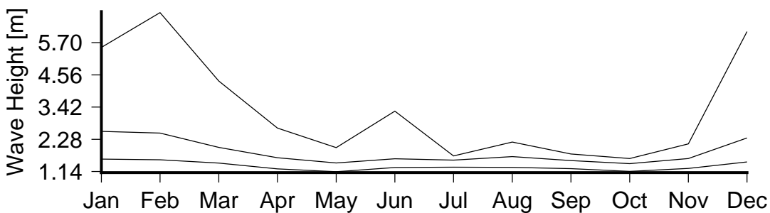
Figure 7 Monthly variation in large waves (90th percentile)(lower curve), severe waves (99th percentile) (middle curve) and the largest wave(upper curve) in Apia Harbour Entrance.
