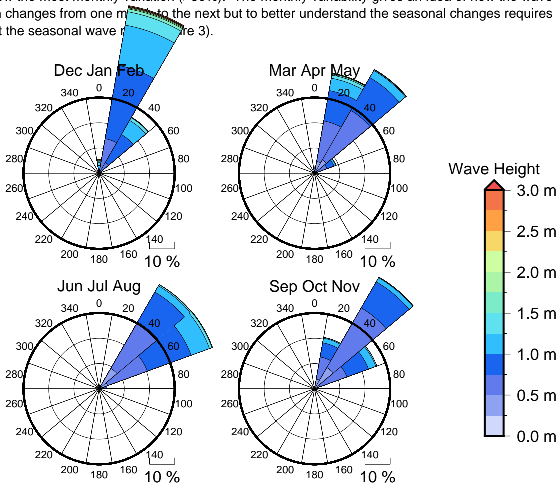
Figure 3 Seasonal wave roses for Apia Harbour Entrance
