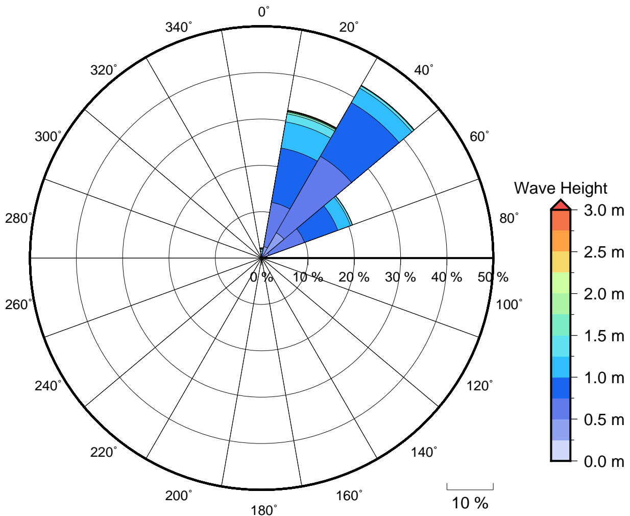
Figure 2 Annual wave rose for Apia Harbour Entrance. Note that direction are where the wave are coming from.
