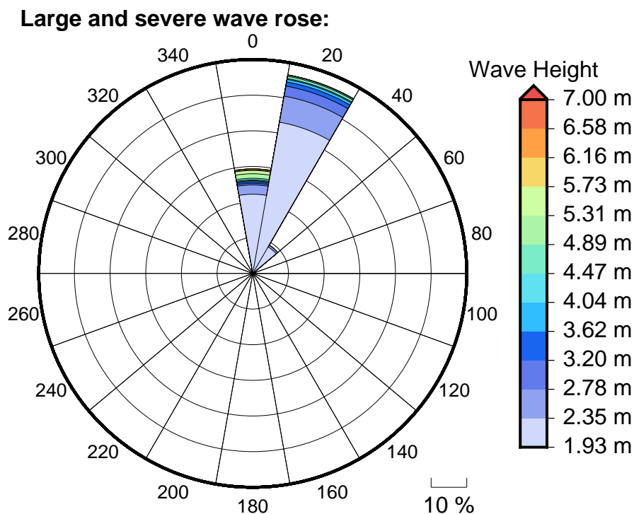
Figure 6 Large, severe and extreme wave roses for Apia Harbour Entrance
