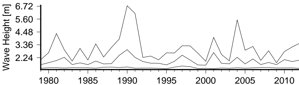
Figure 8 Annual variation in large waves (90th percentile)(lower curve), severe waves (99th percentile) (middle curve) and the largest wave(upper curve) in Apia Harbour Entrance.
