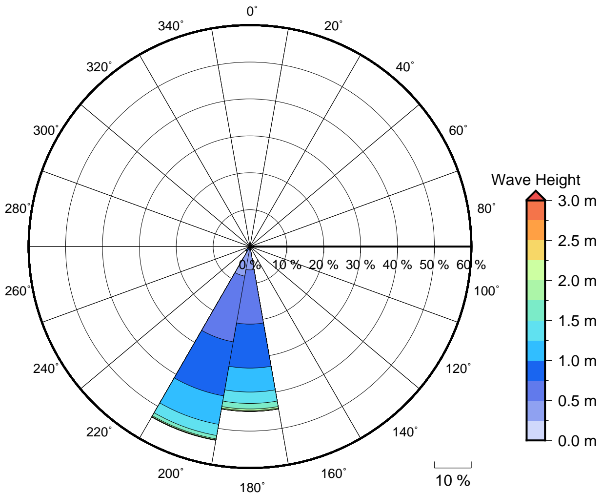
Figure 2 Annual wave rose for Aganoa. Note that direction are where the wave are coming from.
