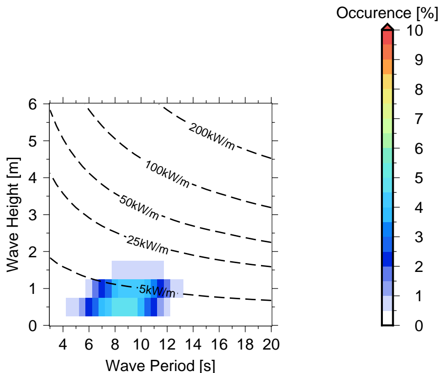
Figure 10 Occurrences of sea states in Aganoa .
