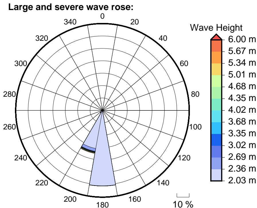
Figure 6 Large, severe and extreme wave roses for Aganoa
