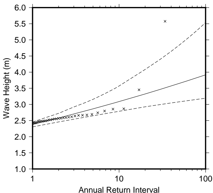
Figure 9 Extreme wave distribution for Aganoa. The crosses represents the wave events that occurred since 1979. The plain line is the statistical distribution that best fit the past wave events. The dotted line show the upper and lower high confidence of the fit, there is a 95% chance that the fitted distribution lie between the two dashed lines.
