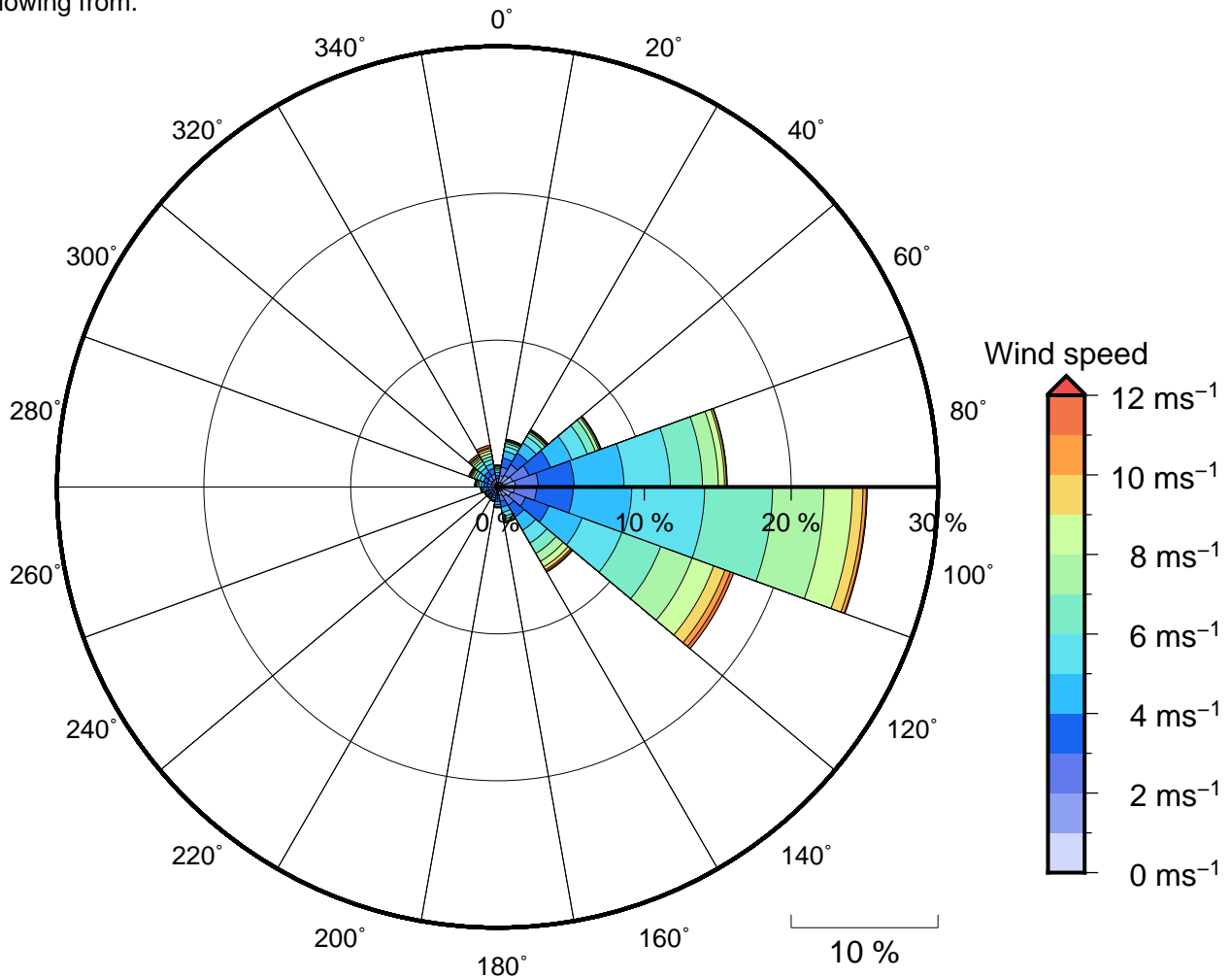
Figure 11 Annual wind rose for Aganoa. Note that directions are where the wind is coming from.
