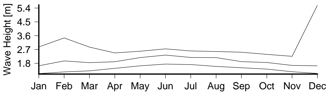
Figure 7 Monthly variation in large waves (90th percentile)(lower curve), severe waves (99th percentile) (middle curve) and the largest wave(upper curve) in Aganoa.
