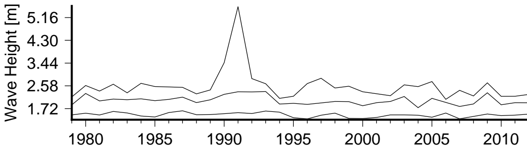
Figure 8 Annual variation in large waves (90th percentile)(lower curve), severe waves (99th percentile) (middle curve) and the largest wave(upper curve) in Aganoa.
