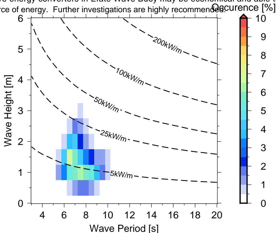
Figure 10 Occurrences of sea states in Efate Wave Buoy .
