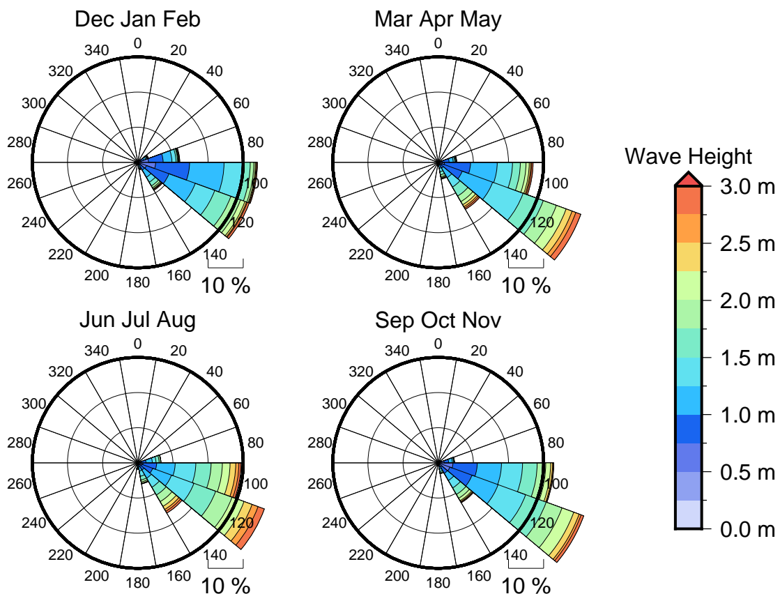
Figure 3 Seasonal wave roses for Efate Wave Buoy
