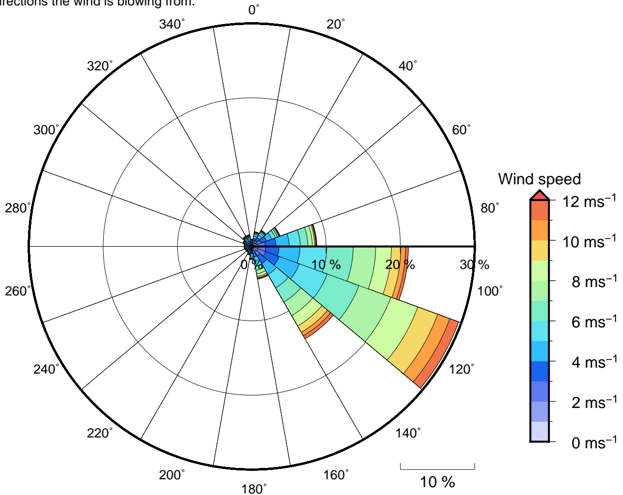
Figure 11 Annual wind rose for Efate Wave Buoy. Note that directions are where the wind is coming from.
