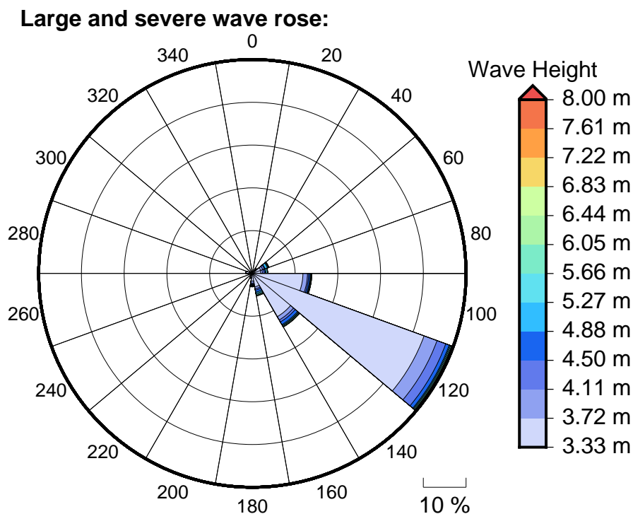
Figure 6 Large, severe and extreme wave roses for Efate Wave Buoy
