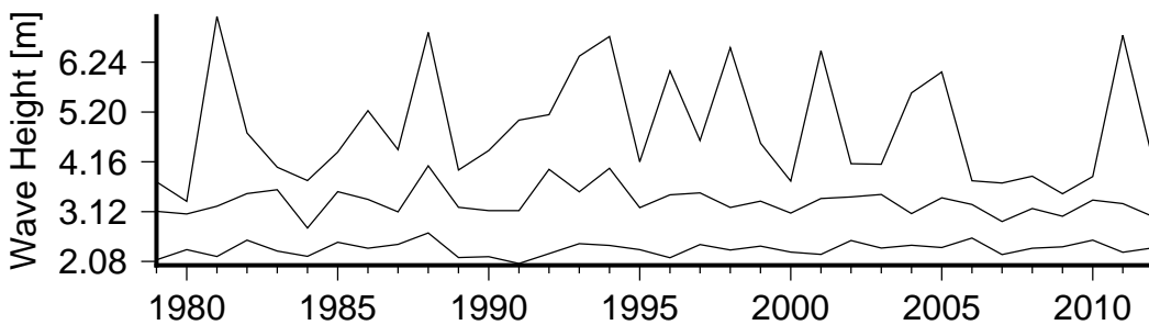
Figure 8 Annual variation in large waves (90th percentile)(lower curve), severe waves (99th percentile) (middle curve) and the largest wave(upper curve) in Efate Wave Buoy.
