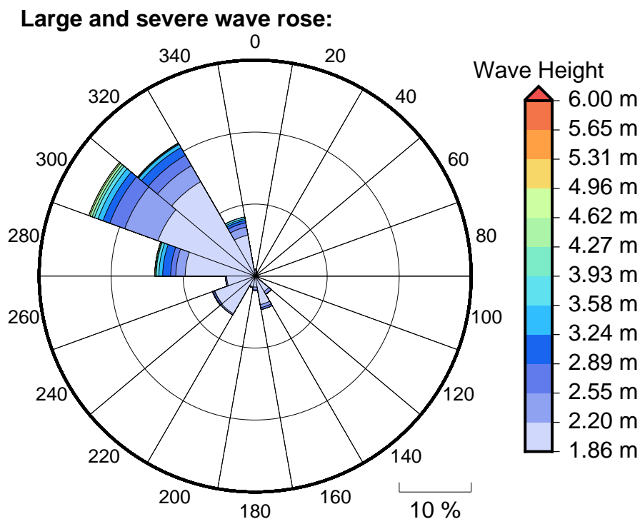
Figure 6 Large, severe and extreme wave roses for Neiafu
