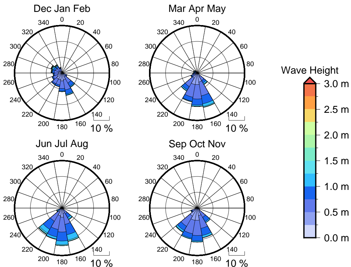
Figure 3 Seasonal wave roses for Neiafu
