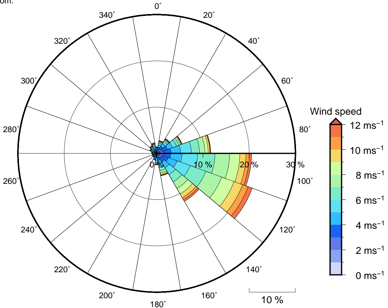
Figure 11 Annual wind rose for Neiafu. Note that directions are where the wind is coming from.
