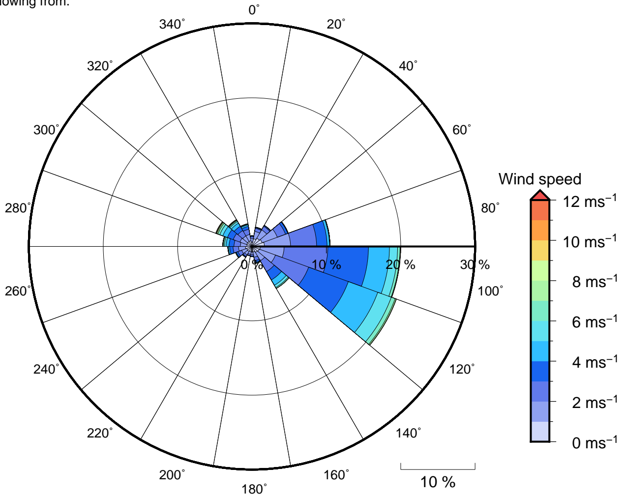
Figure 11 Annual wind rose for Isabel Is.. Note that directions are where the wind is coming from .
