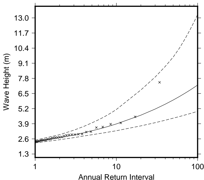
Figure 9 Extreme wave distribution for Isabel Is.. The crosses represents the wave events that occurred since 1979. The plain line is the statistical distribution that best fit the past wave events. The dotted line show the upper and lower high confidence of the fit, there is a 95% chance that the fitted distribution lie between the two dashed lines.
