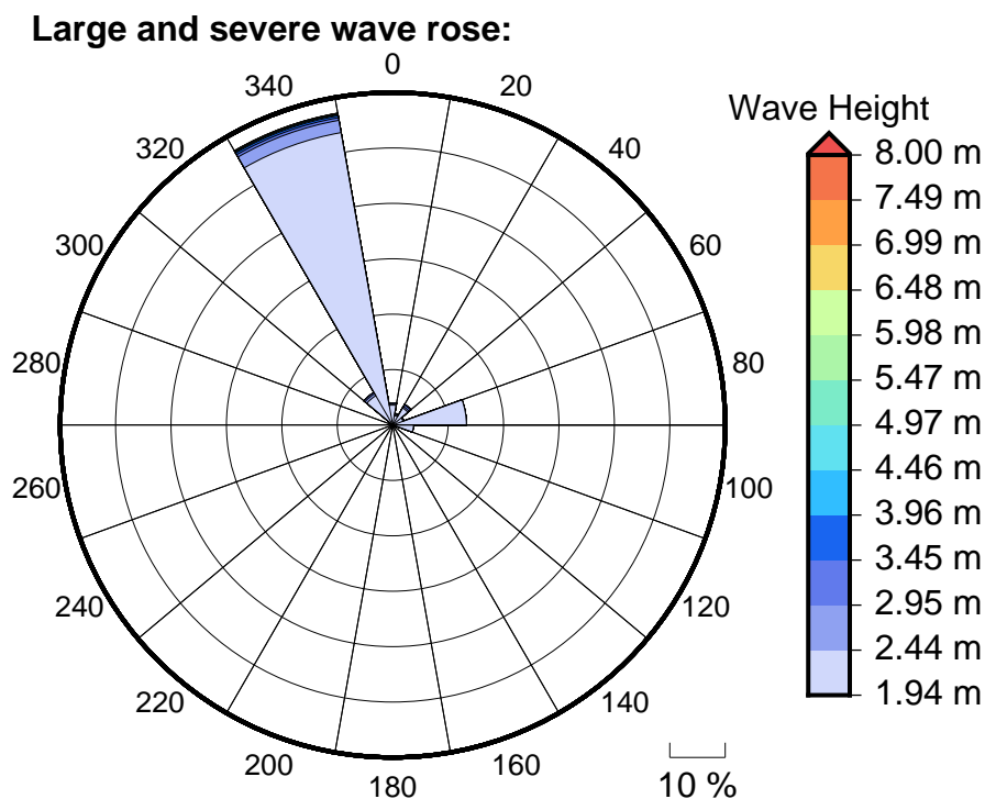
Figure 6 Large, severe and extreme wave roses for Isabel Is.
