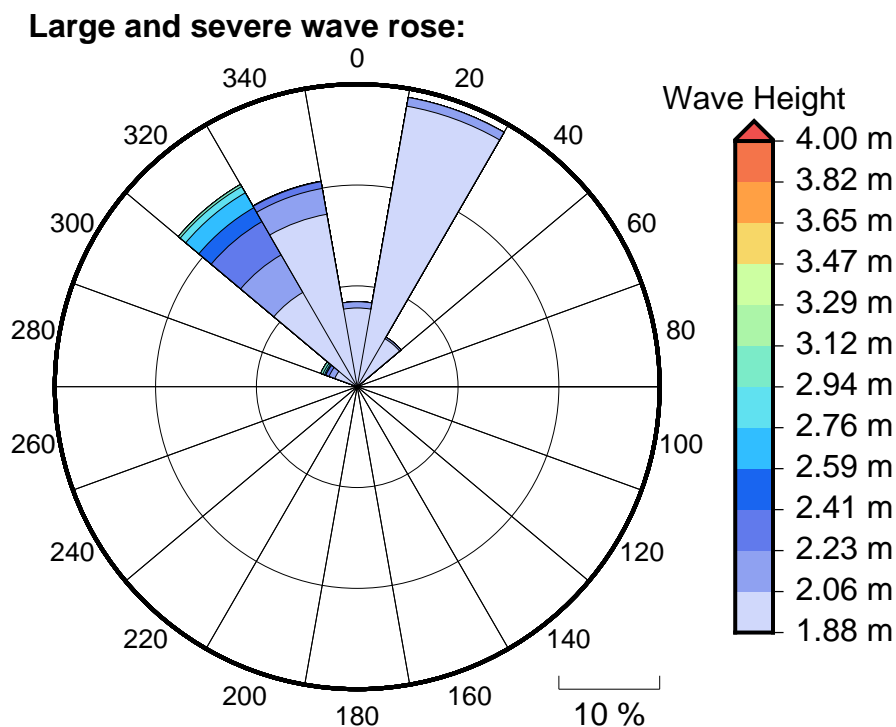
Figure 6 Large, severe and extreme wave roses for Lorengau
