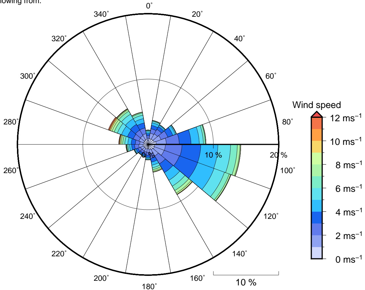
Figure 11 Annual wind rose for Lorengau. Note that directions are where the wind is coming from.
