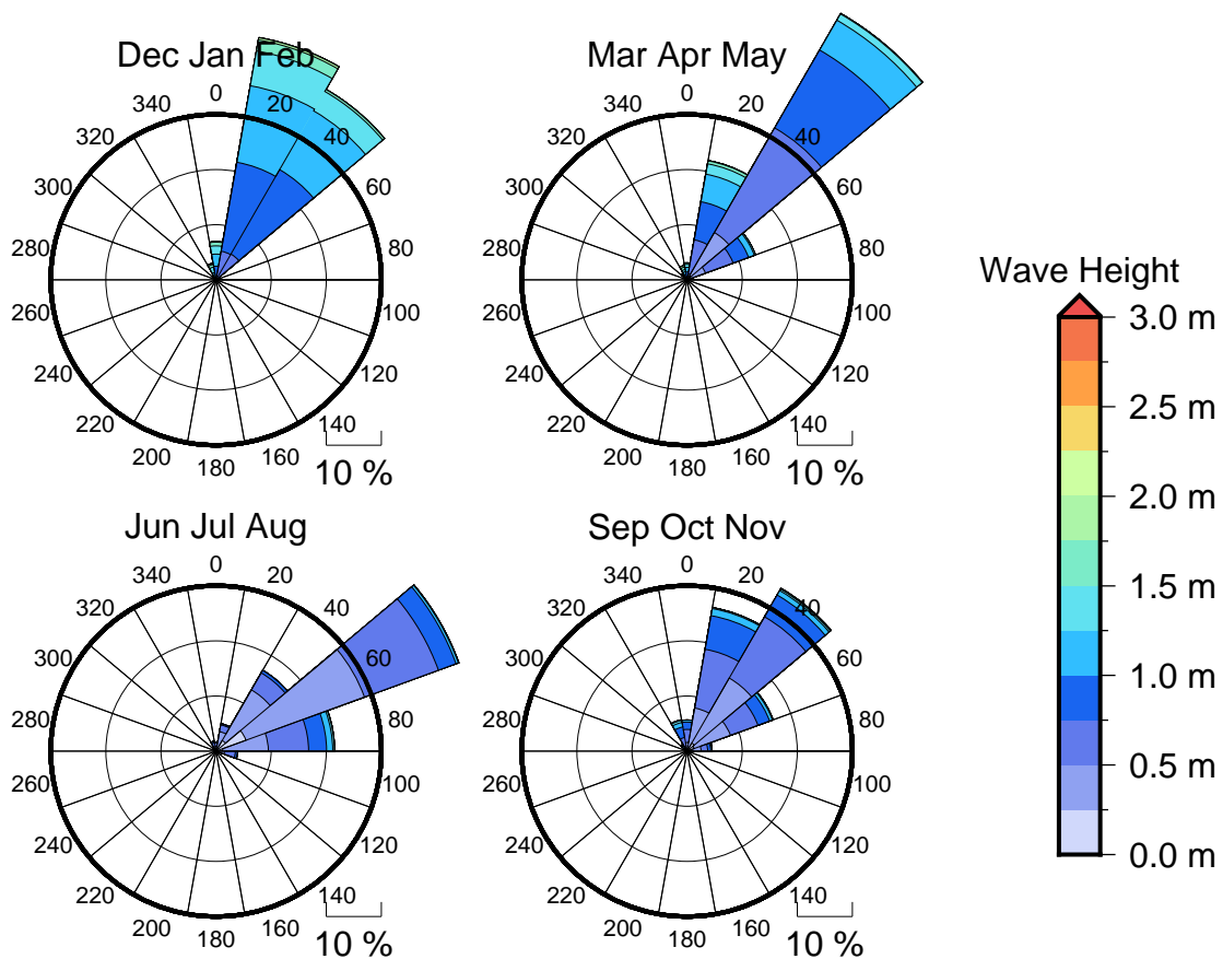
Figure 3 Seasonal wave roses for Lorengau
