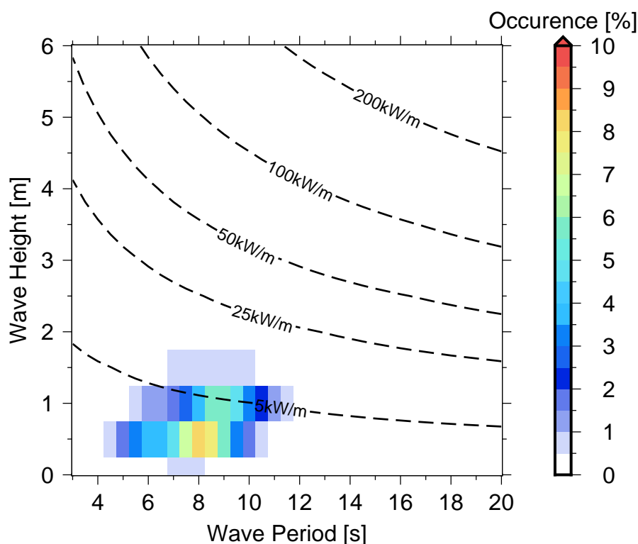
Figure 10 Occurrences of sea states in Lorengau .
