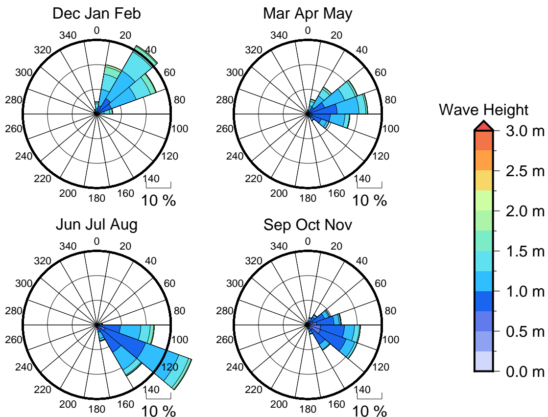
Figure 3 Seasonal wave roses for Nauru
