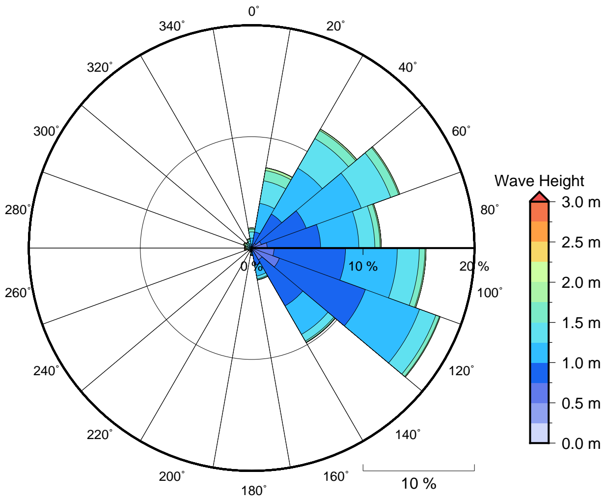
Figure 2 Annual wave rose for Nauru. Note that direction are where the wave are coming from.
