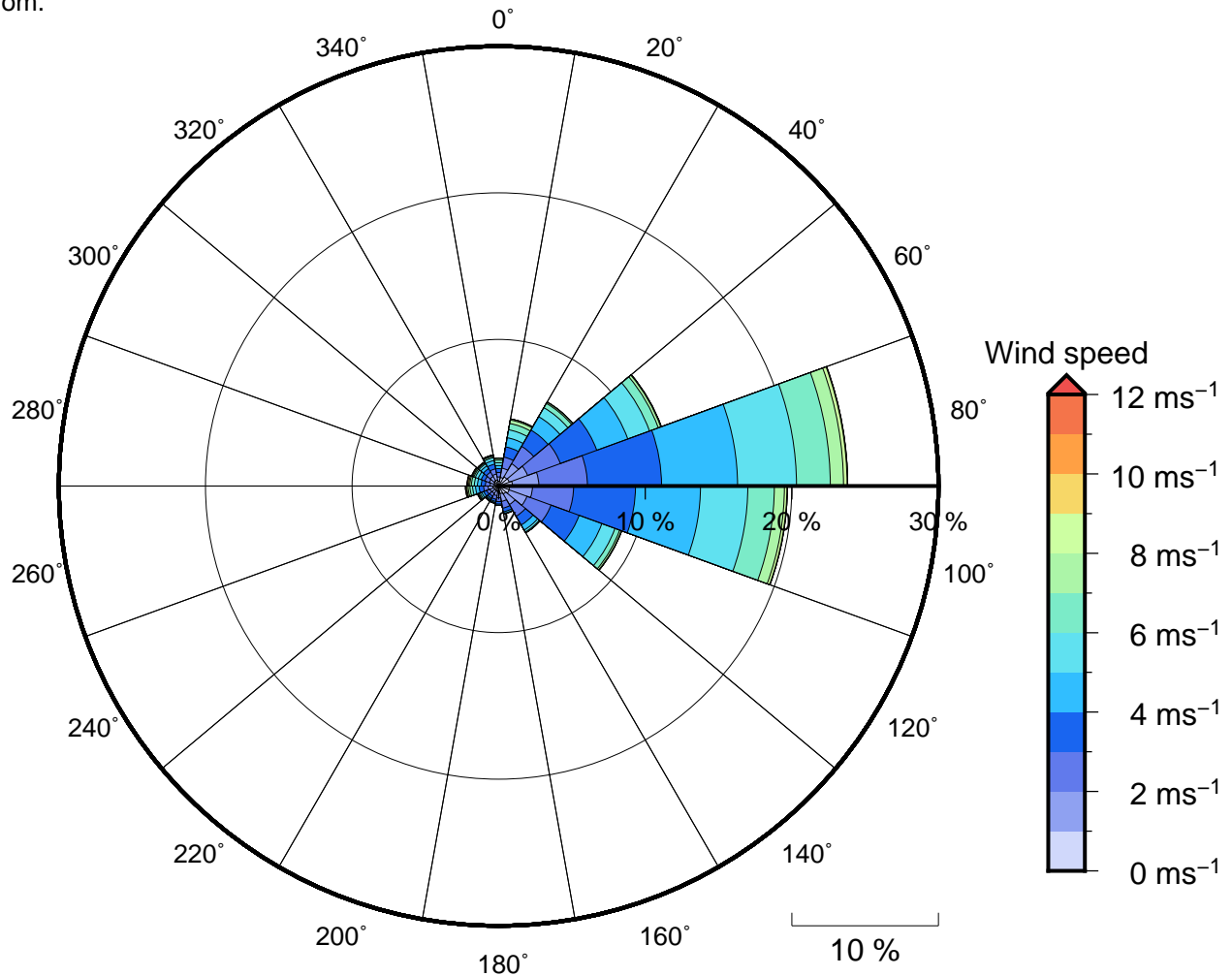
Figure 11 Annual wind rose for Nauru. Note that directions are where the wind is coming from .
