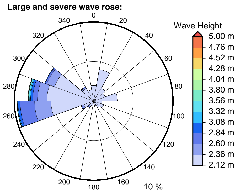
Figure 6 Large, severe and extreme wave roses for Nauru
