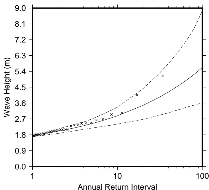
Figure 9 Extreme wave distribution for Yanuca Island. The crosses represents the wave events that occurred since 1979. The plain line is the statistical distribution that best fit the past wave events. The dotted line show the upper and lower high confidence of the fit, there is a 95% chance that the fitted distribution lie between the two dashed lines.
