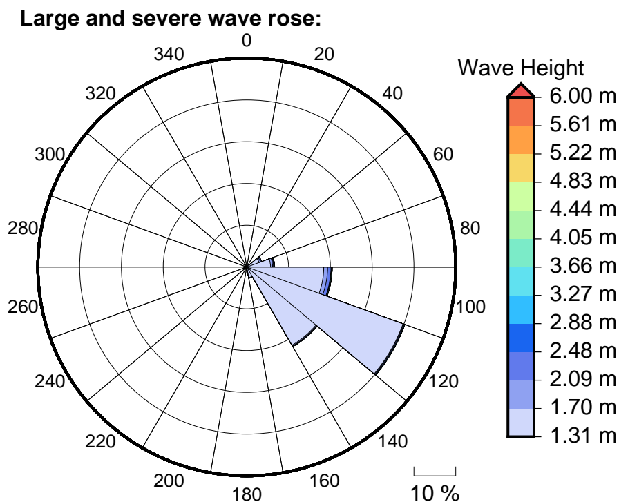
Figure 6 Large, severe and extreme wave roses for Yanuca Island
