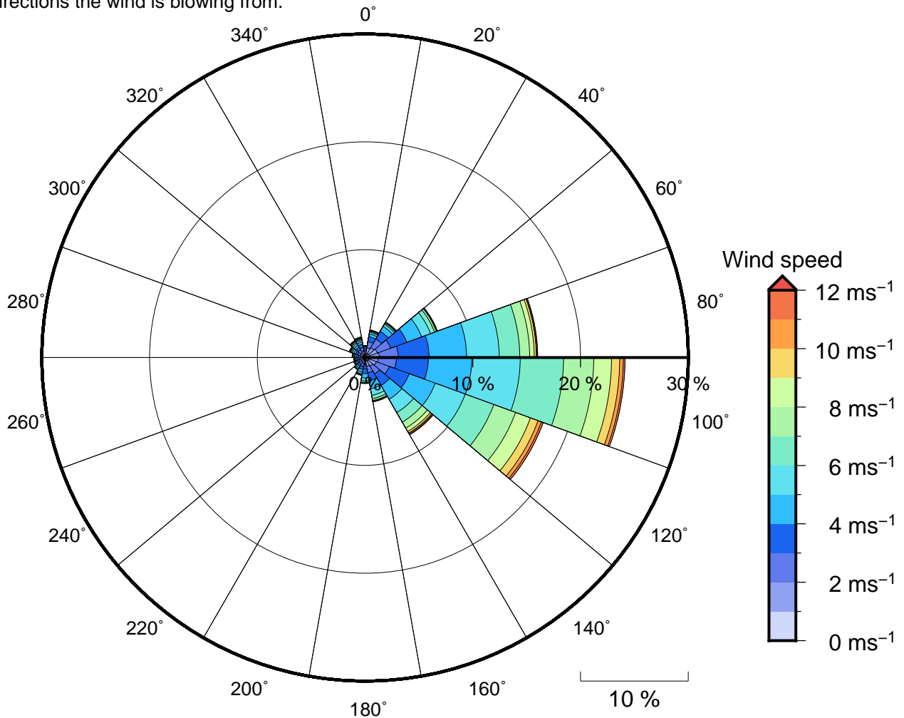
Figure 11 Annual wind rose for Yanuca Island. Note that directions are where the wind is coming from.
