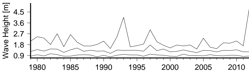
Figure 8 Annual variation in large waves (90th percentile)(lower curve), severe waves (99th percentile) (middle curve) and the largest wave(upper curve) in Yanuca Island.
