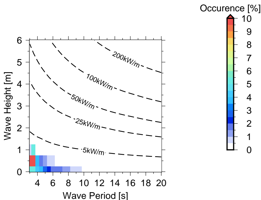
Figure 10 Occurrences of sea states in Yanuca Island .
