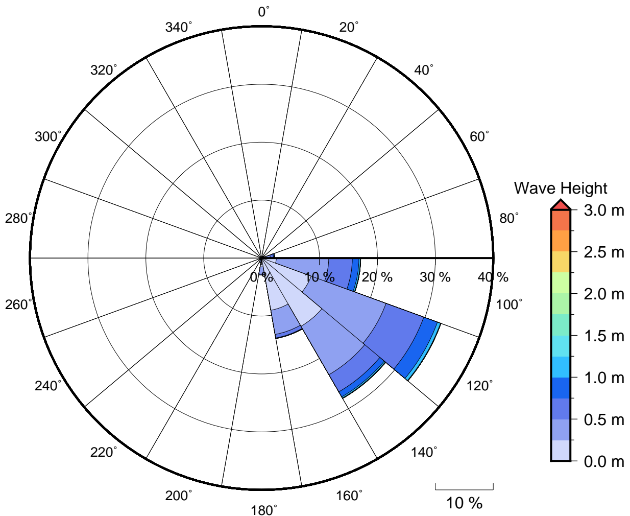
Figure 2 Annual wave rose for Yanuca Island. Note that direction are where the wave are coming from .
