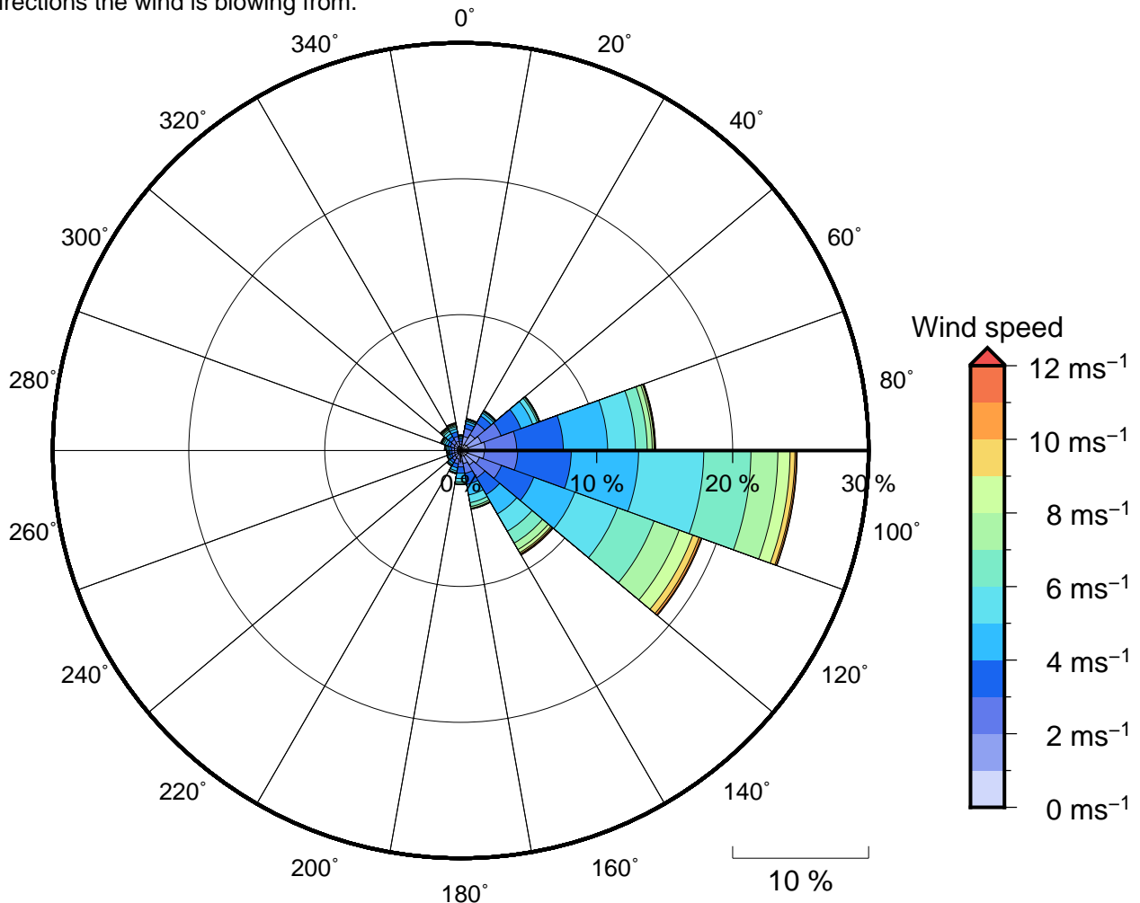
Figure 11 Annual wind rose for Wellesley Resort. Note that directions are where the wind is coming from.
