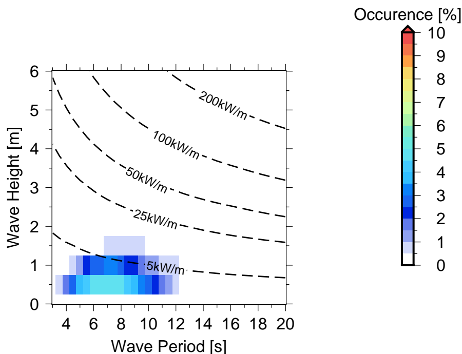
Figure 10 Occurrences of sea states in Wellesley Resort .
