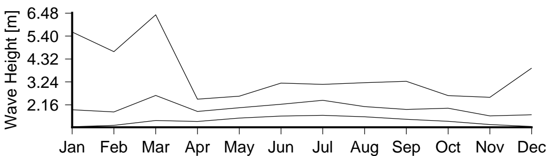
Figure 7 Monthly variation in large waves (90th percentile)(lower curve), severe waves (99th percentile) (middle curve) and the largest wave(upper curve) in Wellesley Resort.
