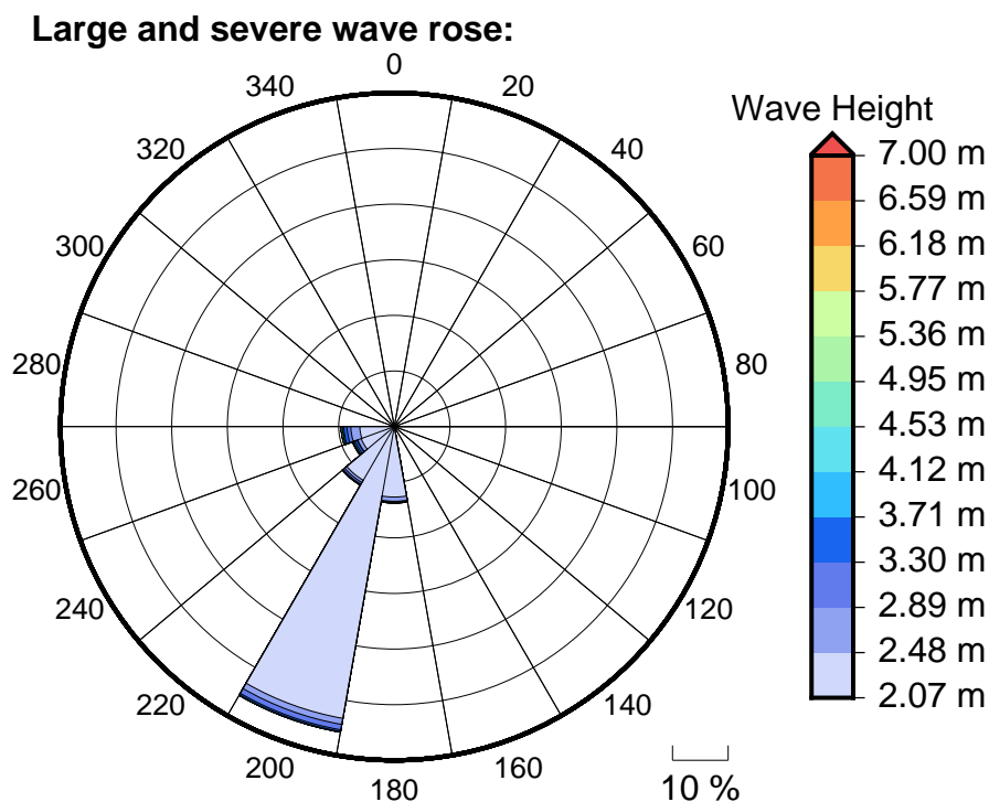
Figure 6 Large, severe and extreme wave roses for Wellesley Resort
