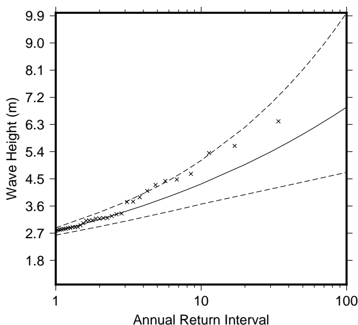
Figure 9 Extreme wave distribution for Wellesley Resort. The crosses represents the wave events that occurred since 1979. The plain line is the statistical distribution that best fit the past wave events. The dotted line show the upper and lower high confidence of the fit, there is a 95% chance that the fitted distribution lie between the two dashed lines.
