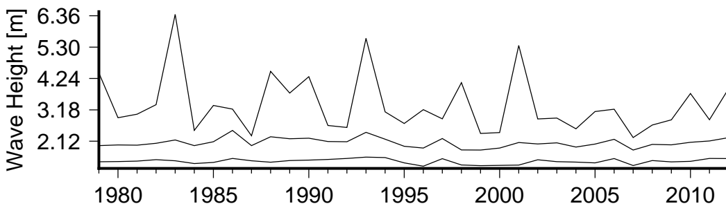
Figure 8 Annual variation in large waves (90th percentile)(lower curve), severe waves (99th percentile) (middle curve) and the largest wave(upper curve) in Wellesley Resort.
