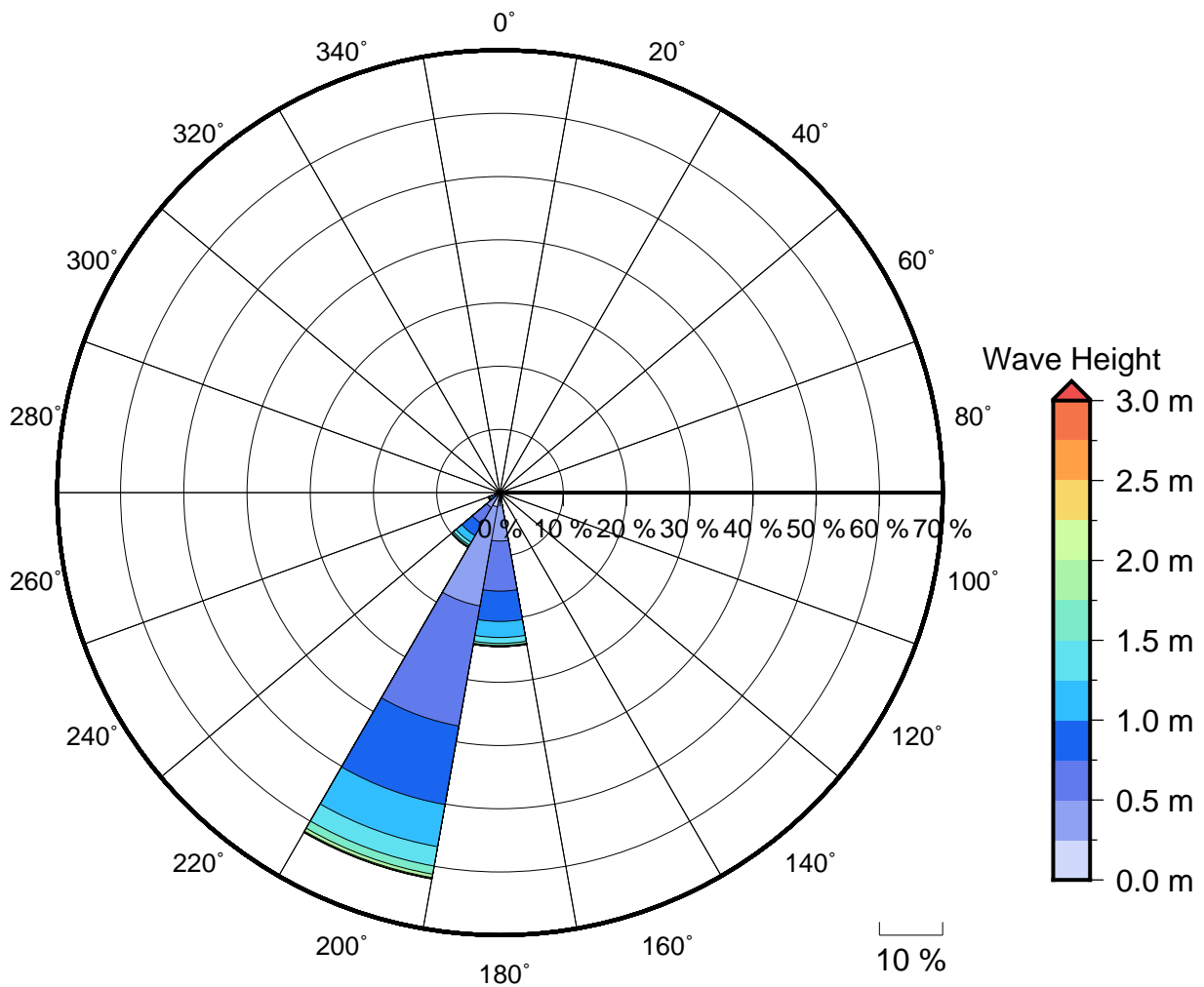
Figure 2 Annual wave rose for Wellesley Resort. Note that direction are where the wave are coming from .
