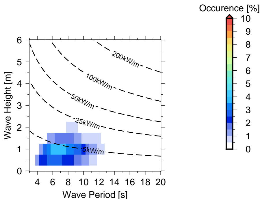
Figure 10 Occurrences of sea states in Warwick Hotel .
