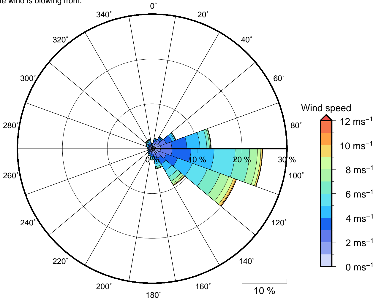
Figure 11 Annual wind rose for Warwick Hotel. Note that directions are where the wind is coming from.
