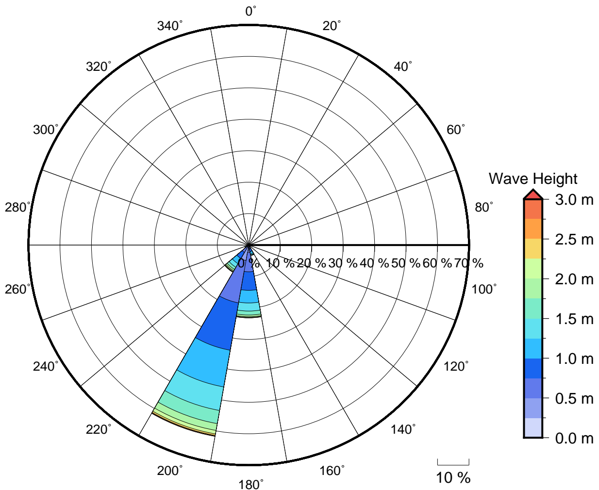
Figure 2 Annual wave rose for Warwick Hotel. Note that direction are where the wave are coming from .
