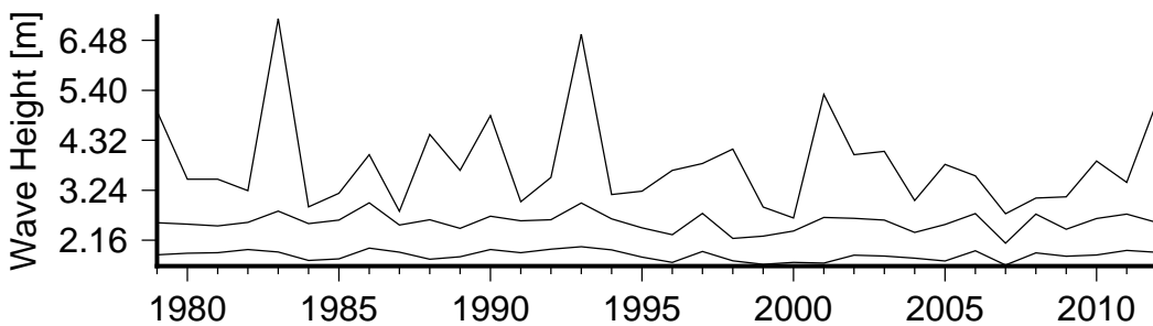
Figure 8 Annual variation in large waves (90th percentile)(lower curve), severe waves (99th percentile) (middle curve) and the largest wave(upper curve) in Warwick Hotel.
