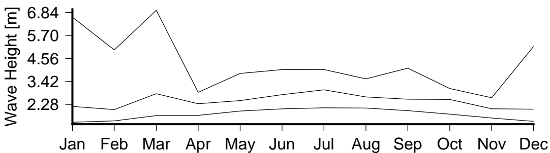
Figure 7 Monthly variation in large waves (90th percentile)(lower curve), severe waves (99th percentile) (middle curve) and the largest wave(upper curve) in Warwick Hotel.
