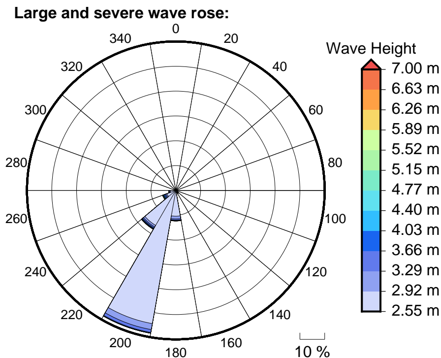
Figure 6 Large, severe and extreme wave roses for Warwick Hotel
