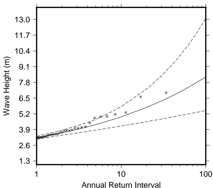
Figure 9 Extreme wave distribution for Warwick Hotel. The crosses represents the wave events that occurred since 1979. The plain line is the statistical distribution that best fit the past wave events. The dotted line show the upper and lower high confidence of the fit, there is a 95% chance that the fitted distribution lie between the two dashed lines.
