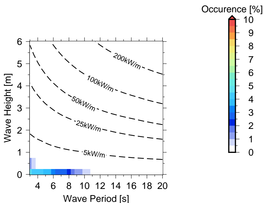
Figure 10 Occurrences of sea states in Vunisea .
