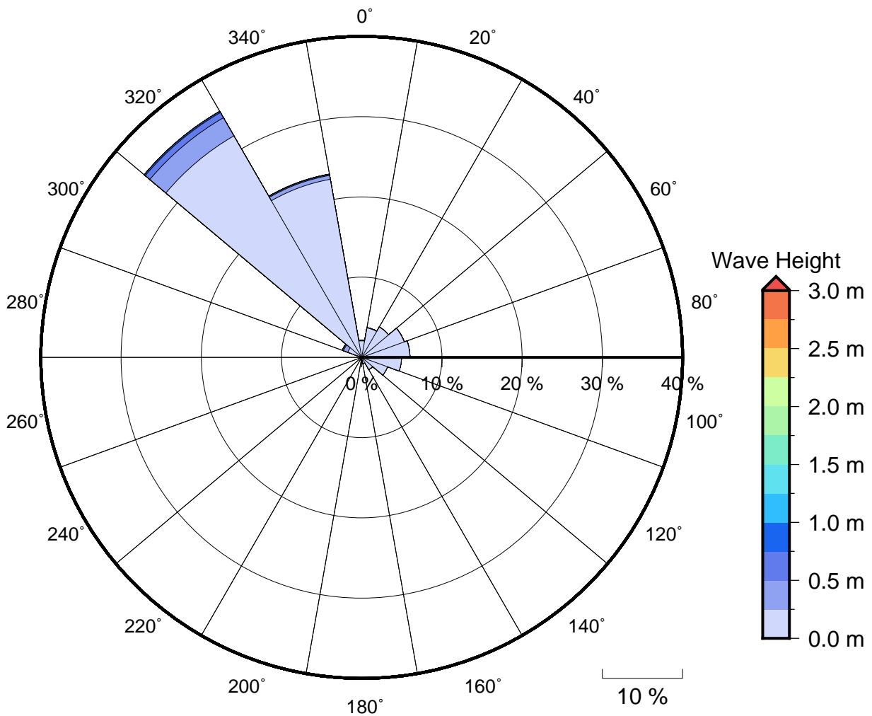
Figure 2 Annual wave rose for Vunisea. Note that direction are where the wave are coming from.
