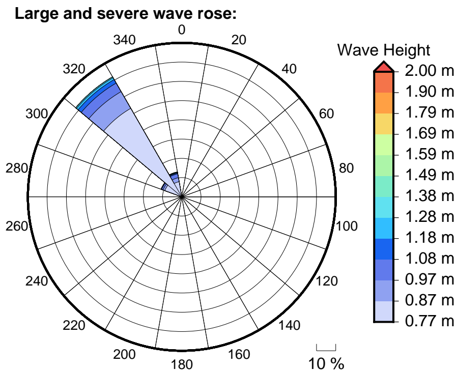
Figure 6 Large, severe and extreme wave roses for Vunisea
