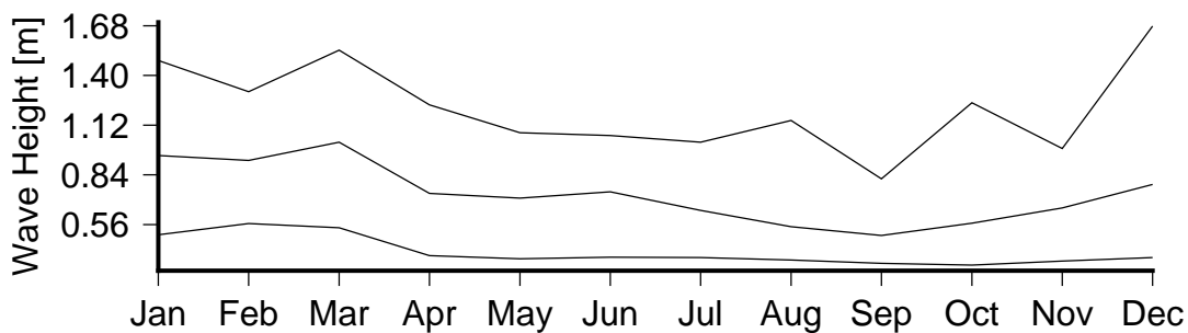
Figure 7 Monthly variation in large waves (90th percentile)(lower curve), severe waves (99th percentile) (middle curve) and the largest wave(upper curve) in Vunisea.
