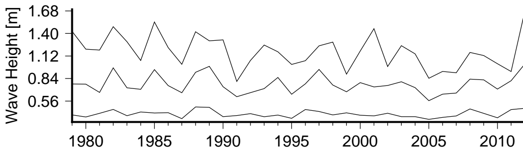
Figure 8 Annual variation in large waves (90th percentile)(lower curve), severe waves (99th percentile) (middle curve) and the largest wave(upper curve) in Vunisea.
