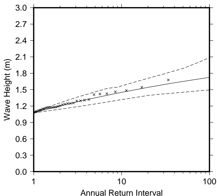
Figure 9 Extreme wave distribution for Vunisea. The crosses represents the wave events that occurred since 1979. The plain line is the statistical distribution that best fit the past wave events. The dotted line show the upper and lower high confidence of the fit, there is a 95% chance that the fitted distribution lie between the two dashed lines.
