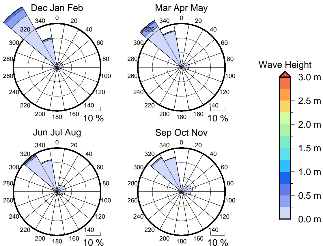
Figure 3 Seasonal wave roses for Vunisea
