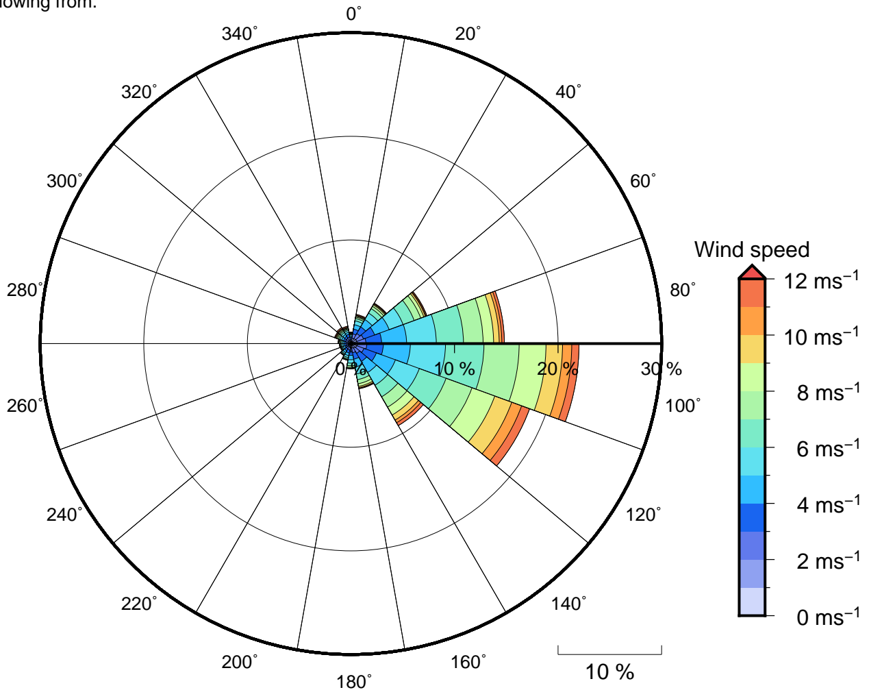
Figure 11 Annual wind rose for Vunisea. Note that directions are where the wind is coming from.
