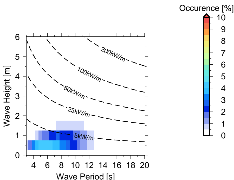
Figure 10 Occurrences of sea states in Votua Passage .
