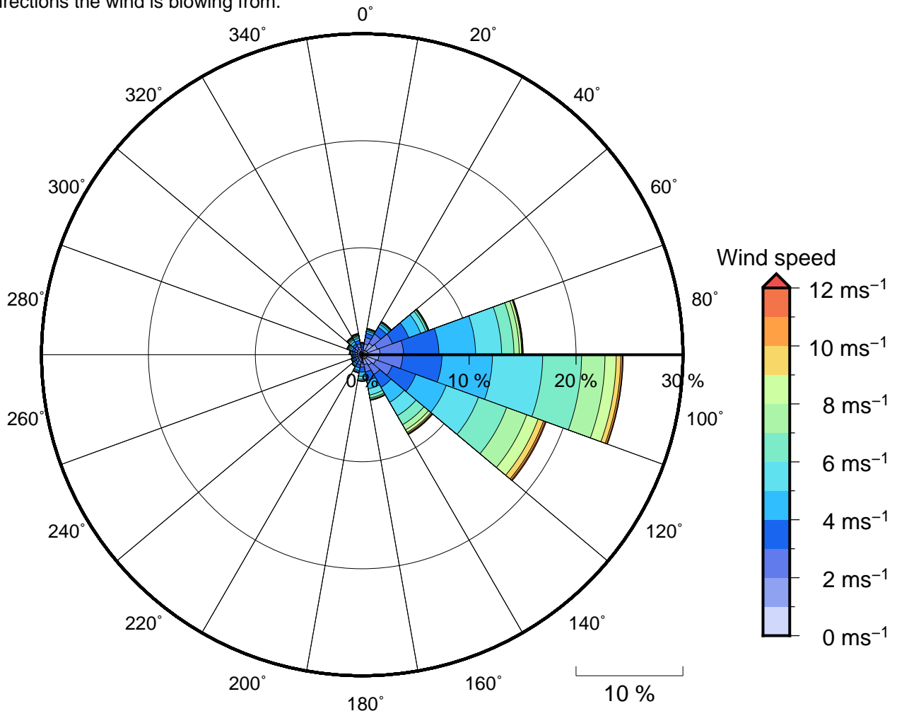
Figure 11 Annual wind rose for Votua Passage. Note that directions are where the wind is coming from.
