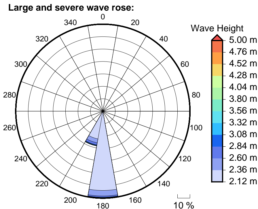
Figure 6 Large, severe and extreme wave roses for Votua Passage
