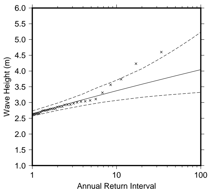
Figure 9 Extreme wave distribution for Votua Passage. The crosses represents the wave events that occurred since 1979. The plain line is the statistical distribution that best fit the past wave events. The dotted line show the upper and lower high confidence of the fit, there is a 95% chance that the fitted distribution lie between the two dashed lines.
