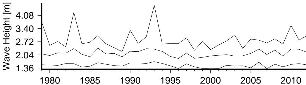
Figure 8 Annual variation in large waves (90th percentile)(lower curve), severe waves (99th percentile) (middle curve) and the largest wave(upper curve) in Votua Passage.
