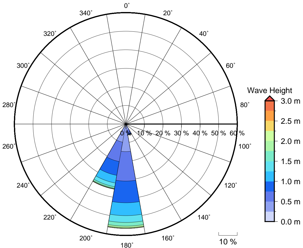
Figure 2 Annual wave rose for Votua Passage. Note that direction are where the wave are coming from .
