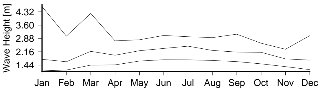
Figure 7 Monthly variation in large waves (90th percentile)(lower curve), severe waves (99th percentile) (middle curve) and the largest wave(upper curve) in Votua Passage.
