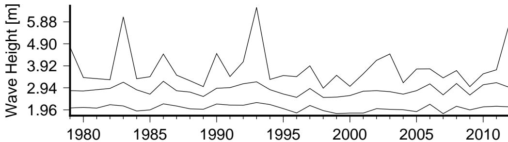
Figure 8 Annual variation in large waves (90th percentile)(lower curve), severe waves (99th percentile) (middle curve) and the largest wave(upper curve) in Viagra Reef.
