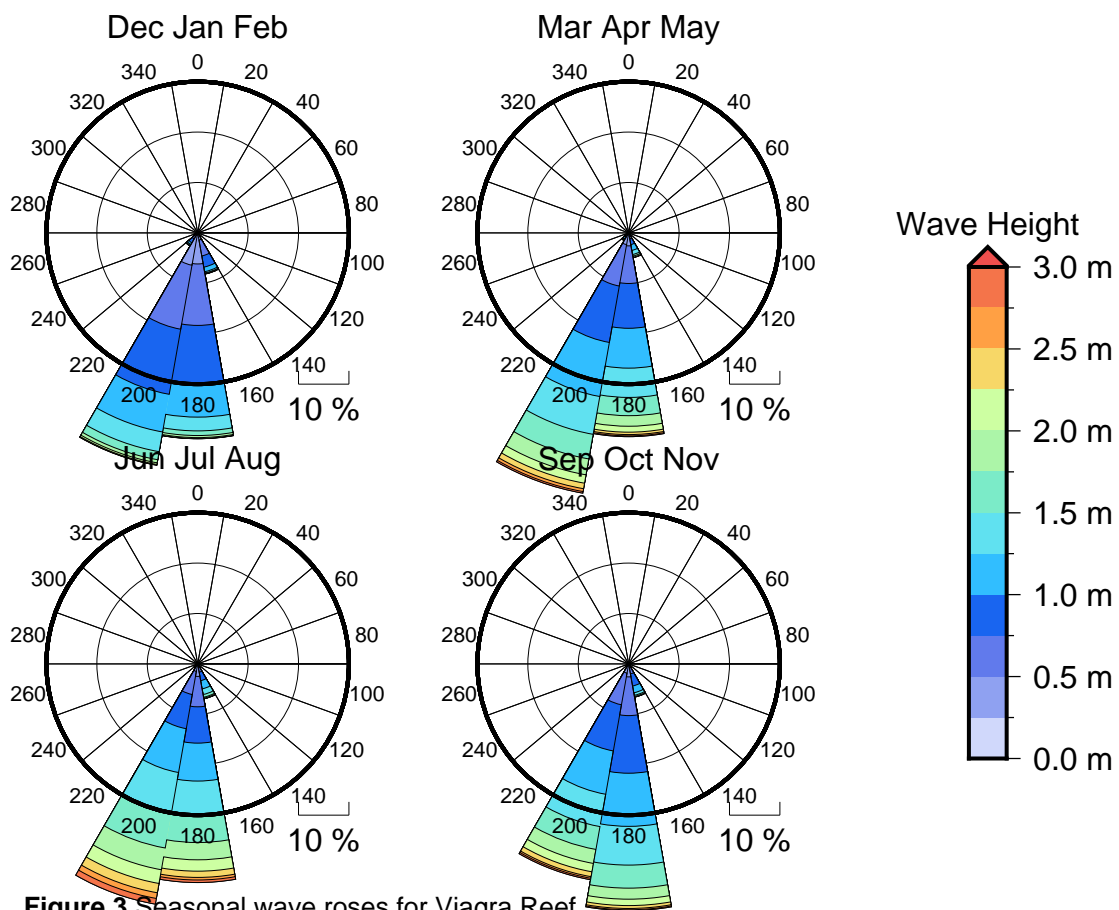
Figure 3 Seasonal wave roses for Viagra Reef
