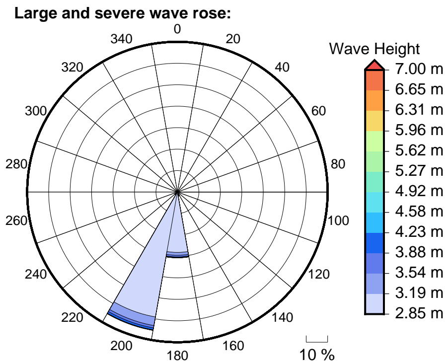
Figure 6 Large, severe and extreme wave roses for Viagra Reef
