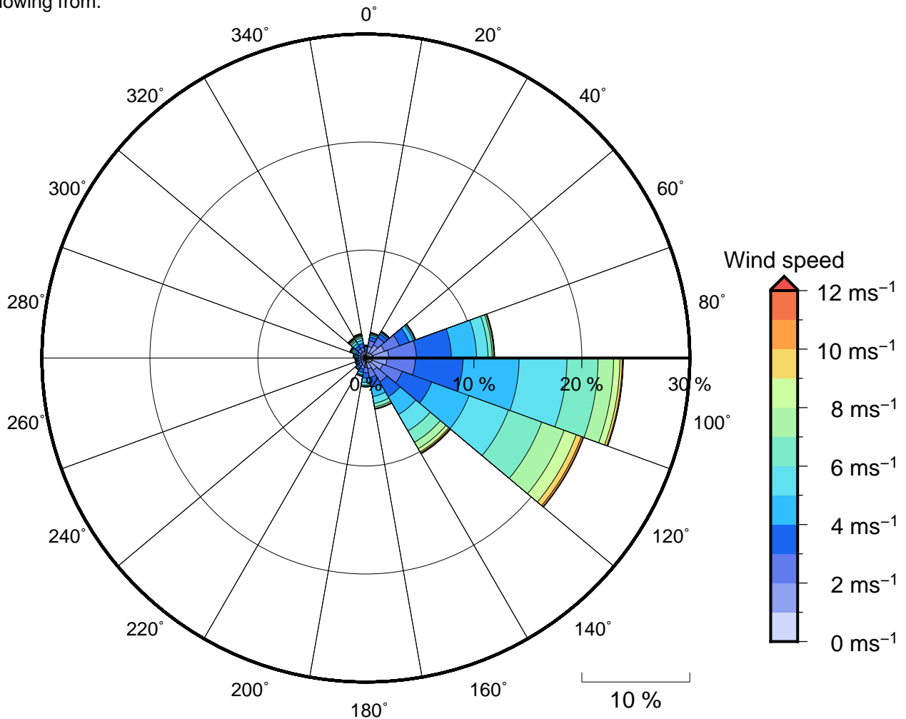
Figure 11 Annual wind rose for Viagra Reef. Note that directions are where the wind is coming from.
