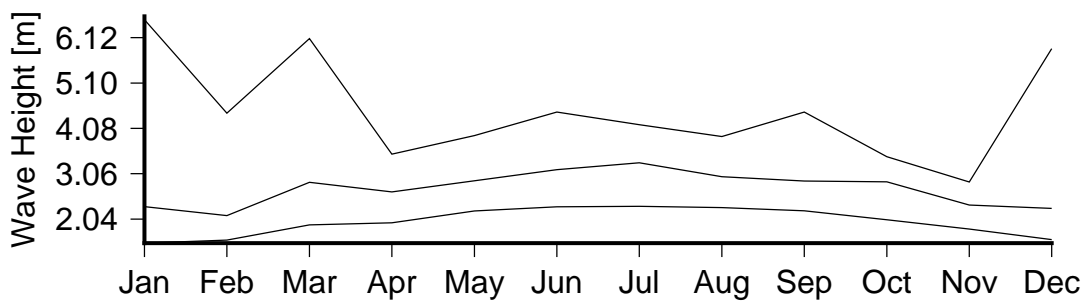
Figure 7 Monthly variation in large waves (90th percentile)(lower curve), severe waves (99th percentile) (middle curve) and the largest wave(upper curve) in Viagra Reef.
