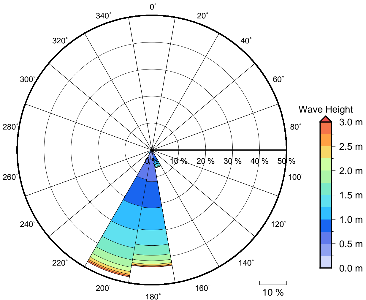
Figure 2 Annual wave rose for Viagra Reef. Note that direction are where the wave are coming from
