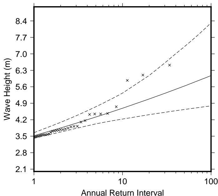
Figure 9 Extreme wave distribution for Viagra Reef. The crosses represents the wave events that occurred since 1979. The plain line is the statistical distribution that best fit the past wave events. The dotted line show the upper and lower high confidence of the fit, there is a 95% chance that the fitted distribution lie between the two dashed lines.
