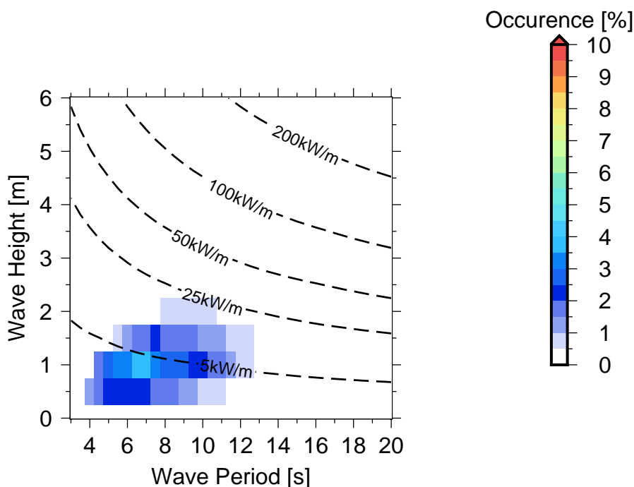
Figure 10 Occurrences of sea states in Viagra Reef .
