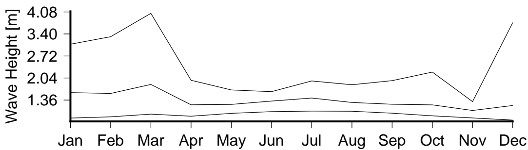
Figure 7 Monthly variation in large waves (90th percentile)(lower curve), severe waves (99th percentile) (middle curve) and the largest wave(upper curve) in Tavarua.
