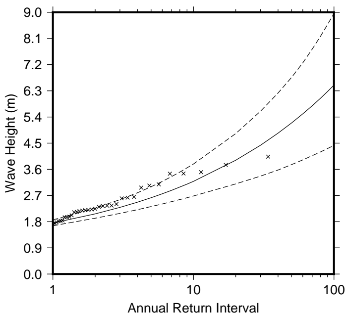
Figure 9 Extreme wave distribution for Tavarua. The crosses represents the wave events that occurred since 1979. The plain line is the statistical distribution that best fit the past wave events. The dotted line show the upper and lower high confidence of the fit, there is a 95% chance that the fitted distribution lie between the two dashed lines.
