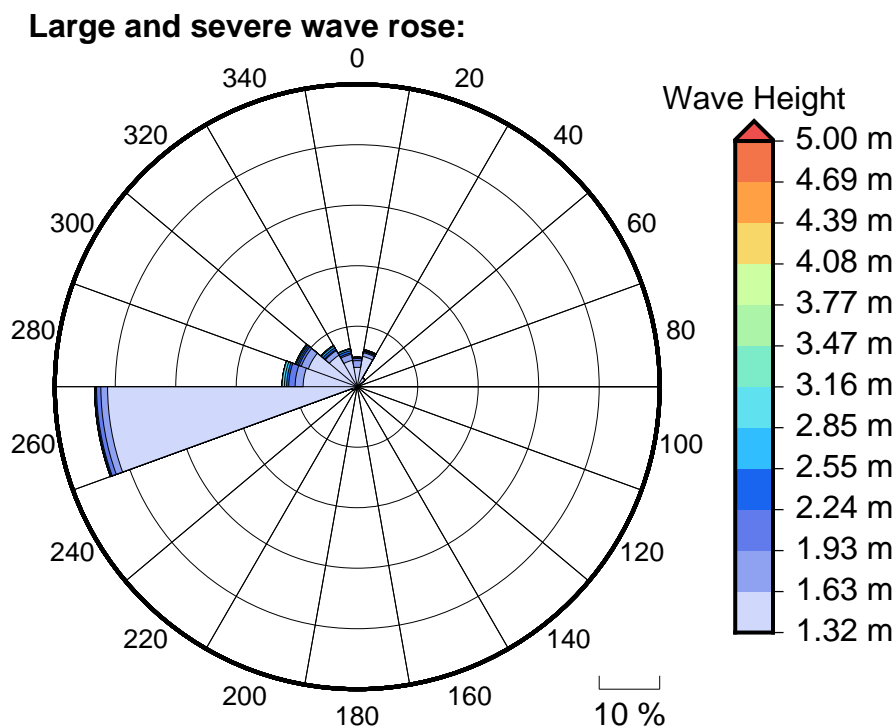
Figure 6 Large, severe and extreme wave roses for Tavarua
