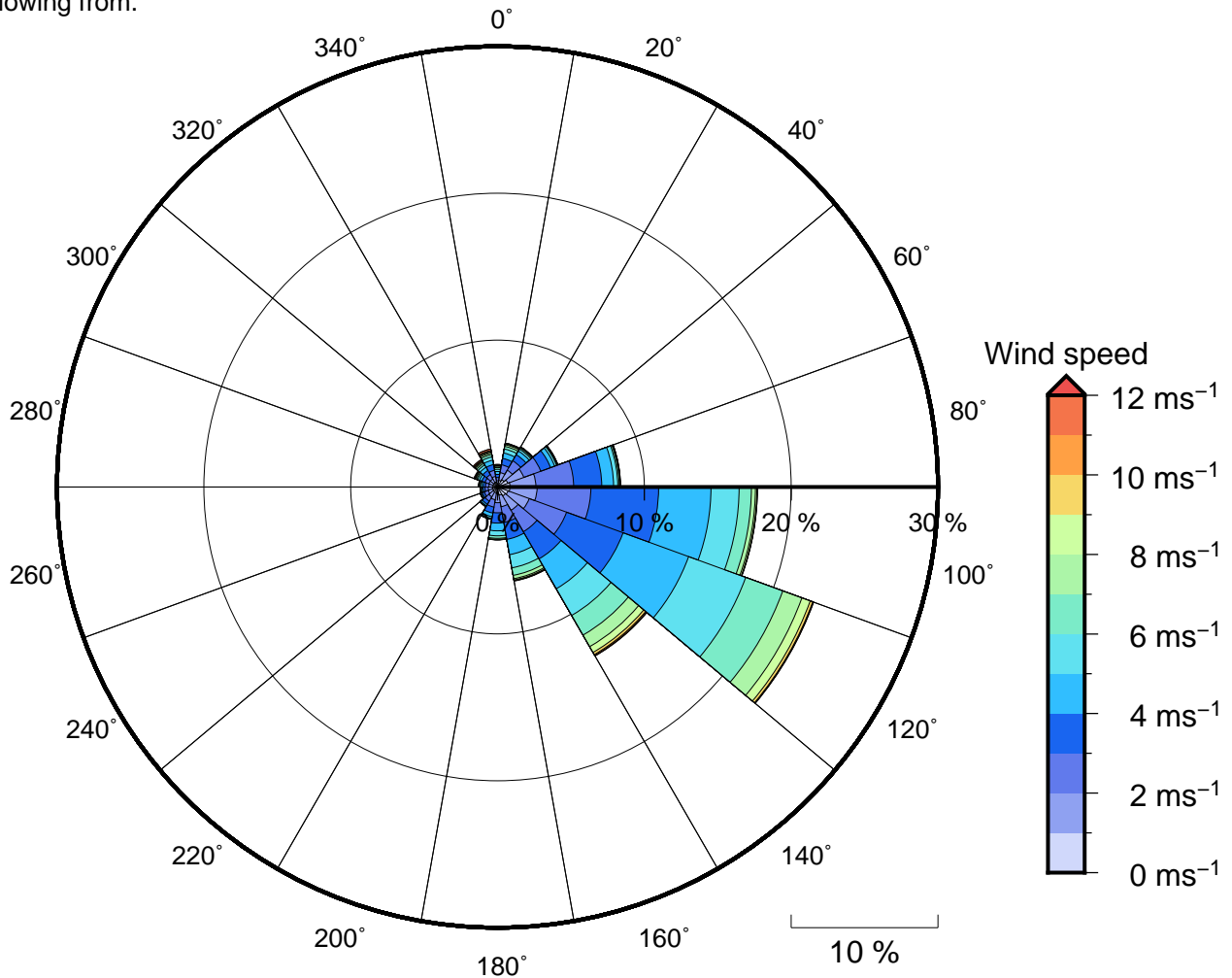
Figure 11 Annual wind rose for Tavarua. Note that directions are where the wind is coming from.
