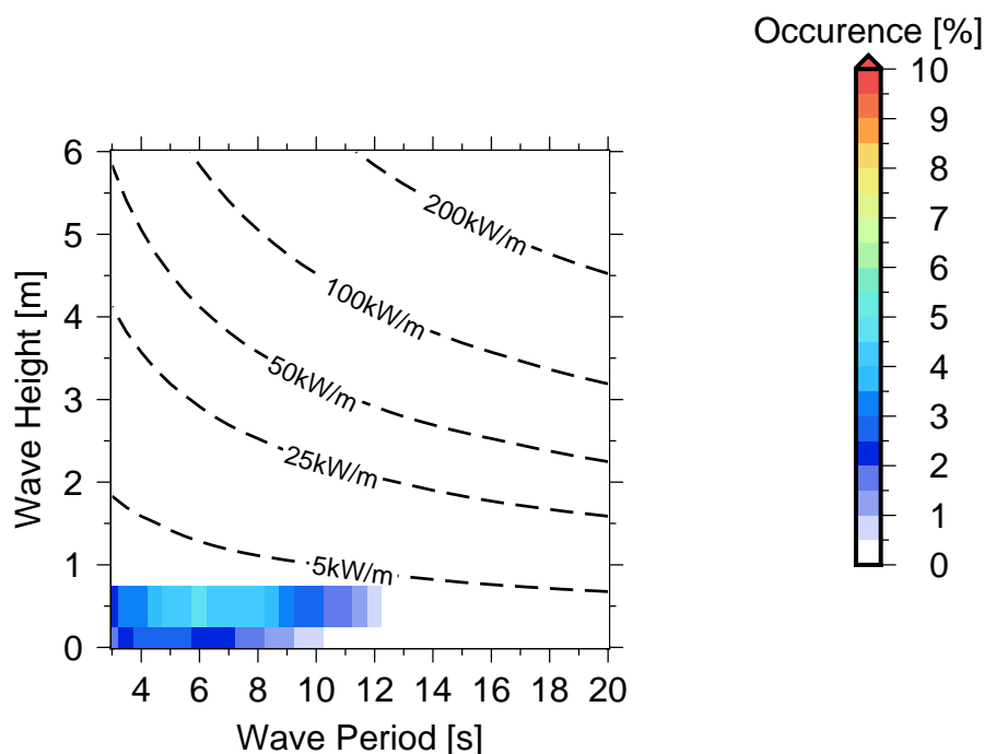
Figure 10 Occurrences of sea states in Tavarua .
