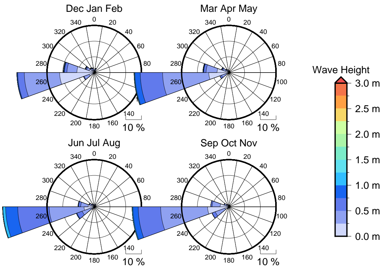
Figure 3 Seasonal wave roses for Tavarua
