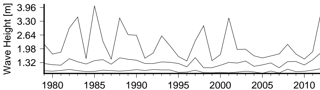
Figure 8 Annual variation in large waves (90th percentile)(lower curve), severe waves (99th percentile) (middle curve) and the largest wave(upper curve) in Tavarua.
