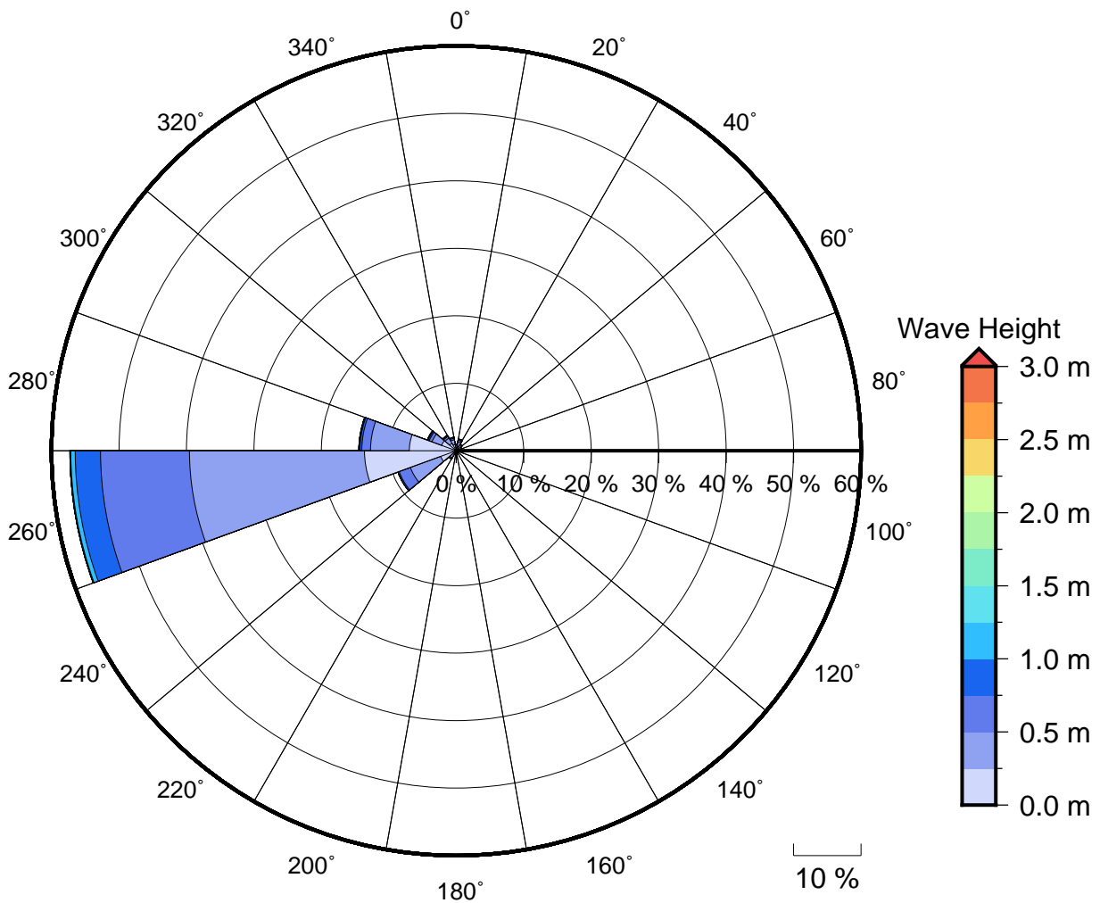
Figure 2 Annual wave rose for Tavarua. Note that direction are where the wave are coming from.
