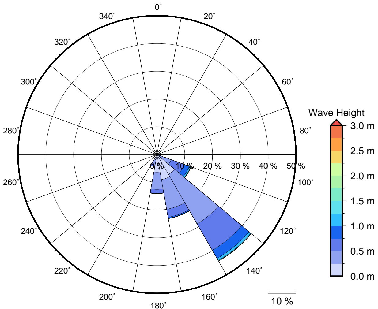
Figure 2 Annual wave rose for Taunovo Beach. Note that direction are where the wave are coming from .
