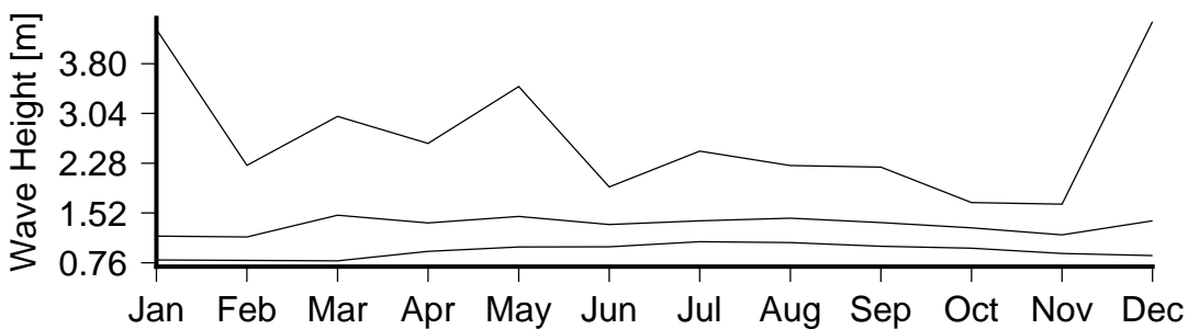
Figure 7 Monthly variation in large waves (90th percentile)(lower curve), severe waves (99th percentile) (middle curve) and the largest wave(upper curve) in Taunovo Beach.
