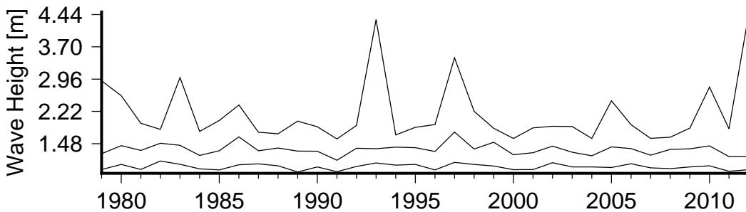
Figure 8 Annual variation in large waves (90th percentile)(lower curve), severe waves (99th percentile) (middle curve) and the largest wave(upper curve) in Taunovo Beach.
