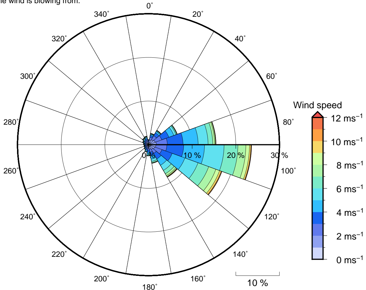
Figure 11 Annual wind rose for Taunovo Beach. Note that directions are where the wind is coming from.
