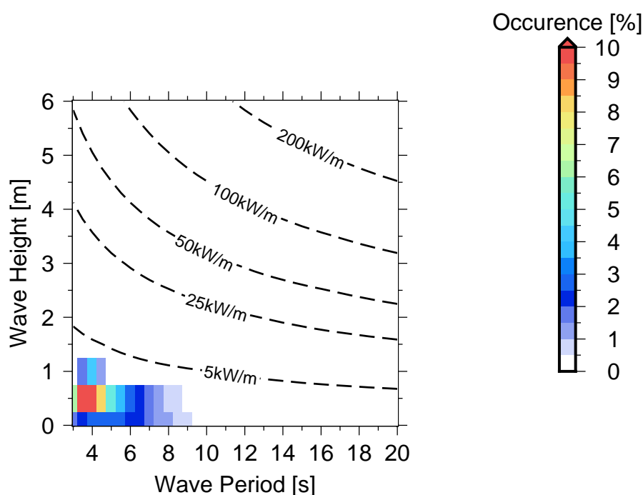
Figure 10 Occurrences of sea states in Taunovo Beach .
