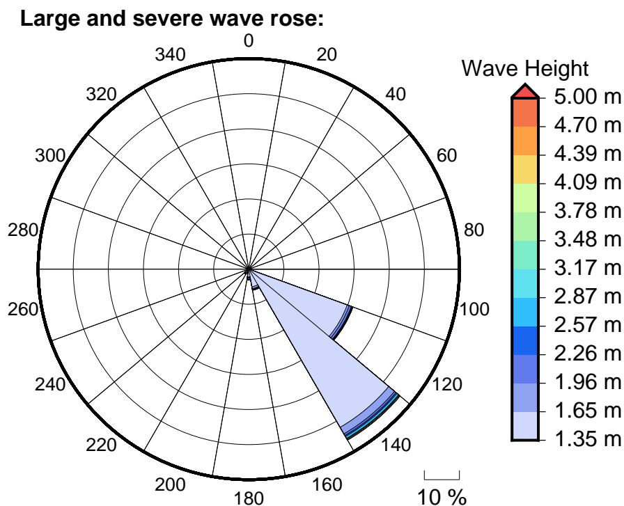
Figure 6 Large, severe and extreme wave roses for Taunovo Beach
