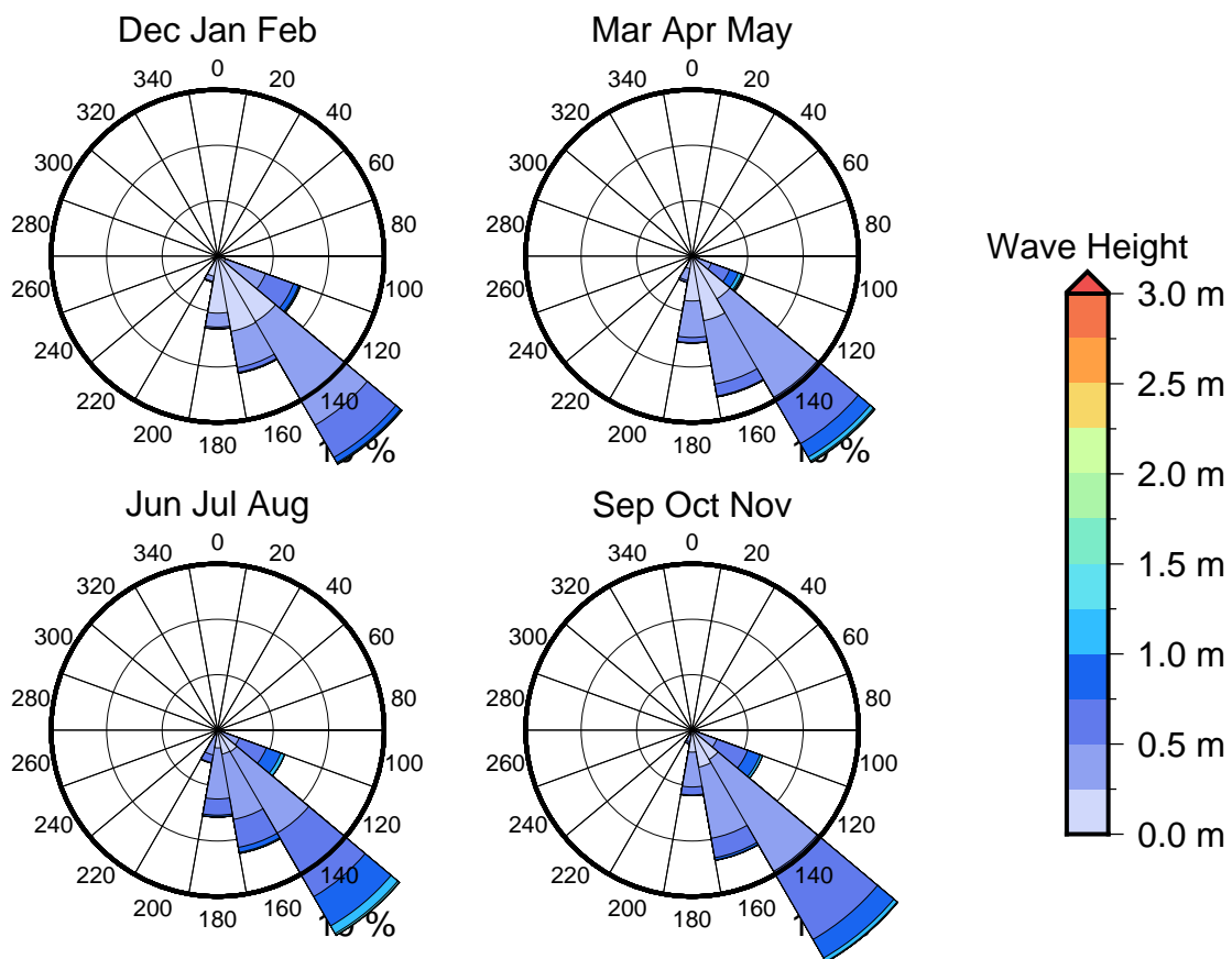
Figure 3 Seasonal wave roses for Taunovo Beach
