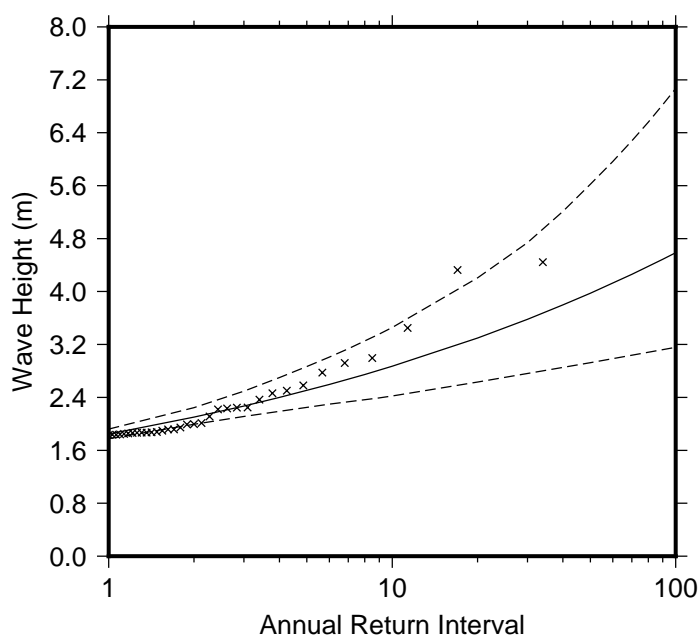
Figure 9 Extreme wave distribution for Taunovo Beach. The crosses represents the wave events that occurred since 1979. The plain line is the statistical distribution that best fit the past wave events. The dotted line show the upper and lower high confidence of the fit, there is a 95% chance that the fitted distribution lie between the two dashed lines.
