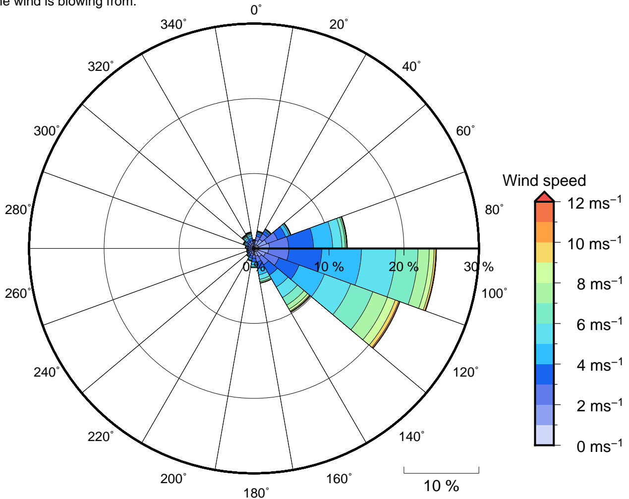
Figure 11 Annual wind rose for Tagage Passage. Note that directions are where the wind is coming from.
