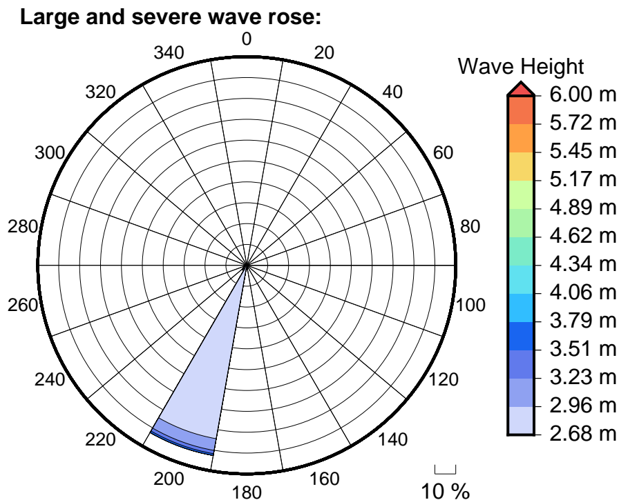
Figure 6 Large, severe and extreme wave roses for Tagage Passage
