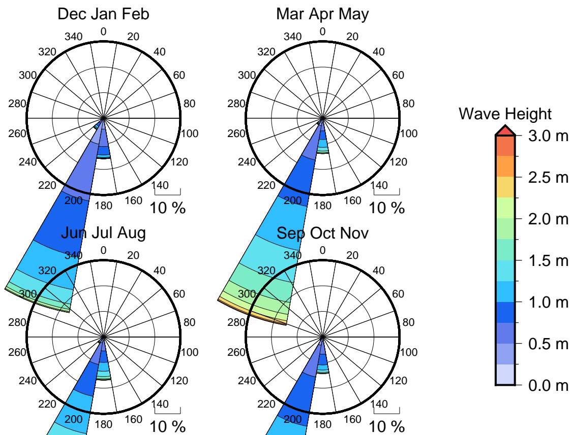
Figure 3 Seasonal wave roses for Tagage Passage
