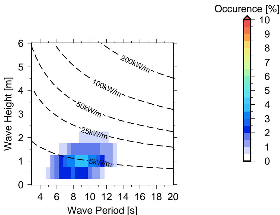
Figure 10 Occurrences of sea states in Tagage Passage .
