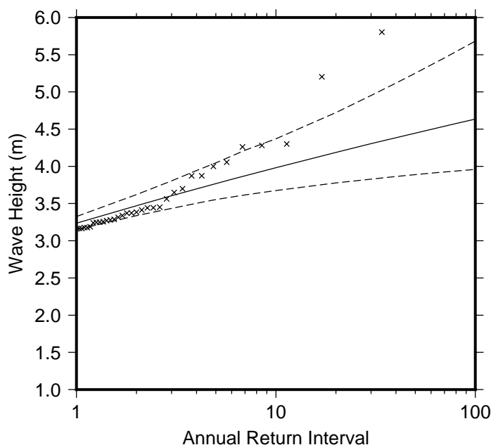
Figure 9 Extreme wave distribution for Tagage Passage. The crosses represents the wave events that occurred since 1979. The plain line is the statistical distribution that best fit the past wave events. The dotted line show the upper and lower high confidence of the fit, there is a 95% chance that the fitted distribution lie between the two dashed lines.
