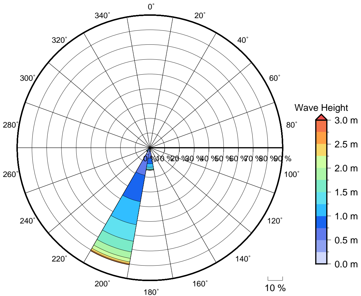
Figure 2 Annual wave rose for Tagage Passage. Note that direction are where the wave are coming from .
