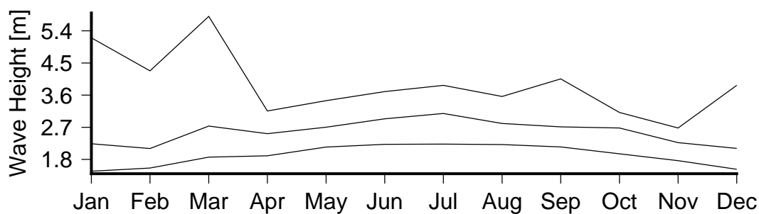
Figure 7 Monthly variation in large waves (90th percentile)(lower curve), severe waves (99th percentile) (middle curve) and the largest wave(upper curve) in Tagage Passage.
