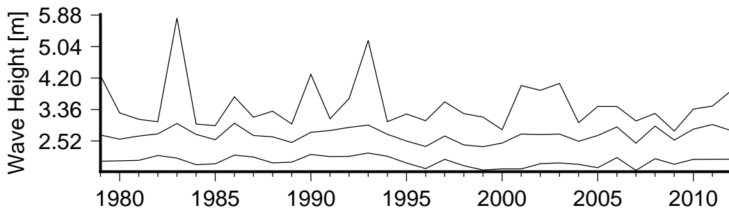
Figure 8 Annual variation in large waves (90th percentile)(lower curve), severe waves (99th percentile) (middle curve) and the largest wave(upper curve) in Tagage Passage.
