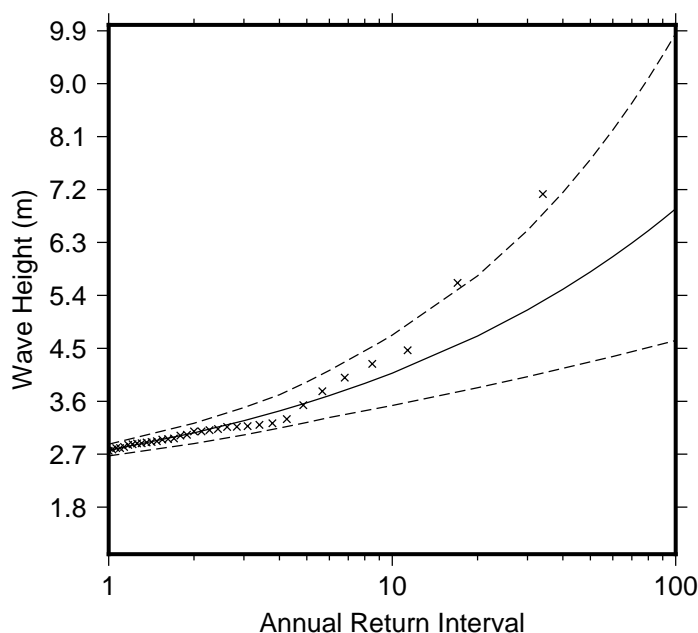
Figure 9 Extreme wave distribution for Suva Point Reef. The crosses represents the wave events that occurred since 1979. The plain line is the statistical distribution that best fit the past wave events. The dotted line show the upper and lower high confidence of the fit, there is a 95% chance that the fitted distribution lie between the two dashed lines.
