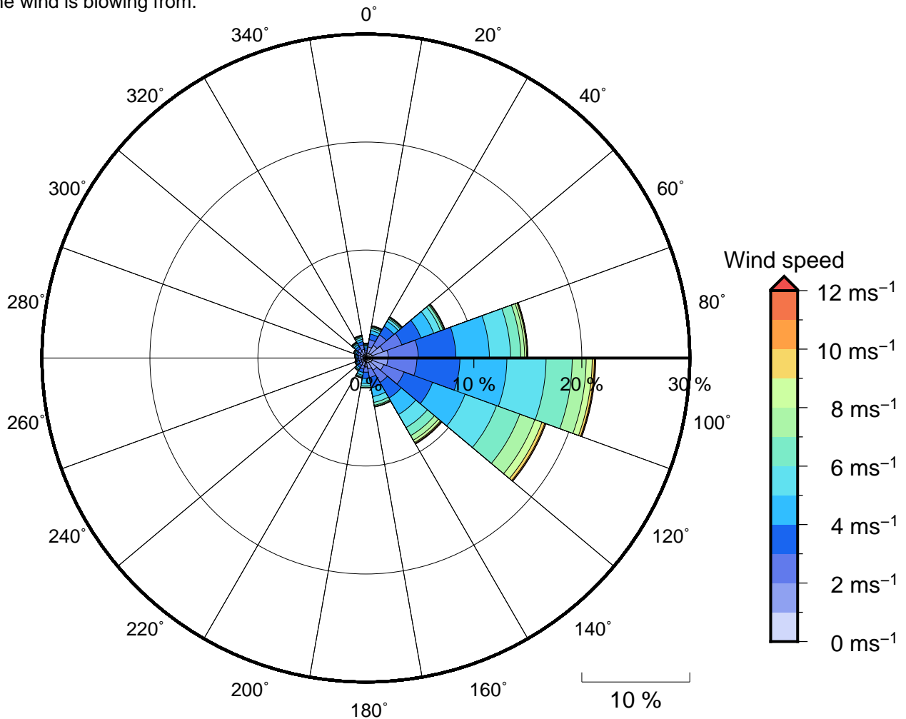
Figure 11 Annual wind rose for Suva Point Reef. Note that directions are where the wind is coming from.
