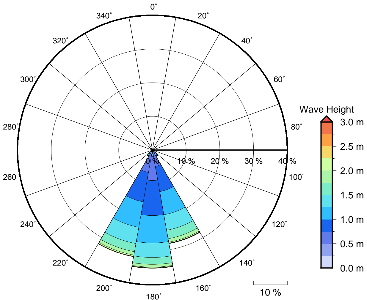
Figure 2 Annual wave rose for Suva Point Reef. Note that direction are where the wave are coming from .
