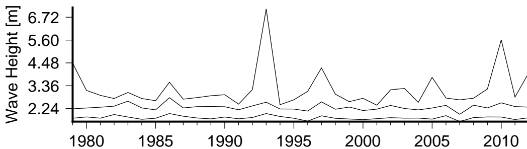
Figure 8 Annual variation in large waves (90th percentile)(lower curve), severe waves (99th percentile) (middle curve) and the largest wave(upper curve) in Suva Point Reef.
