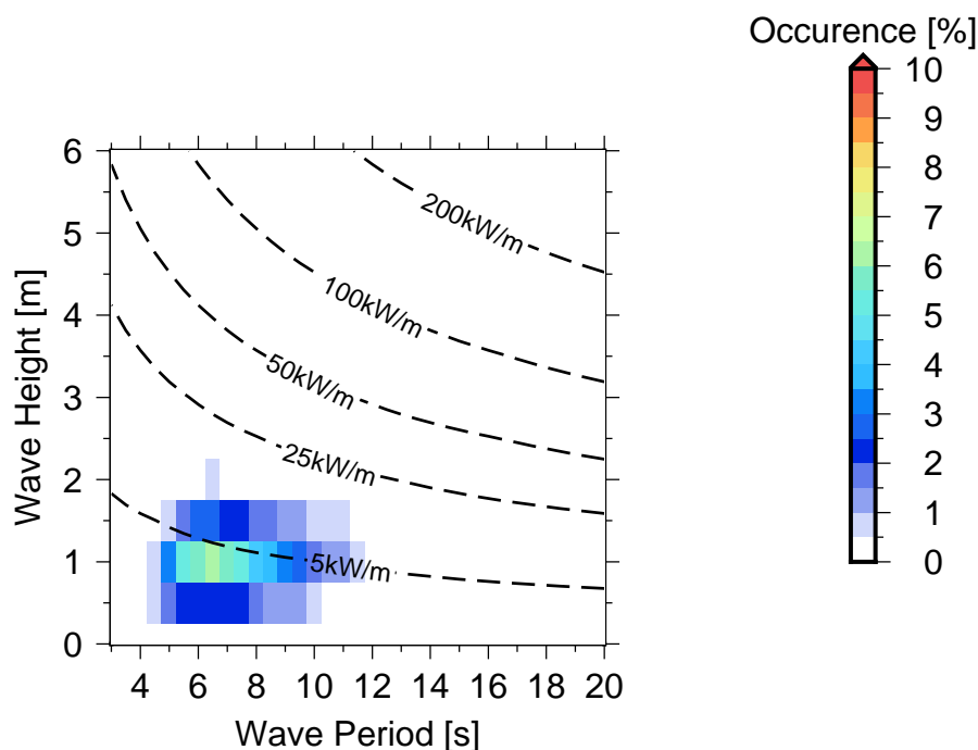
Figure 10 Occurrences of sea states in Suva Point Reef .
