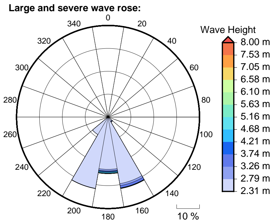
Figure 6 Large, severe and extreme wave roses for Suva Point Reef
