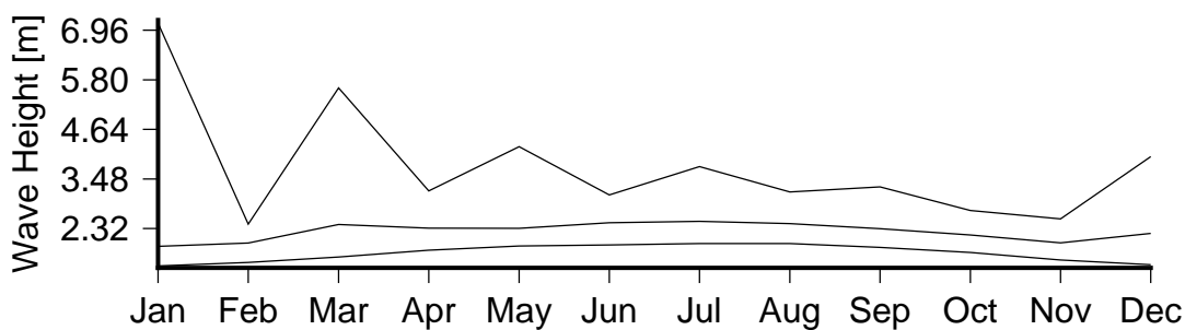
Figure 7 Monthly variation in large waves (90th percentile)(lower curve), severe waves (99th percentile) (middle curve) and the largest wave(upper curve) in Suva Point Reef.
