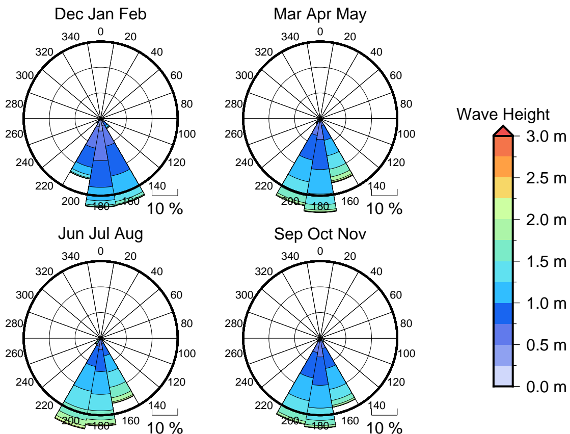
Figure 3 Seasonal wave roses for Suva Point Reef
