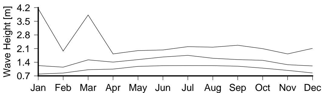
Figure 7 Monthly variation in large waves (90th percentile)(lower curve), severe waves (99th percentile) (middle curve) and the largest wave(upper curve) in Suva Harbour Passage.
