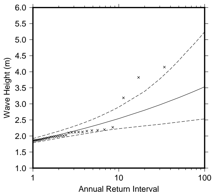
Figure 9 Extreme wave distribution for Suva Harbour Passage. The crosses represents the wave events that occurred since 1979. The plain line is the statistical distribution that best fit the past wave events. The dotted line show the upper and lower high confidence of the fit, there is a 95% chance that the fitted distribution lie between the two dashed lines.
