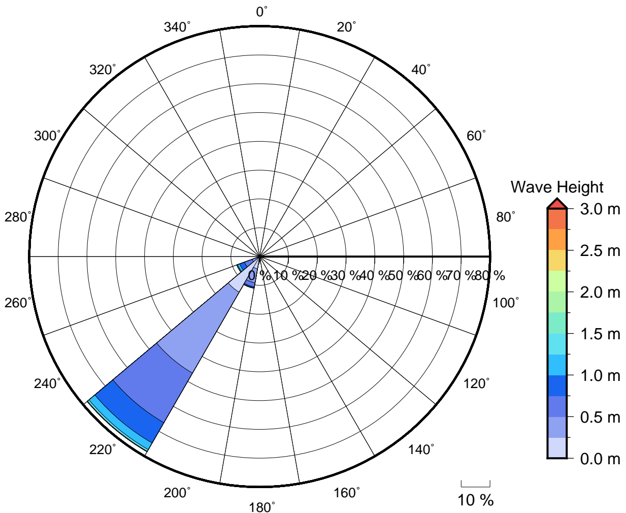
Figure 2 Annual wave rose for Suva Harbour Passage. Note that direction are where the wave are coming from.
