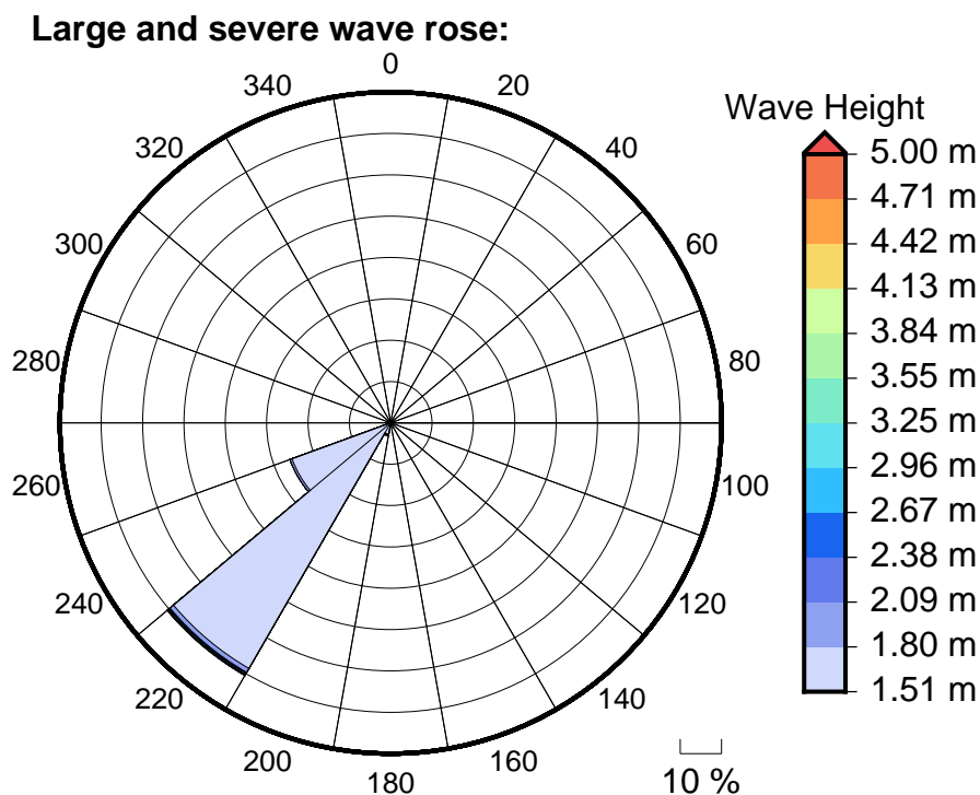
Figure 6 Large, severe and extreme wave roses for Suva Harbour Passage
