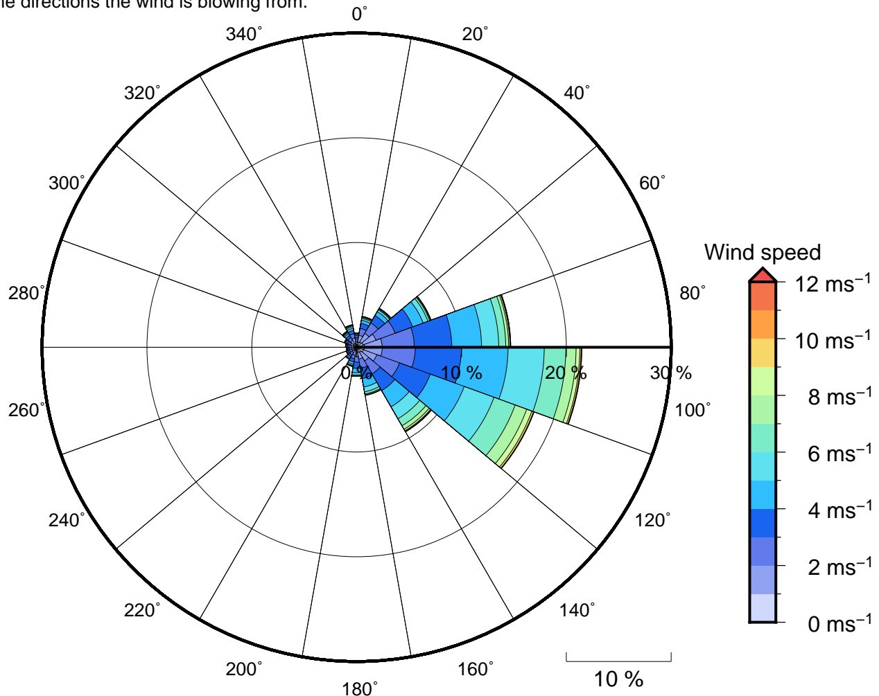
Figure 11 Annual wind rose for Suva Harbour Passage. Note that directions are where the wind is coming from.
