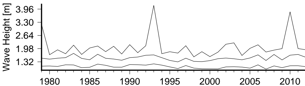
Figure 8 Annual variation in large waves (90th percentile)(lower curve), severe waves (99th percentile) (middle curve) and the largest wave(upper curve) in Suva Harbour Passage.
