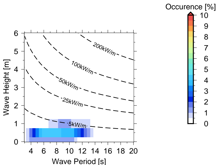
Figure 10 Occurrences of sea states in Suva Harbour Passage .
