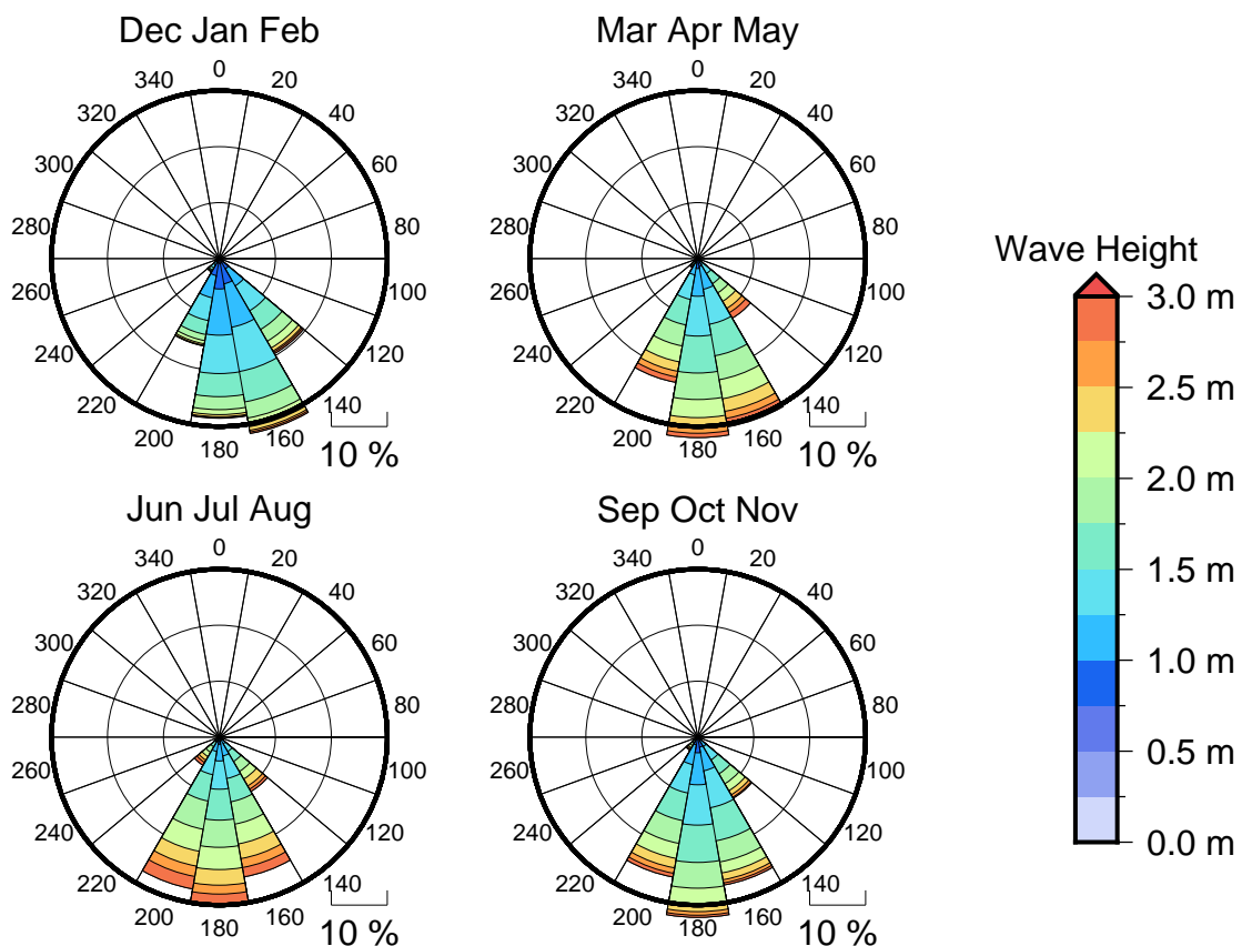
Figure 3 Seasonal wave roses for South West Kadavu
