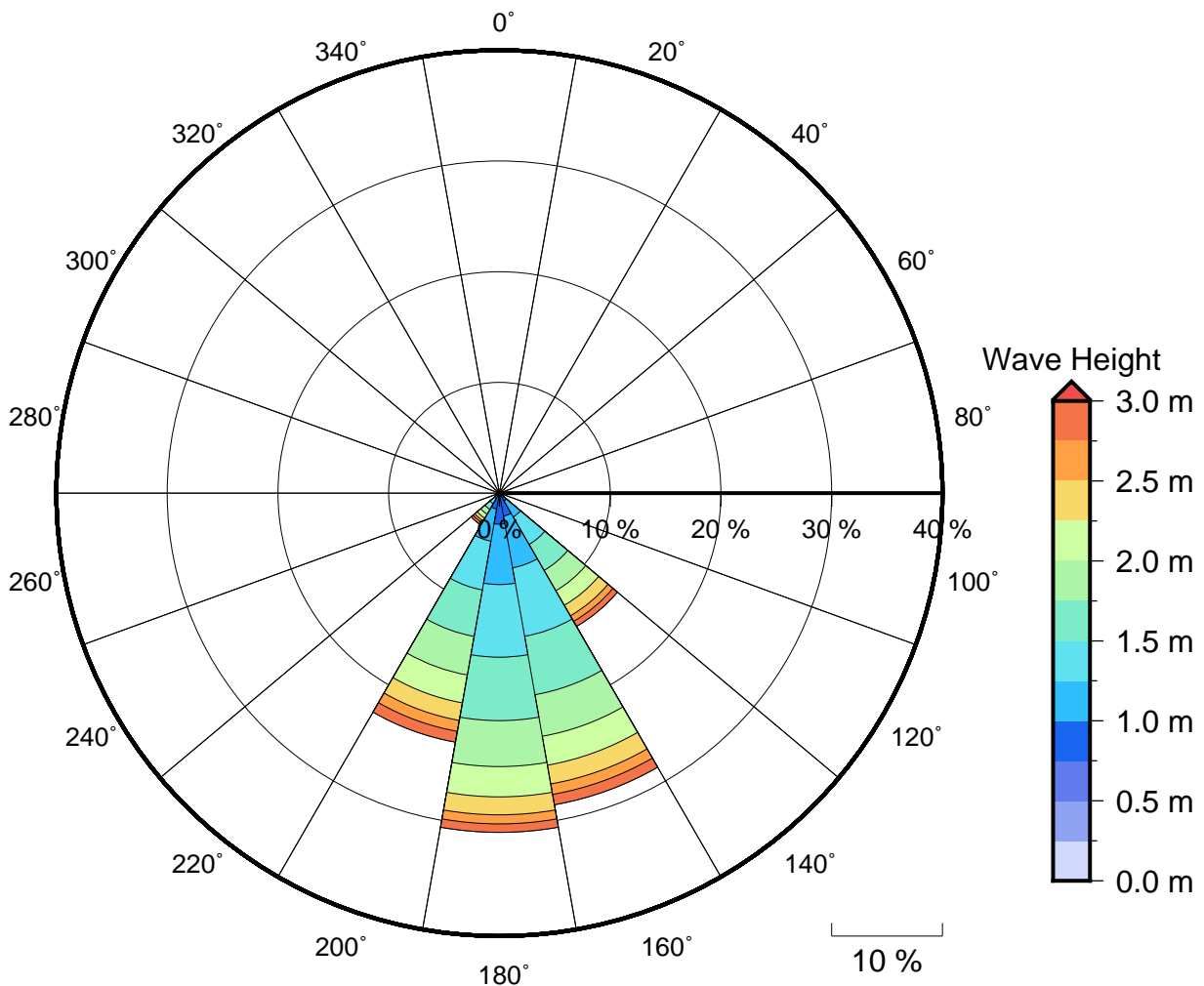
Figure 2 Annual wave rose for South West Kadavu. Note that direction are where the wave are coming from.
