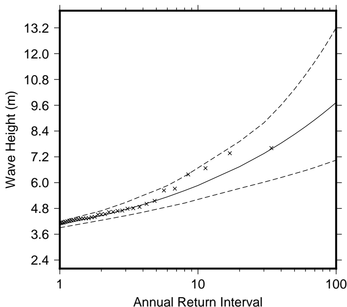
Figure 9 Extreme wave distribution for South West Kadavu. The crosses represents the wave events that occurred since 1979. The plain line is the statistical distribution that best fit the past wave events. The dotted line show the upper and lower high confidence of the fit, there is a 95% chance that the fitted distribution lie between the two dashed lines.
