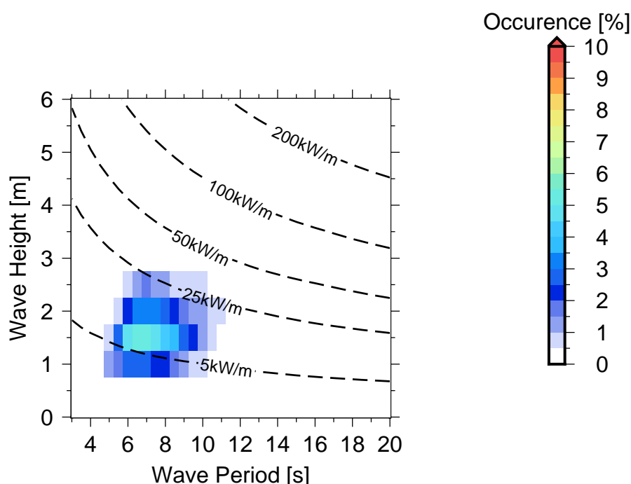
Figure 10 Occurrences of sea states in South West Kadavu .
