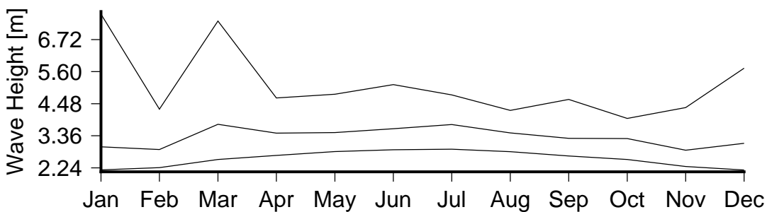
Figure 7 Monthly variation in large waves (90th percentile)(lower curve), severe waves (99th percentile) (middle curve) and the largest wave(upper curve) in South West Kadavu.
