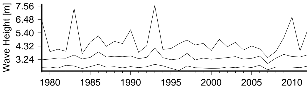
Figure 8 Annual variation in large waves (90th percentile)(lower curve), severe waves (99th percentile) (middle curve) and the largest wave(upper curve) in South West Kadavu.
