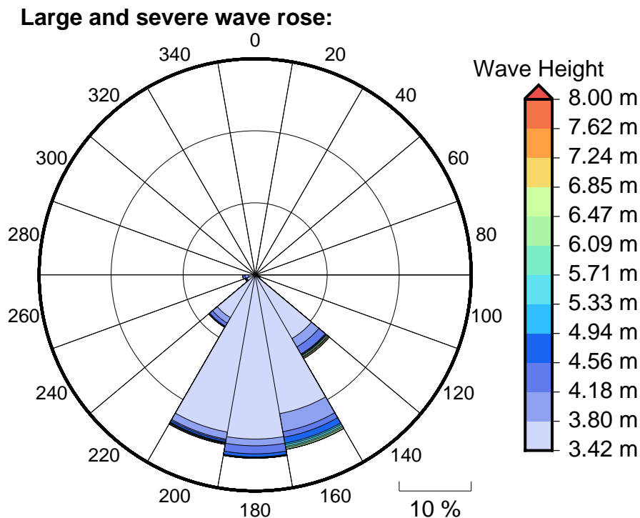
Figure 6 Large, severe and extreme wave roses for South West Kadavu
