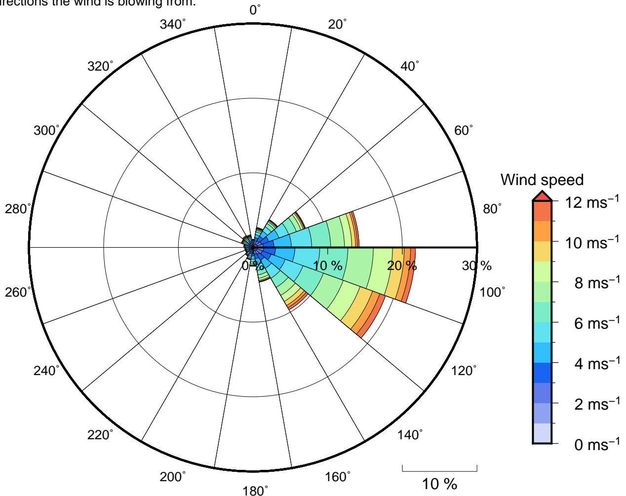
Figure 11 Annual wind rose for South West Kadavu. Note that directions are where the wind is coming from.
