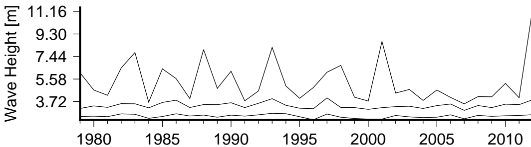
Figure 8 Annual variation in large waves (90th percentile)(lower curve), severe waves (99th percentile) (middle curve) and the largest wave(upper curve) in South Vatulele.
