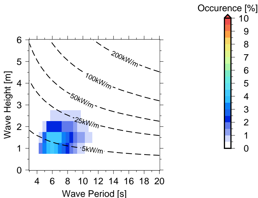
Figure 10 Occurences of sea states in South Vatulele .
