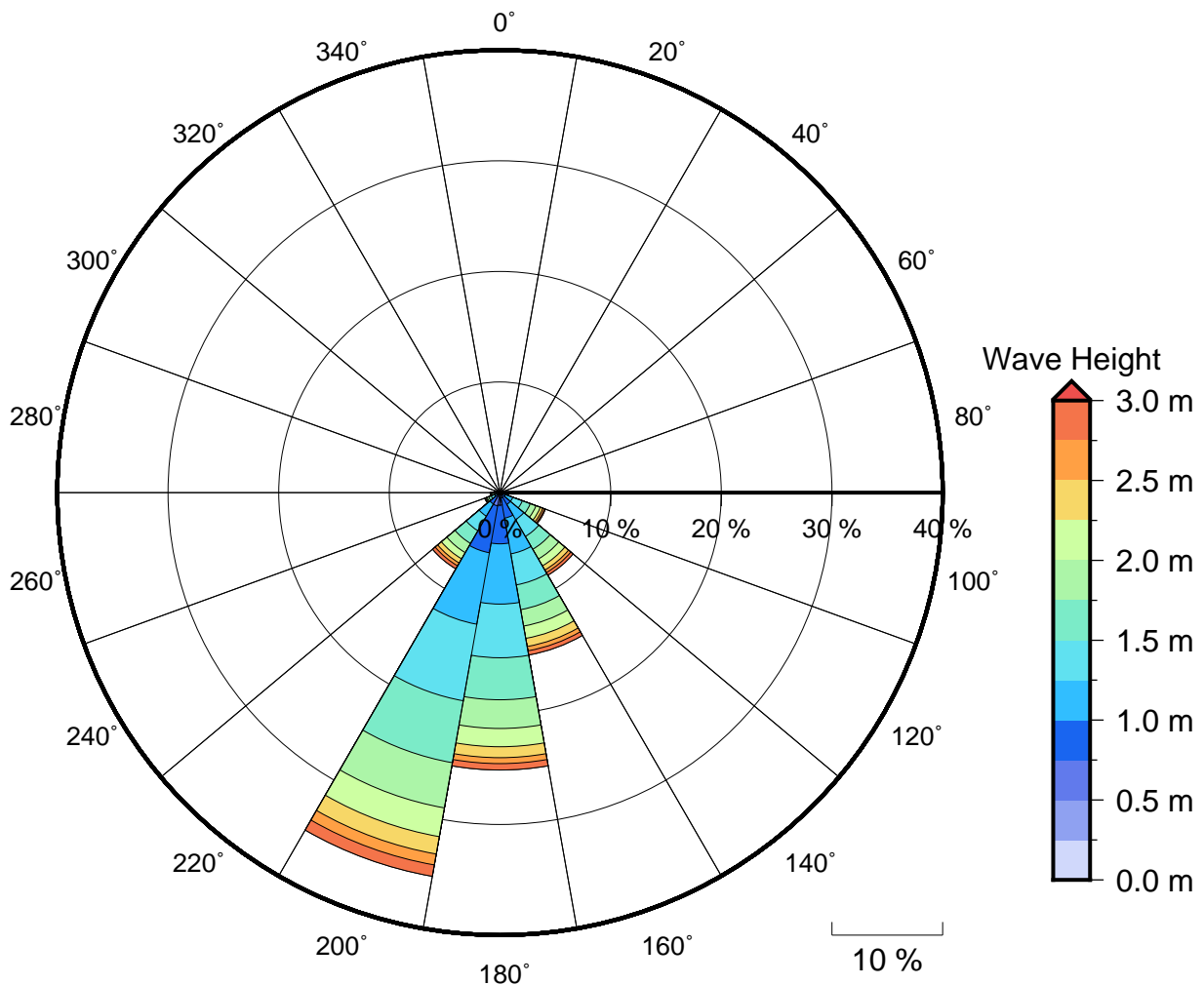
Figure 2 Annual wave rose for South Vatulele. Note that direction are where the wave are coming from .
