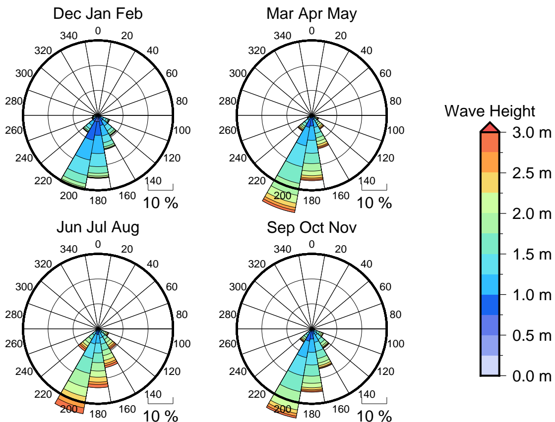
Figure 3 Seasonal wave roses for South Vatulele
