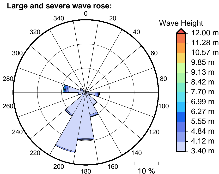
Figure 6 Large, severe and extreme wave roses for South Vatulele
