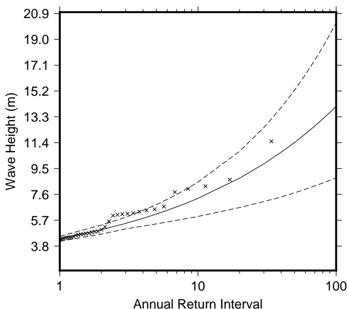
Figure 9 Extreme wave distribution for South Vatulele. The crosses represents the wave events that occurred since 1979. The plain line is the statistical distribution that best fit the past wave events. The dotted line show the upper and lower high confidence of the fit, there is a 95% chance that the fitted distribution lie between the two dashed lines.
