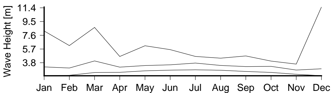
Figure 7 Monthly variation in large waves (90th percentile)(lower curve), severe waves (99th percentile) (middle curve) and the largest wave(upper curve) in South Vatulele.
