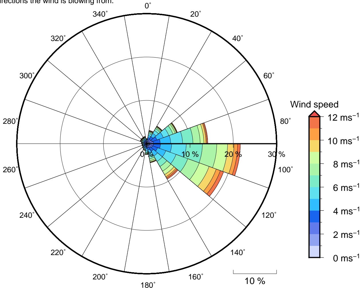
Figure 11 Annual wind rose for South Kadavu. Note that directions are where the wind is coming from.
