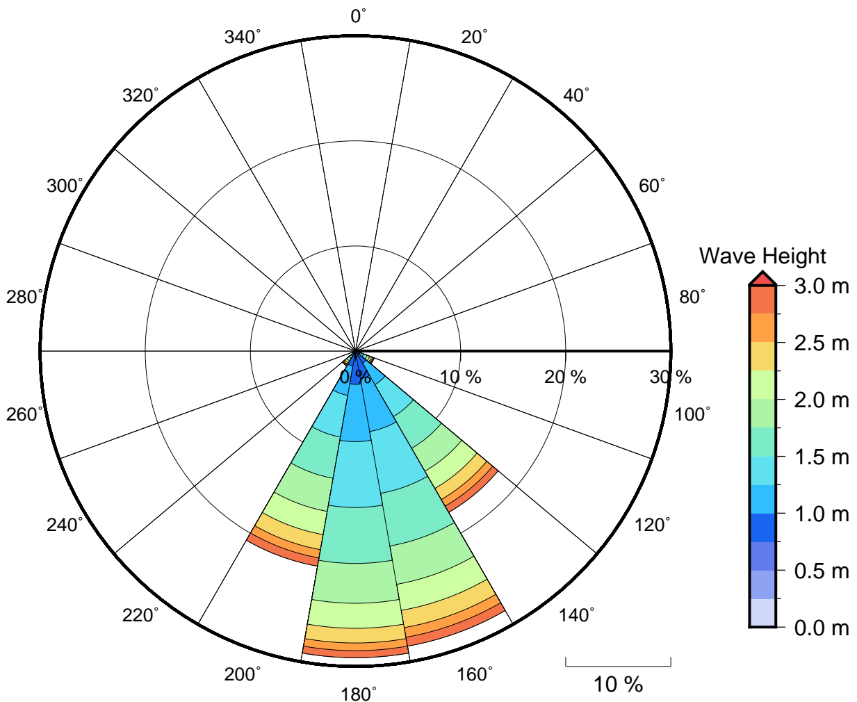
Figure 2 Annual wave rose for South Kadavu. Note that direction are where the wave are coming from .
