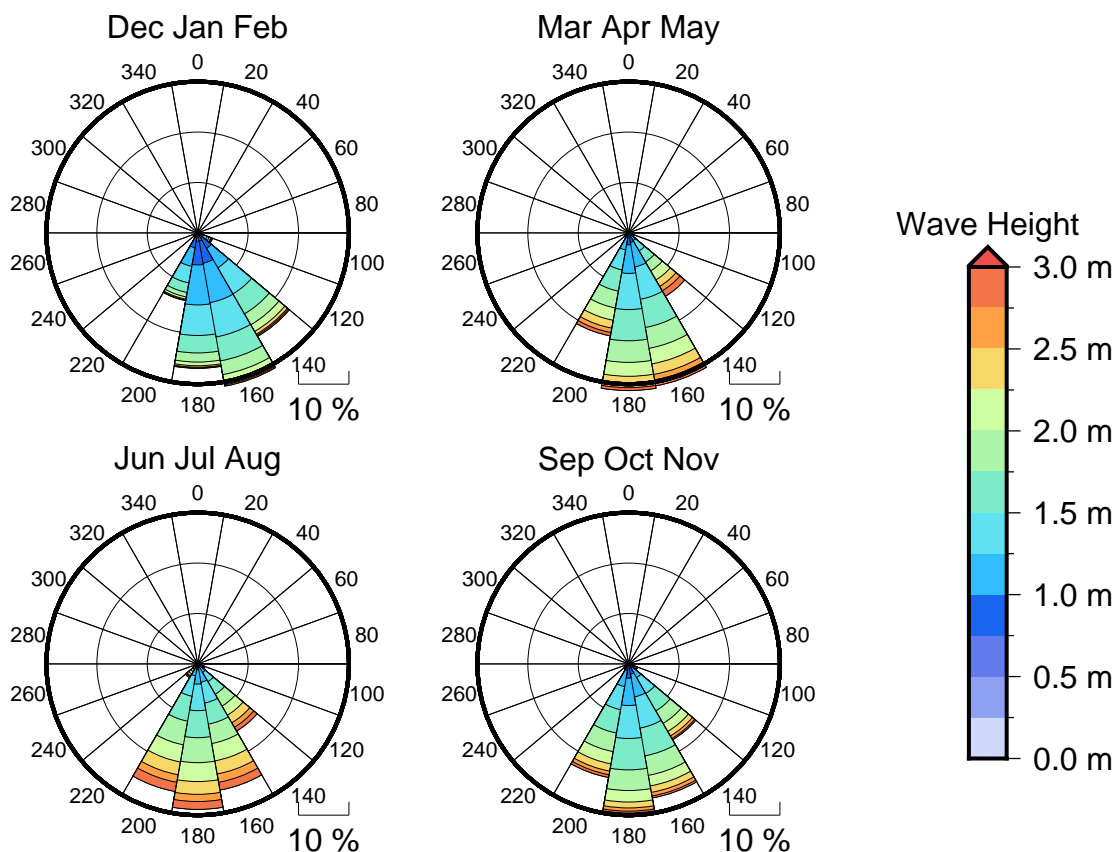
Figure 3 Seasonal wave roses for South Kadavu
