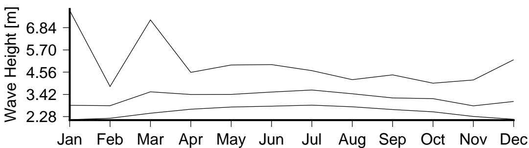
Figure 7 Monthly variation in large waves (90th percentile)(lower curve), severe waves (99th percentile) (middle curve) and the largest wave(upper curve) in South Kadavu.
