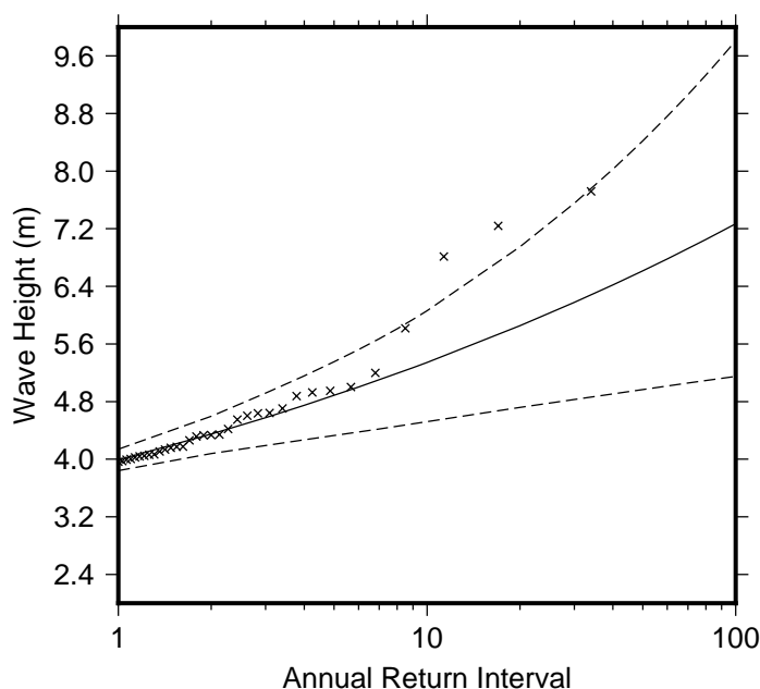
Figure 9 Extreme wave distribution for South Kadavu. The crosses represents the wave events that occurred since 1979. The plain line is the statistical distribution that best fit the past wave events. The dotted line show the upper and lower high confidence of the fit, there is a 95% chance that the fitted distribution lie between the two dashed lines.
