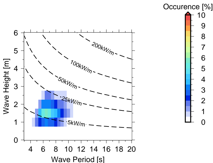
Figure 10 Occurrences of sea states in South Kadavu .
