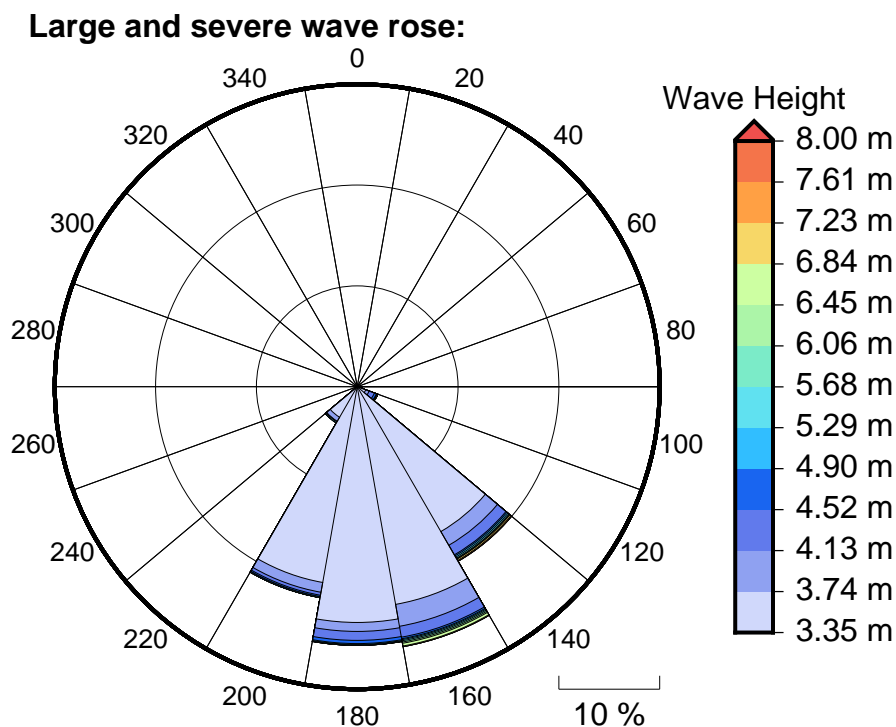
Figure 6 Large, severe and extreme wave roses for South Kadavu
