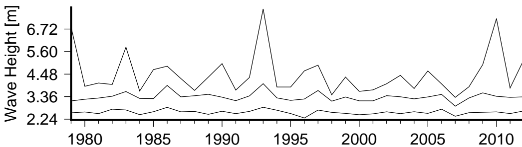
Figure 8 Annual variation in large waves (90th percentile)(lower curve), severe waves (99th percentile) (middle curve) and the largest wave(upper curve) in South Kadavu.
