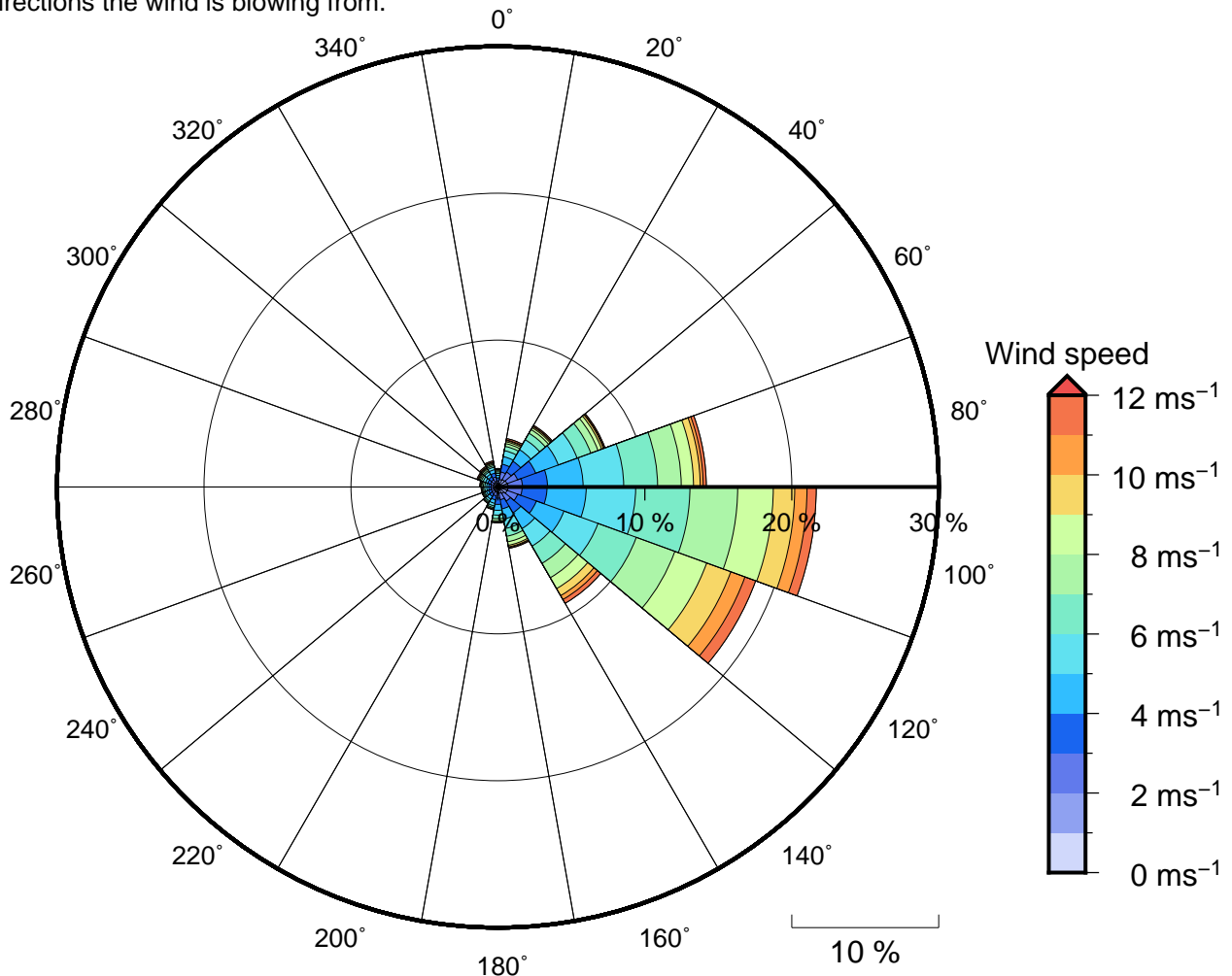
Figure 11 Annual wind rose for South East Kadavu. Note that directions are where the wind is coming from.
