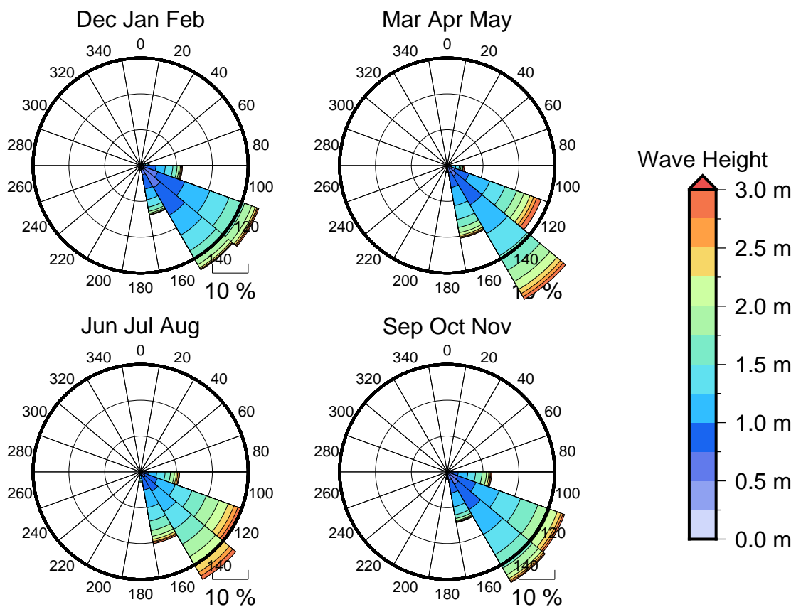
Figure 3 Seasonal wave roses for South East Kadavu
