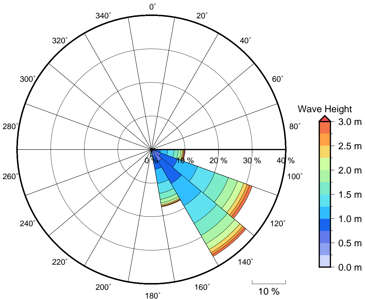
Figure 2 Annual wave rose for South East Kadavu. Note that direction are where the wave are coming from.
