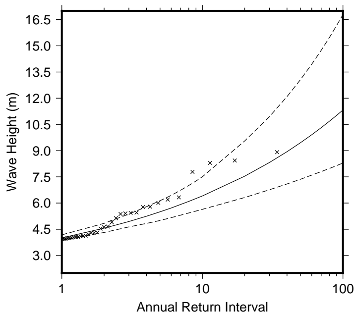
Figure 9 Extreme wave distribution for South East Kadavu. The crosses represents the wave events that occurred since 1979. The plain line is the statistical distribution that best fit the past wave events. The dotted line show the upper and lower high confidence of the fit, there is a 95% chance that the fitted distribution lie between the two dashed lines.
