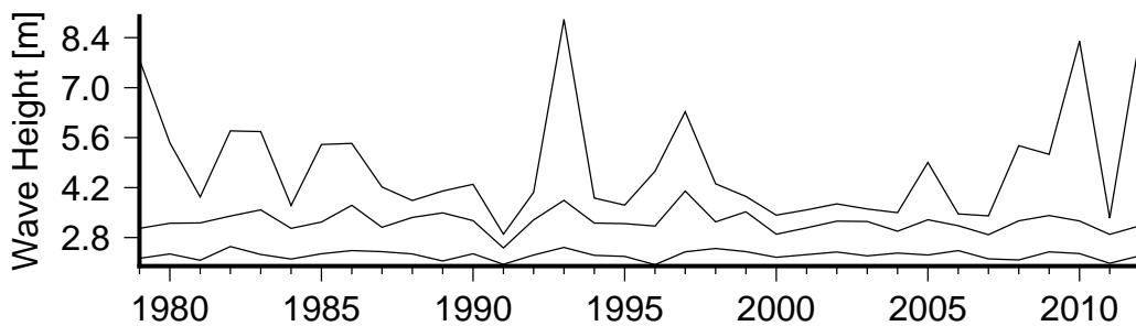
Figure 8 Annual variation in large waves (90th percentile)(lower curve), severe waves (99th percentile) (middle curve) and the largest wave(upper curve) in South East Kadavu.
