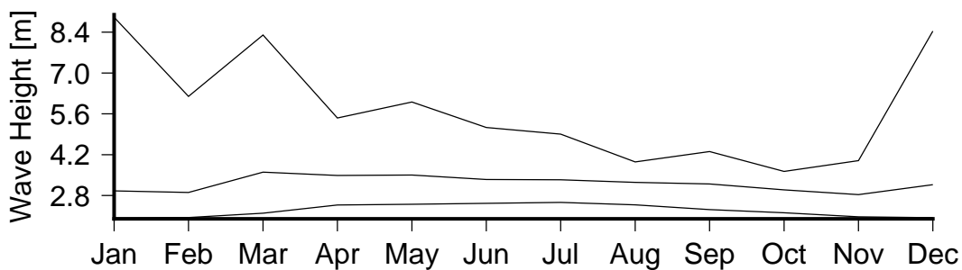
Figure 7 Monthly variation in large waves (90th percentile)(lower curve), severe waves (99th percentile) (middle curve) and the largest wave(upper curve) in South East Kadavu.
