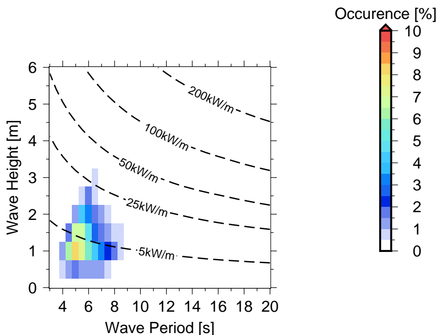
Figure 10 Occurrences of sea states in South East Kadavu .
