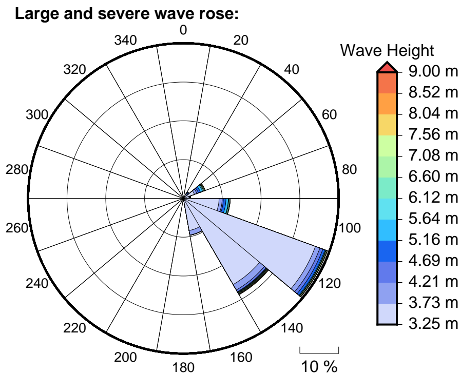
Figure 6 Large, severe and extreme wave roses for South East Kadavu
