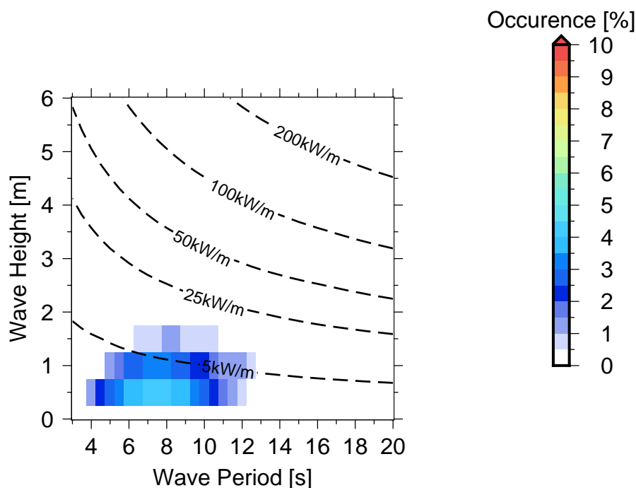
Figure 10 Occurrences of sea states in Somosomo Bay .
