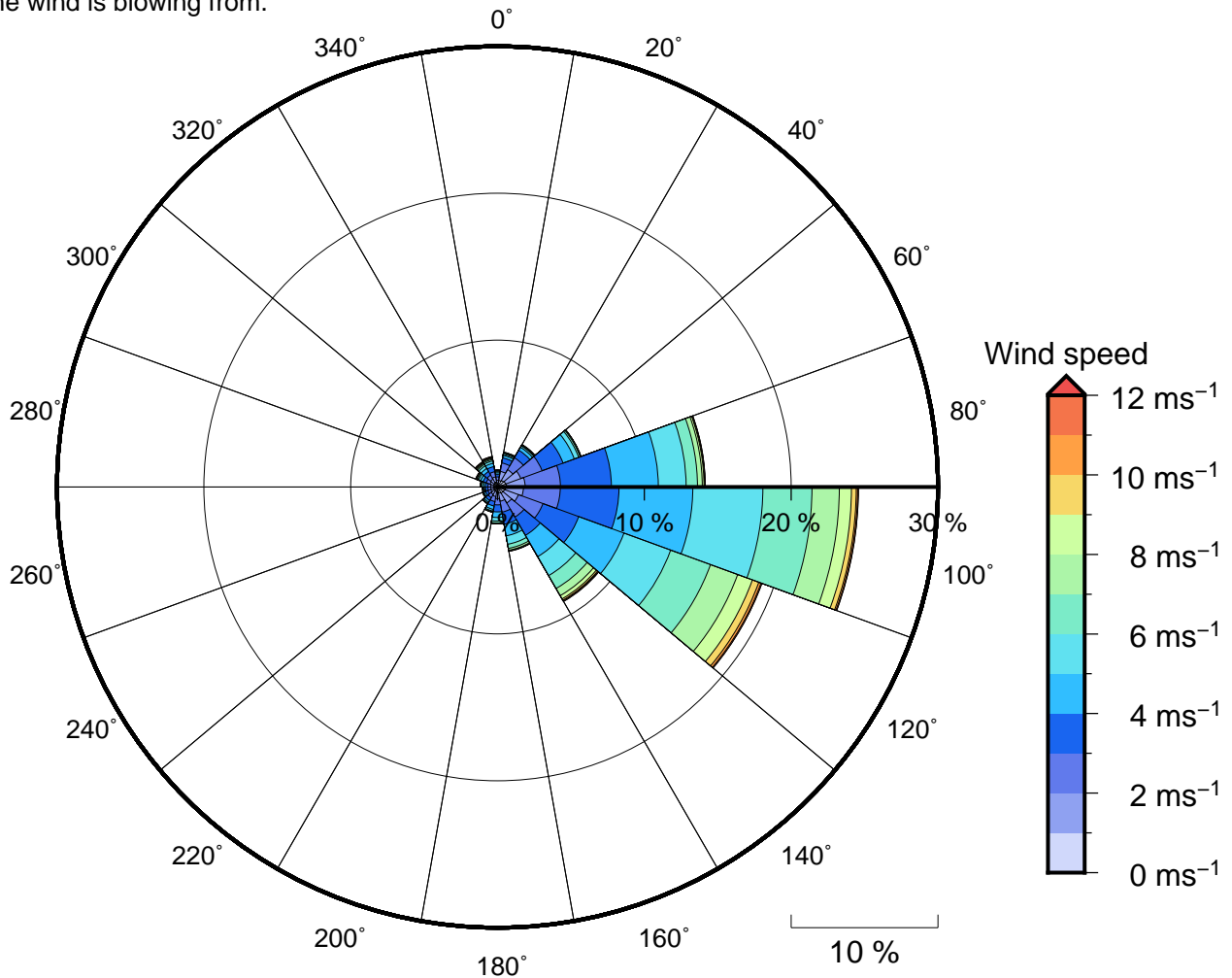
Figure 11 Annual wind rose for Somosomo Bay. Note that directions are where the wind is coming from.
