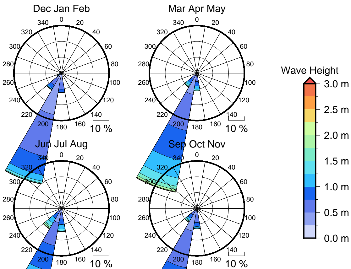
Figure 3 Seasonal wave roses for Somosomo Bay
