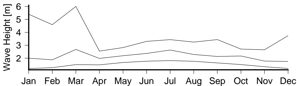
Figure 7 Monthly variation in large waves (90th percentile)(lower curve), severe waves (99th percentile) (middle curve) and the largest wave(upper curve) in Somosomo Bay.
