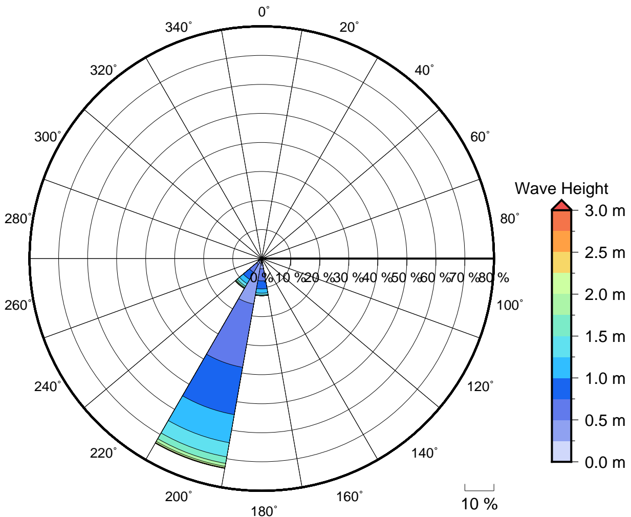
Figure 2 Annual wave rose for Somosomo Bay. Note that direction are where the wave are coming from .
