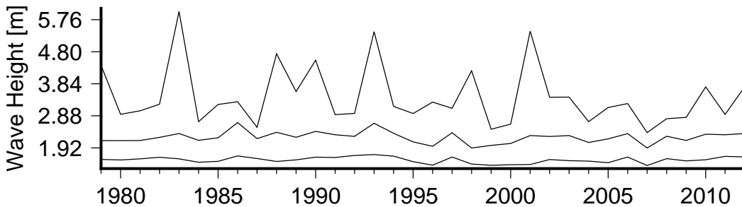
Figure 8 Annual variation in large waves (90th percentile)(lower curve), severe waves (99th percentile) (middle curve) and the largest wave(upper curve) in Somosomo Bay.
