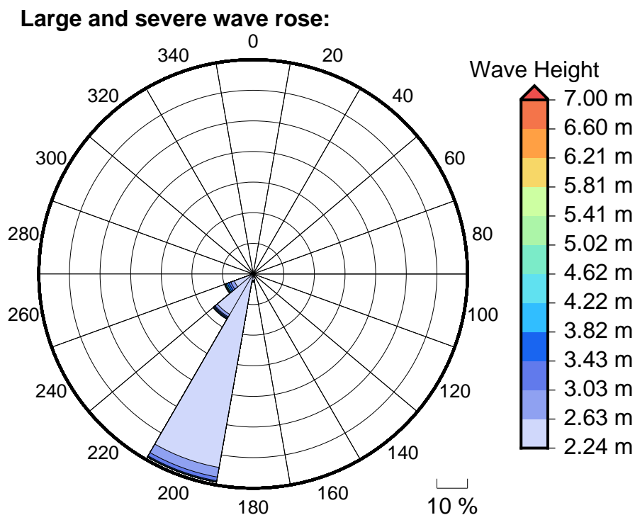
Figure 6 Large, severe and extreme wave roses for Somosomo Bay
