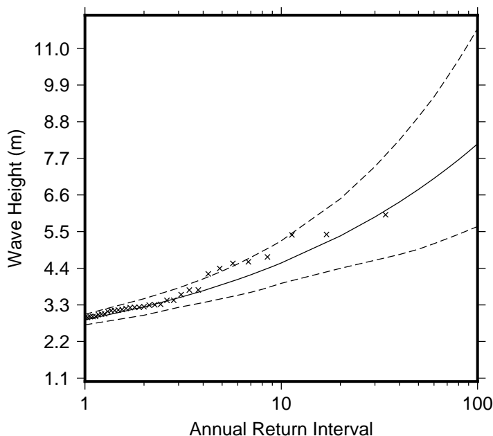
Figure 9 Extreme wave distribution for Somosomo Bay. The crosses represents the wave events that occurred since 1979. The plain line is the statistical distribution that best fit the past wave events. The dotted line show the upper and lower high confidence of the fit, there is a 95% chance that the fitted distribution lie between the two dashed lines.
