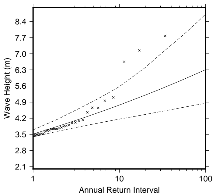
Figure 9 Extreme wave distribution for Sigatoka River Mouth. The crosses represents the wave events that occurred since 1979. The plain line is the statistical distribution that best fit the past wave events. The dotted line show the upper and lower high confidence of the fit, there is a 95% chance that the fitted distribution lie between the two dashed lines.
