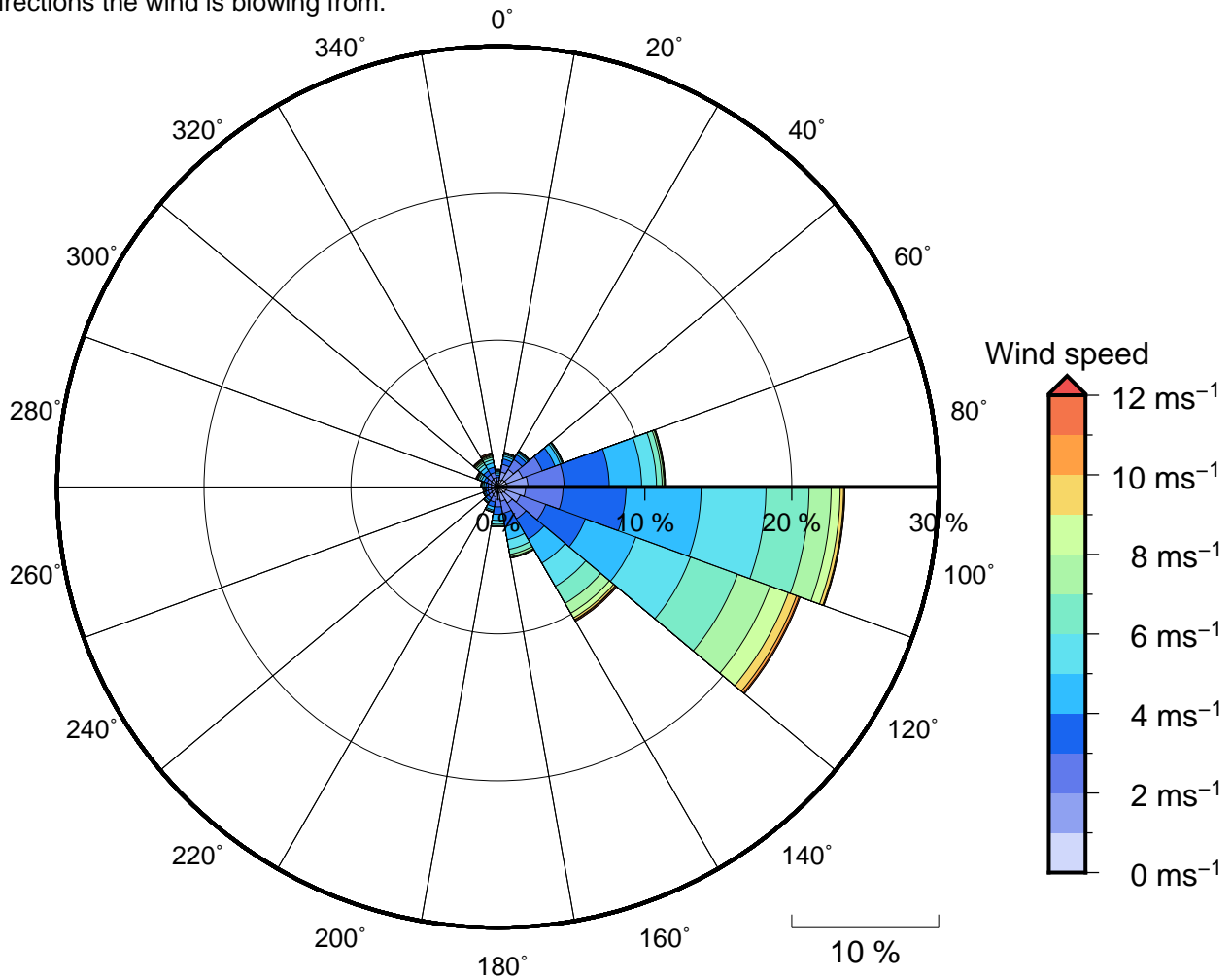
Figure 11 Annual wind rose for Sigatoka River Mouth. Note that directions are where the wind is coming from.
