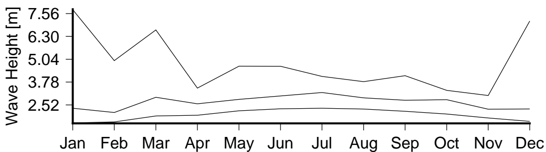
Figure 7 Monthly variation in large waves (90th percentile)(lower curve), severe waves (99th percentile) (middle curve) and the largest wave(upper curve) in Sigatoka River Mouth.
