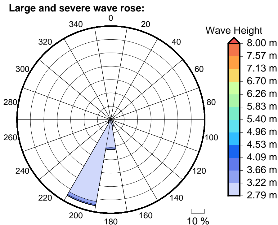
Figure 6 Large, severe and extreme wave roses for Sigatoka River Mouth
