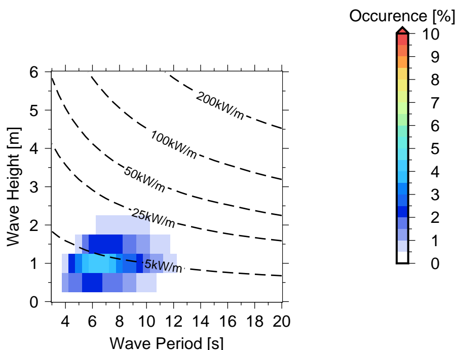
Figure 10 Occurences of sea states in Sigatoka River Mouth .
