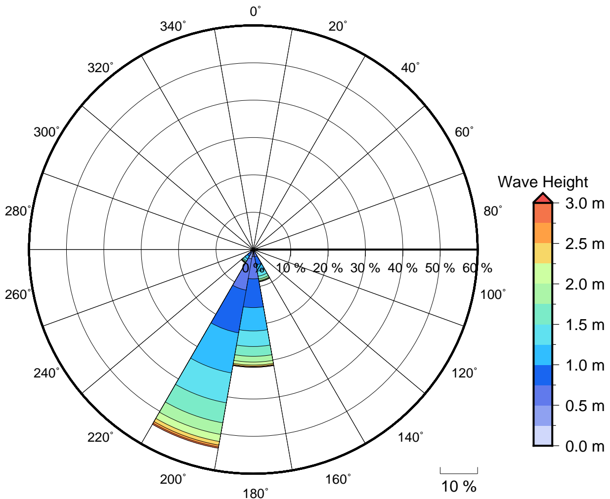
Figure 2 Annual wave rose for Sigatoka River Mouth. Note that direction are where the wave are coming from.
