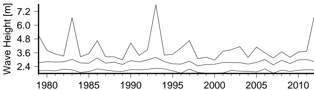
Figure 8 Annual variation in large waves (90th percentile)(lower curve), severe waves (99th percentile) (middle curve) and the largest wave(upper curve) in Sigatoka River Mouth.
