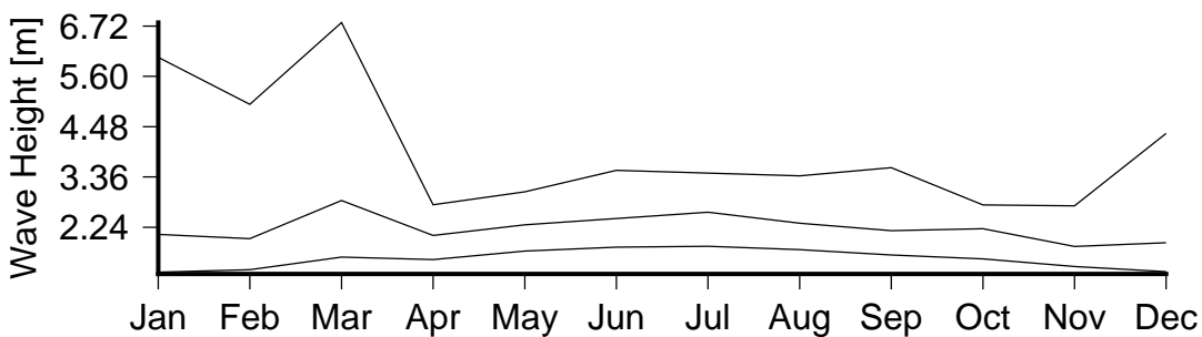
Figure 7 Monthly variation in large waves (90th percentile)(lower curve), severe waves (99th percentile) (middle curve) and the largest wave(upper curve) in Shifties Reef.
