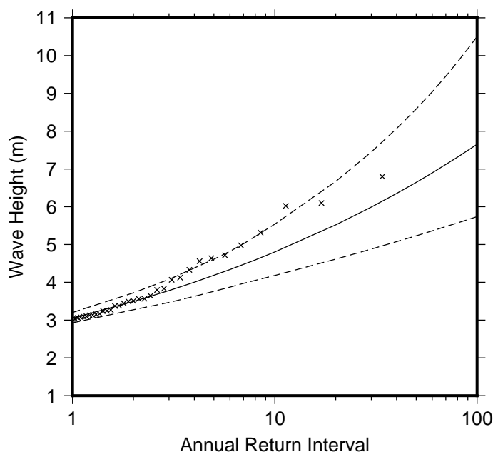
Figure 9 Extreme wave distribution for Shifties Reef. The crosses represents the wave events that occurred since 1979. The plain line is the statistical distribution that best fit the past wave events. The dotted line show the upper and lower high confidence of the fit, there is a 95% chance that the fitted distribution lie between the two dashed lines.
