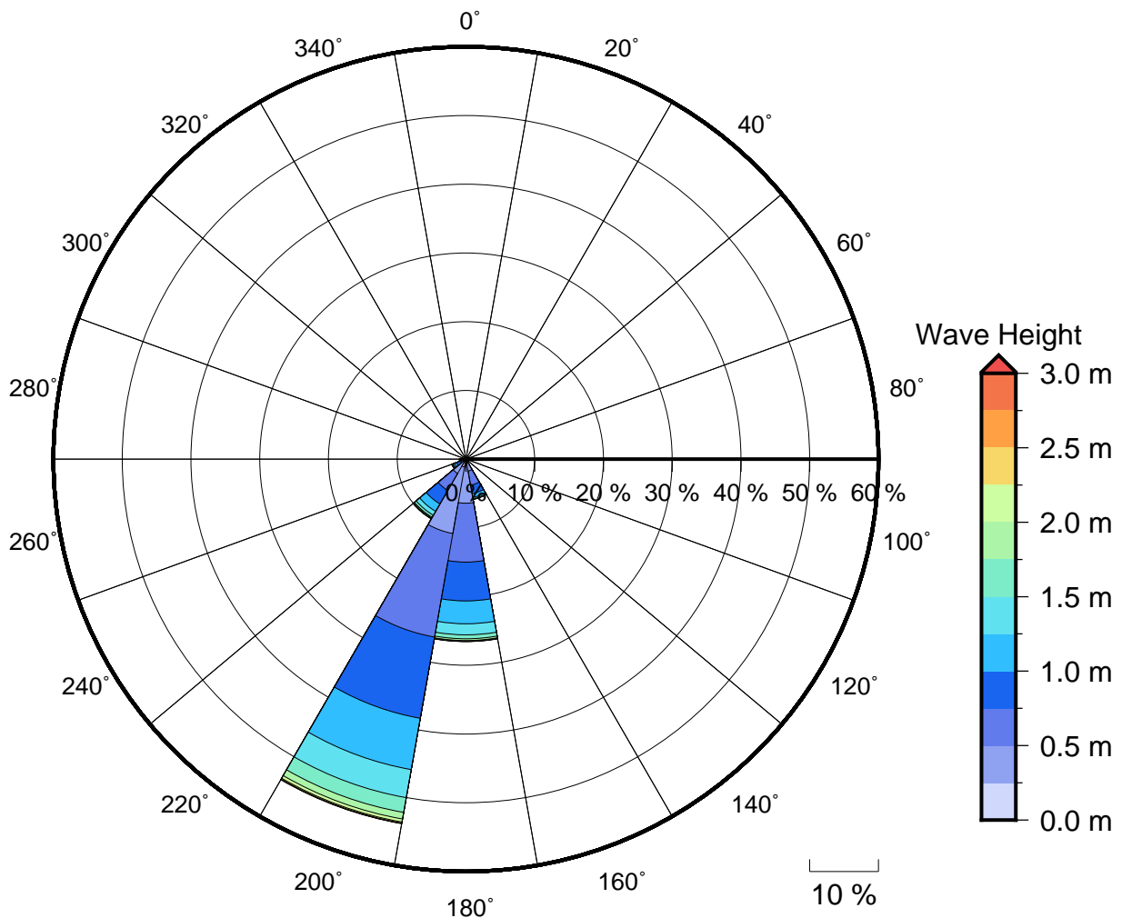
Figure 2 Annual wave rose for Shifties Reef. Note that direction are where the wave are coming from .
