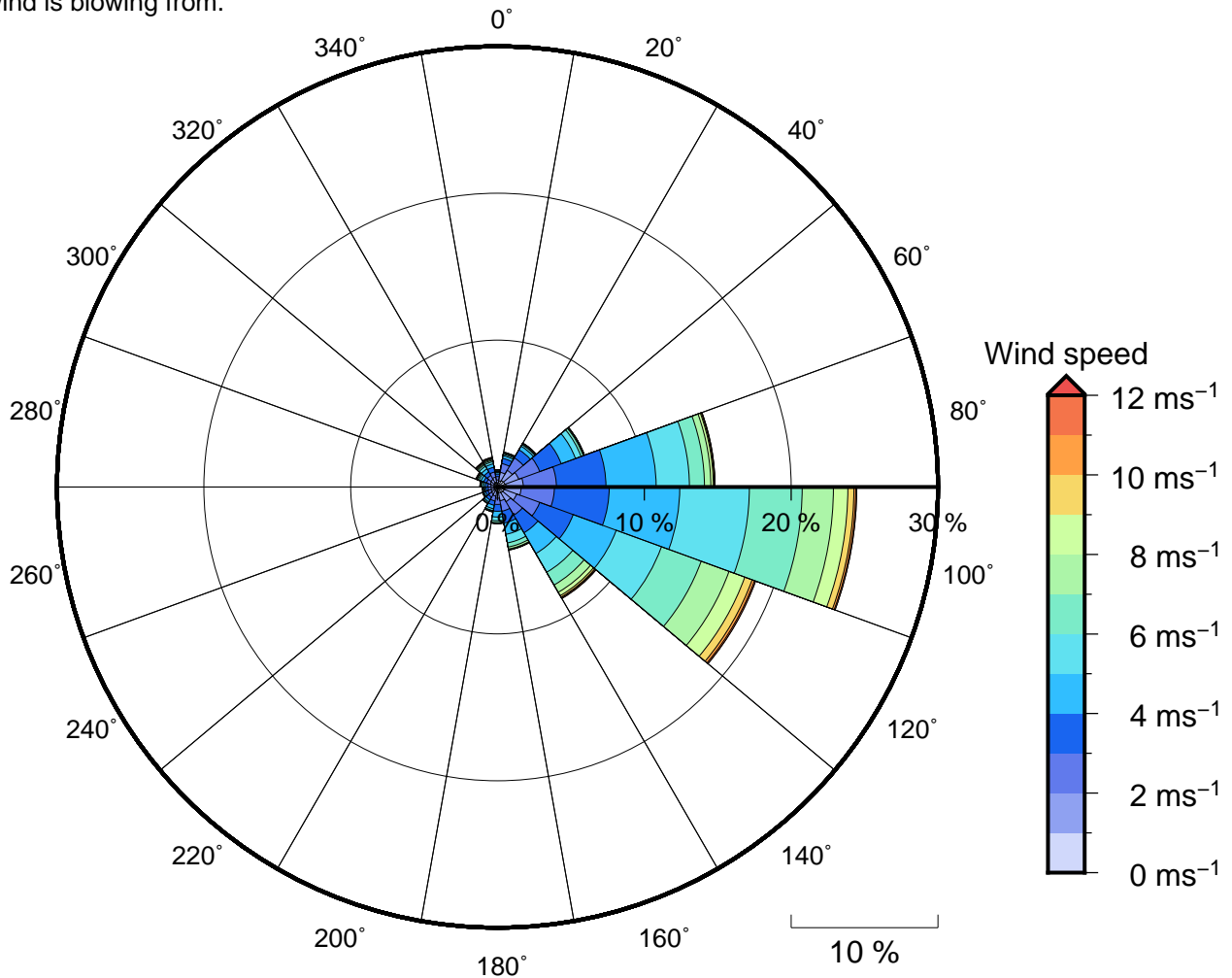
Figure 11 Annual wind rose for Shifties Reef. Note that directions are where the wind is coming from.
