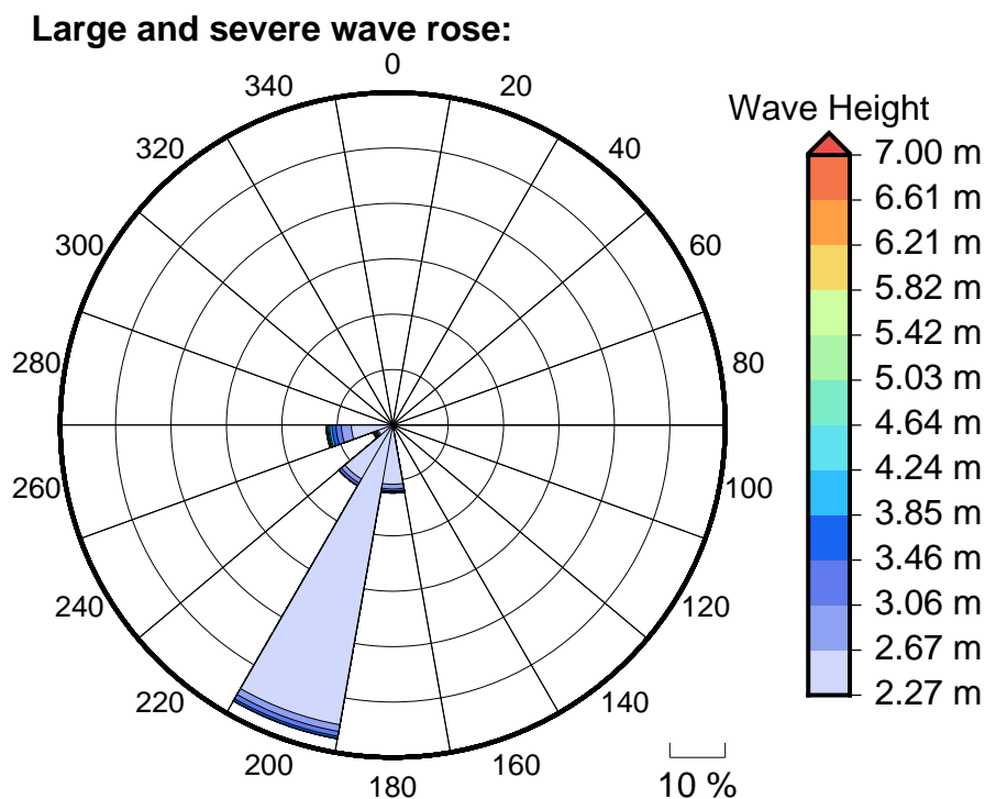
Figure 6 Large, severe and extreme wave roses for Shifties Reef
