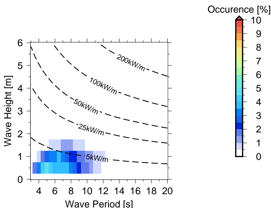
Figure 10 Occurrences of sea states in Shifties Reef .
