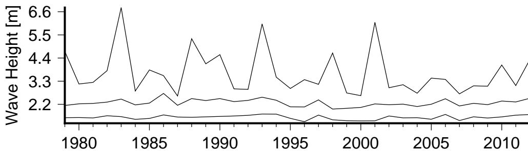
Figure 8 Annual variation in large waves (90th percentile)(lower curve), severe waves (99th percentile) (middle curve) and the largest wave(upper curve) in Shifties Reef.
