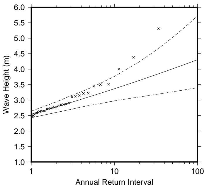
Figure 9 Extreme wave distribution for Rewa River Mouth. The crosses represents the wave events that occurred since 1979. The plain line is the statistical distribution that best fit the past wave events. The dotted line show the upper and lower high confidence of the fit, there is a 95% chance that the fitted distribution lie between the two dashed lines.
