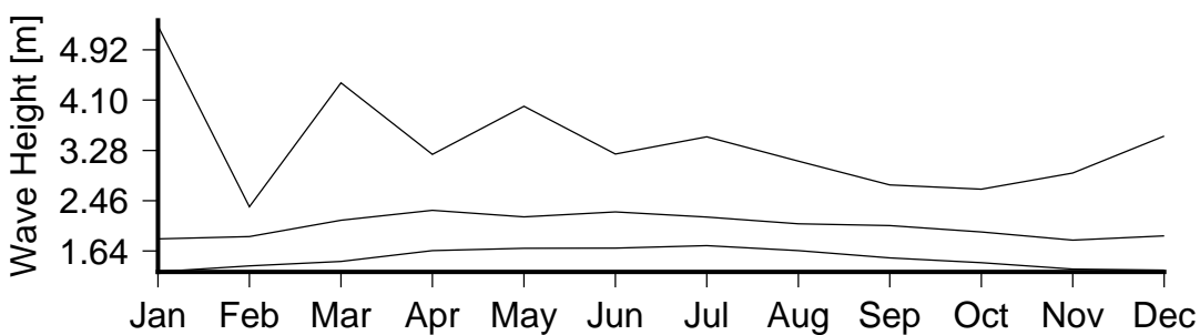
Figure 7 Monthly variation in large waves (90th percentile)(lower curve), severe waves (99th percentile) (middle curve) and the largest wave(upper curve) in Rewa River Mouth.
