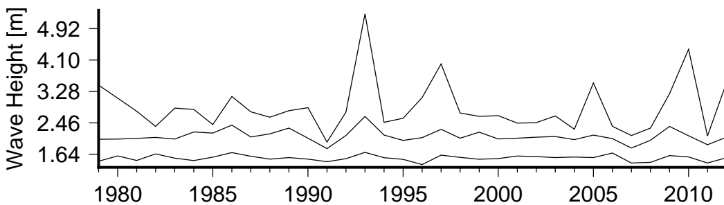
Figure 8 Annual variation in large waves (90th percentile)(lower curve), severe waves (99th percentile) (middle curve) and the largest wave(upper curve) in Rewa River Mouth.
