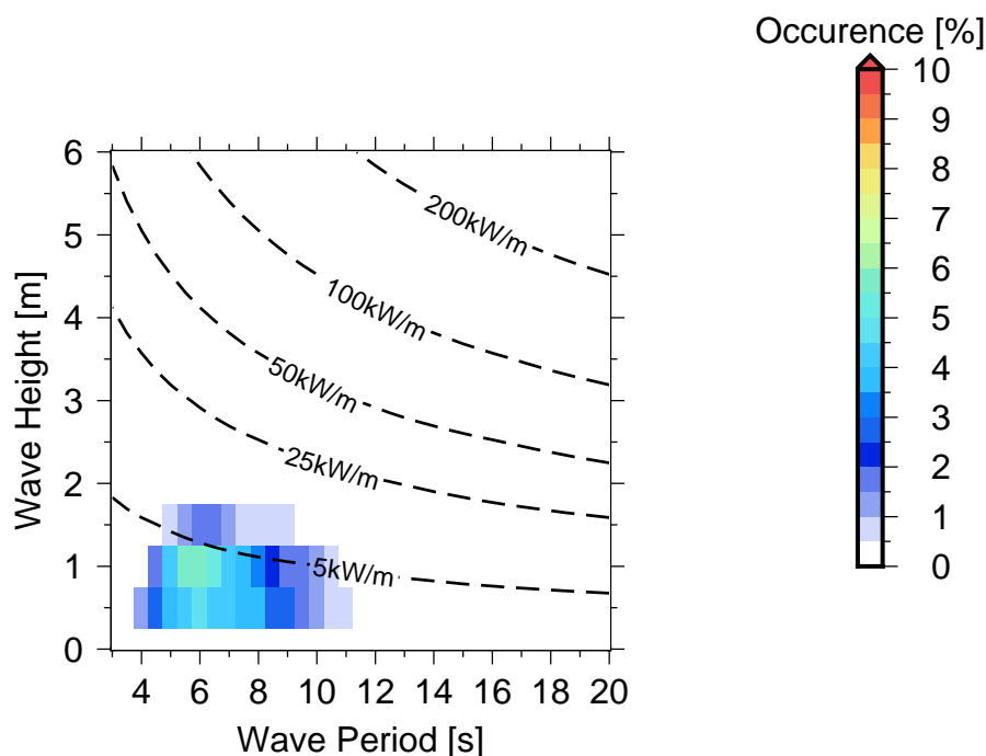
Figure 10 Occurrences of sea states in Rewa River Mouth .
