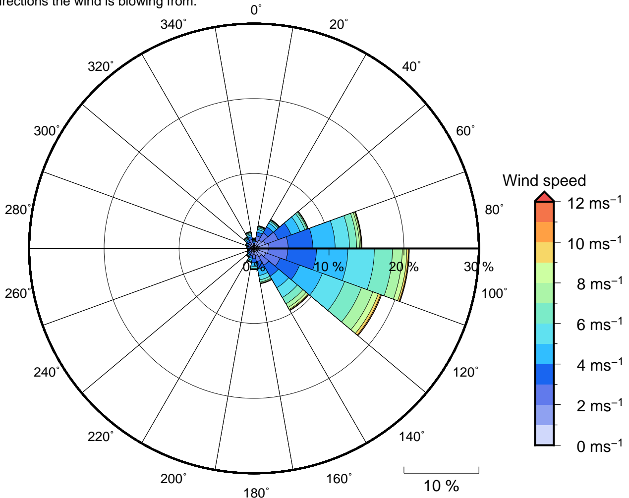
Figure 11 Annual wind rose for Rewa River Mouth. Note that directions are where the wind is coming from.
