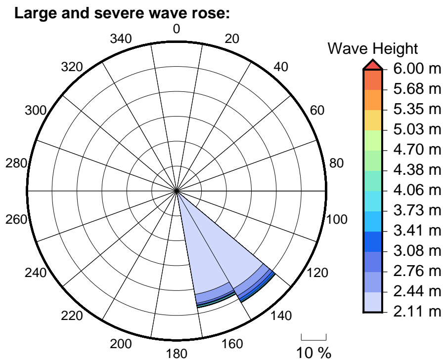
Figure 6 Large, severe and extreme wave roses for Rewa River Mouth
