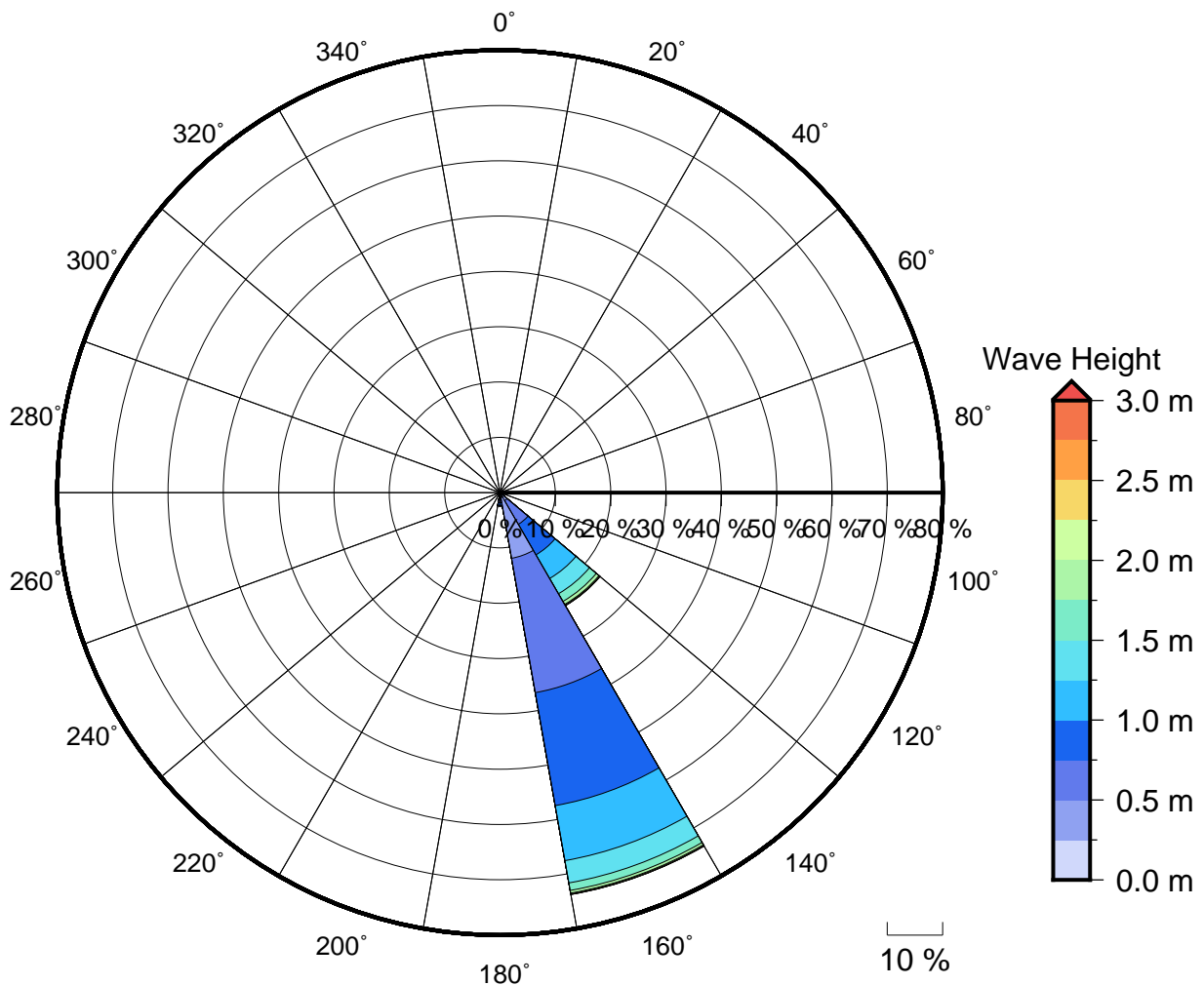
Figure 2 Annual wave rose for Rewa River Mouth. Note that direction are where the wave are coming from.
