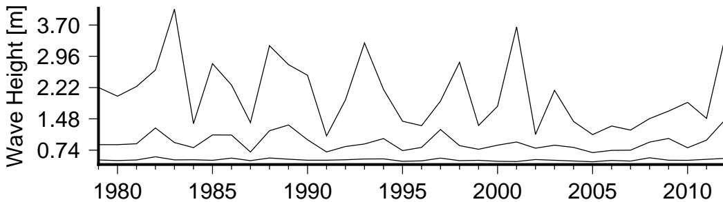
Figure 8 Annual variation in large waves (90th percentile)(lower curve), severe waves (99th percentile) (middle curve) and the largest wave(upper curve) in Raviravi.
