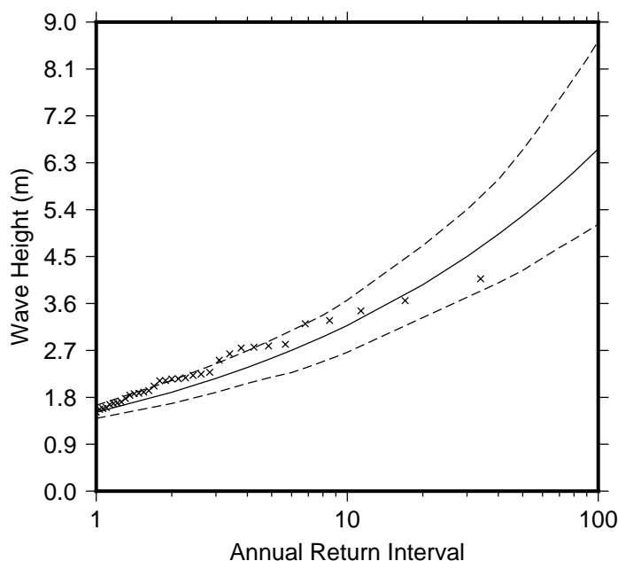
Figure 9 Extreme wave distribution for Raviravi. The crosses represents the wave events that occurred since 1979. The plain line is the statistical distribution that best fit the past wave events. The dotted line show the upper and lower high confidence of the fit, there is a 95% chance that the fitted distribution lie between the two dashed lines.
