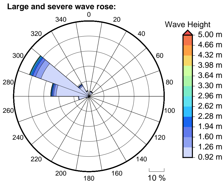
Figure 6 Large, severe and extreme wave roses for Raviravi
