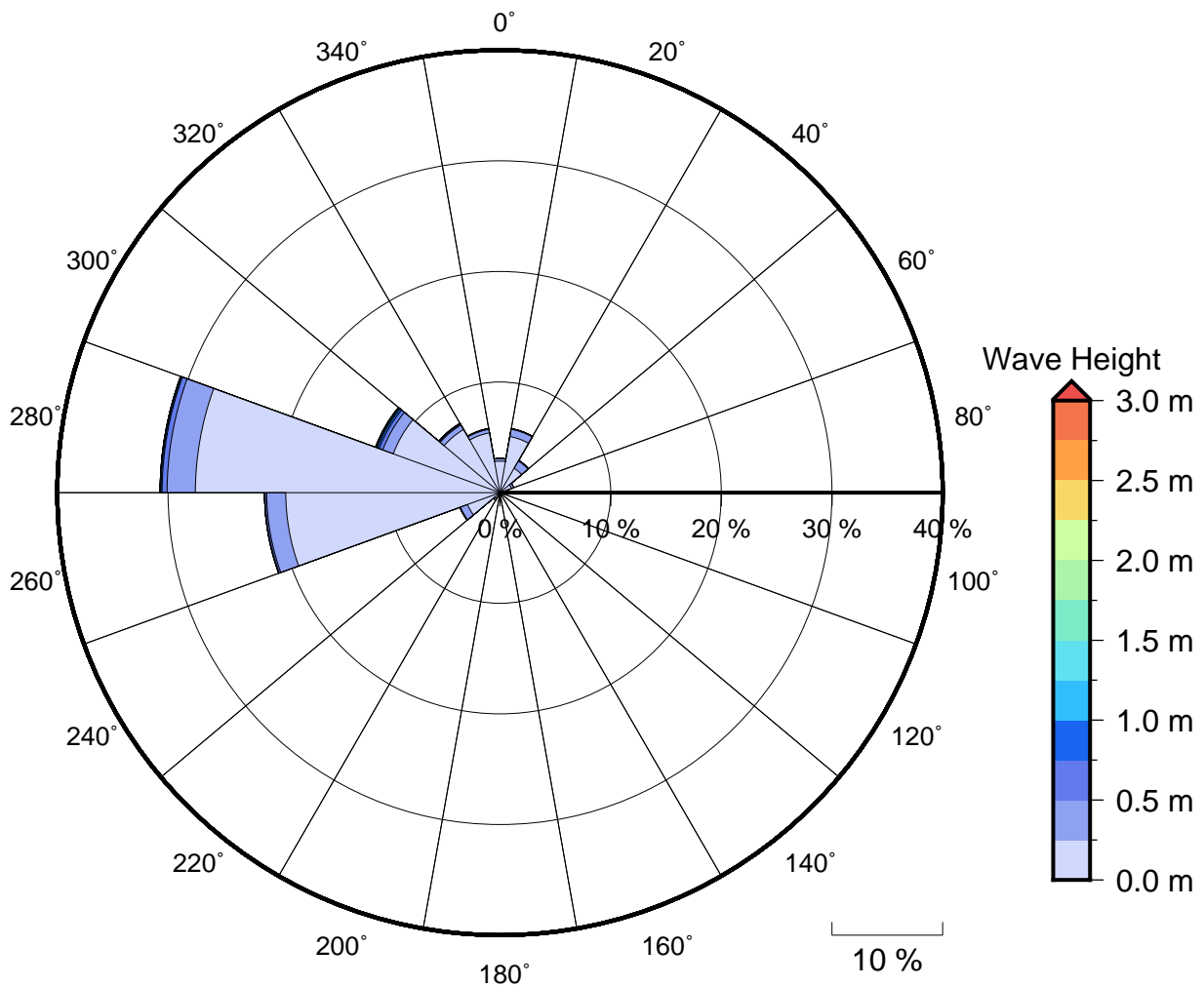
Figure 2 Annual wave rose for Raviravi. Note that direction are where the wave are coming from.
