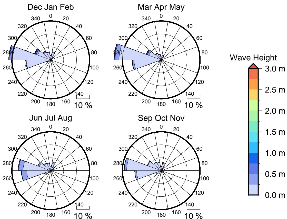
Figure 3 Seasonal wave roses for Raviravi
