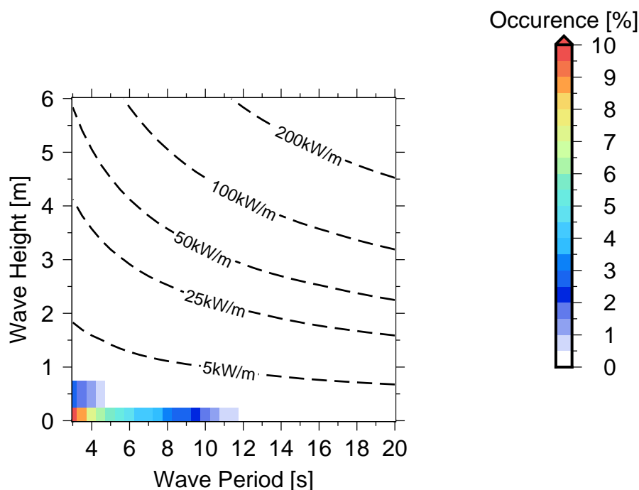
Figure 10 Occurrences of sea states in Raviravi .
