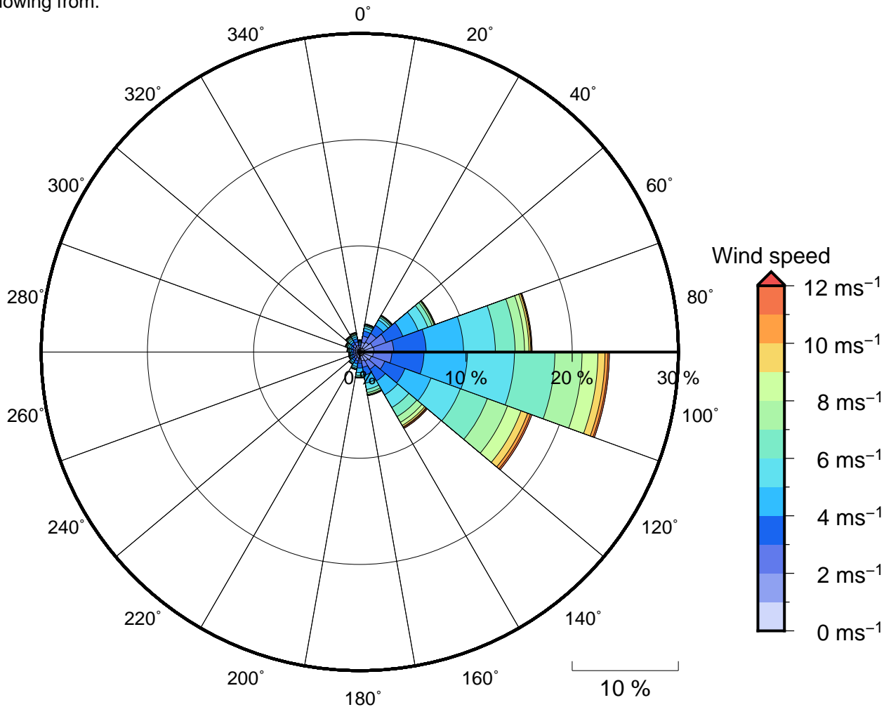
Figure 11 Annual wind rose for Raviravi. Note that directions are where the wind is coming from.
