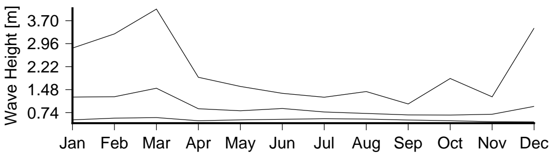
Figure 7 Monthly variation in large waves (90th percentile)(lower curve), severe waves (99th percentile) (middle curve) and the largest wave(upper curve) in Raviravi.
