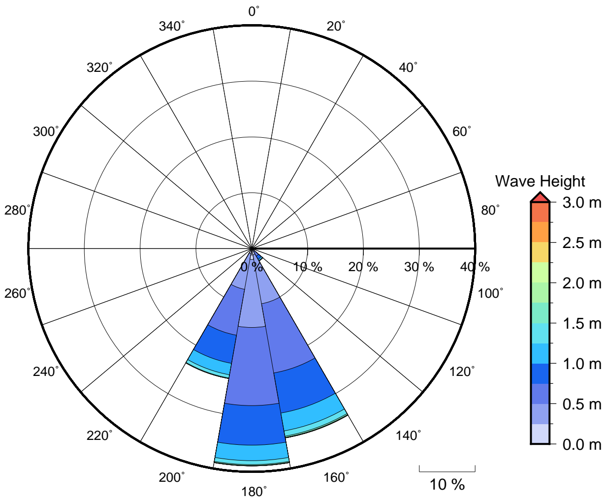
Figure 2 Annual wave rose for Rats Tail Passage. Note that direction are where the wave are coming from.
