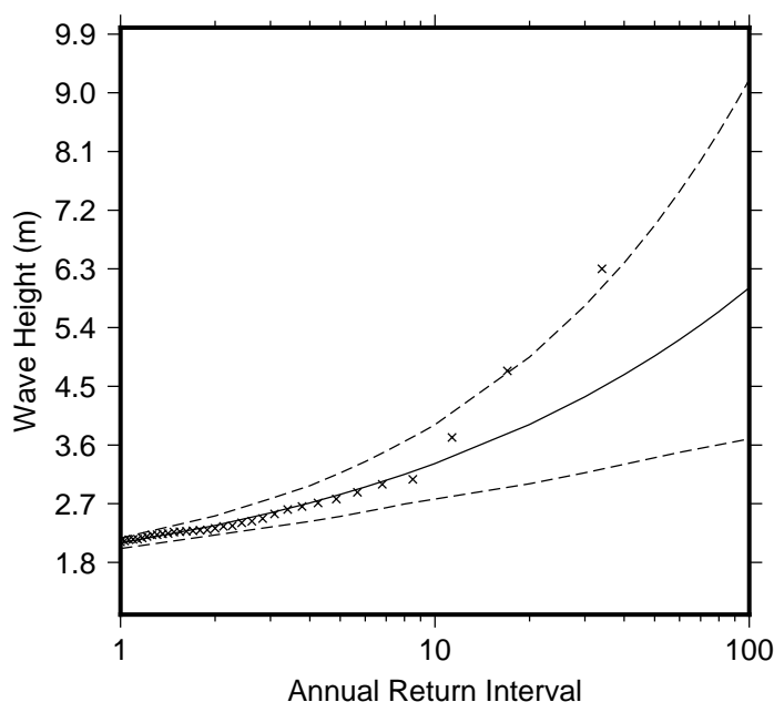
Figure 9 Extreme wave distribution for Rats Tail Passage. The crosses represents the wave events that occurred since 1979. The plain line is the statistical distribution that best fit the past wave events. The dotted line show the upper and lower high confidence of the fit, there is a 95% chance that the fitted distribution lie between the two dashed lines.
