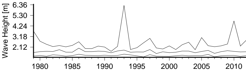
Figure 8 Annual variation in large waves (90th percentile)(lower curve), severe waves (99th percentile) (middle curve) and the largest wave(upper curve) in Rats Tail Passage.
