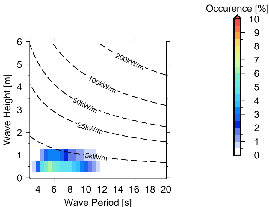
Figure 10 Occurrences of sea states in Rats Tail Passage .
