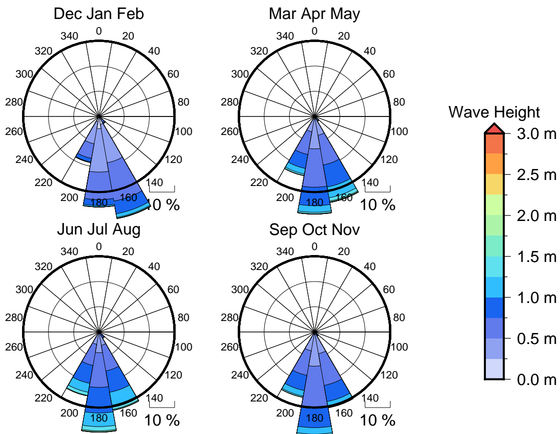
Figure 3 Seasonal wave roses for Rats Tail Passage
