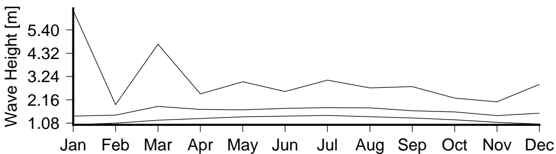
Figure 7 Monthly variation in large waves (90th percentile)(lower curve), severe waves (99th percentile) (middle curve) and the largest wave(upper curve) in Rats Tail Passage.
