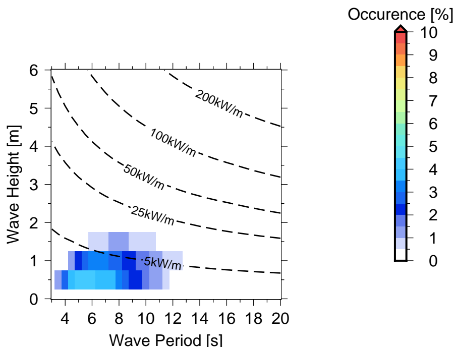
Figure 10 Occurrences of sea states in Pipeline Reef .
