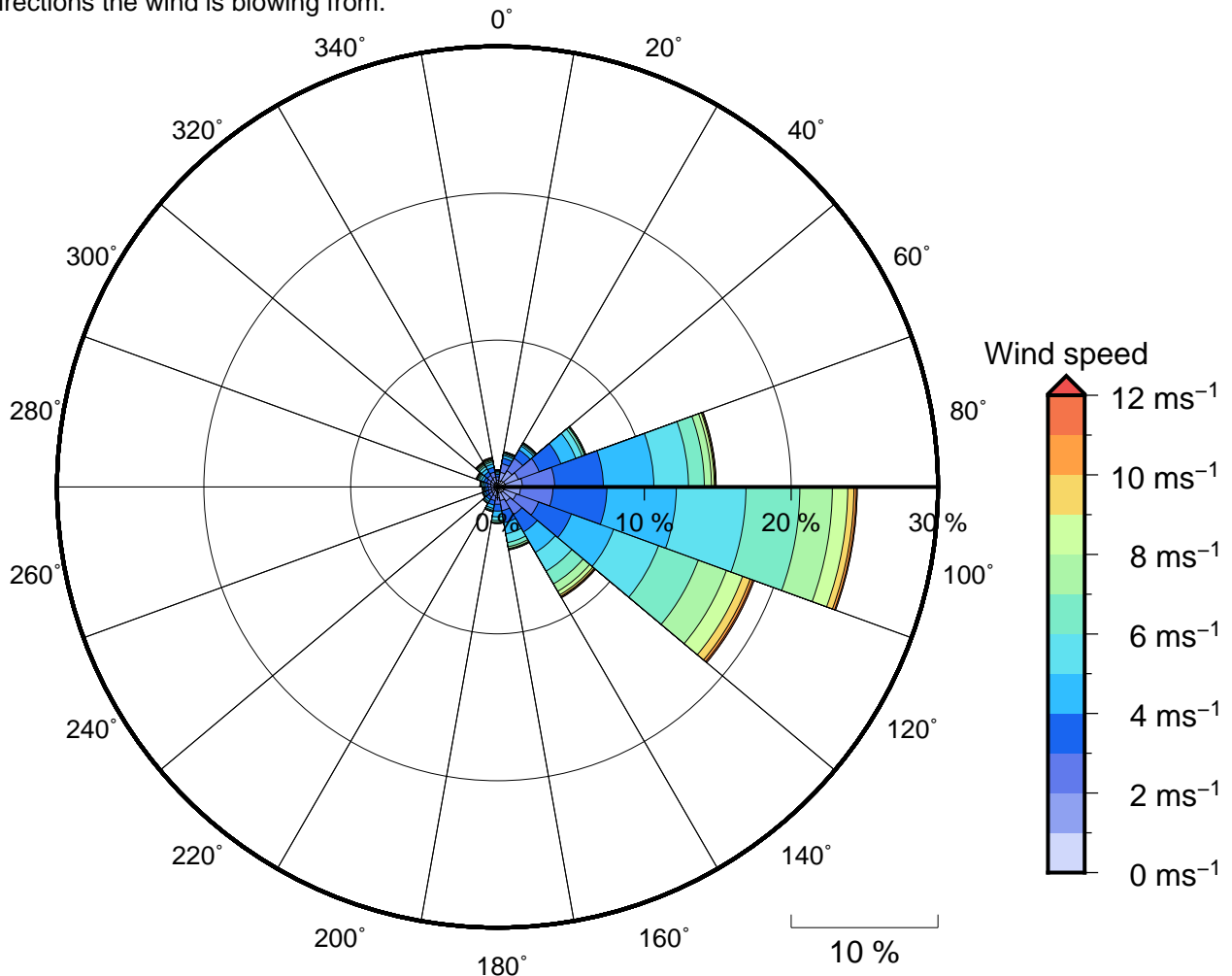
Figure 11 Annual wind rose for Pipeline Reef. Note that directions are where the wind is coming from.
