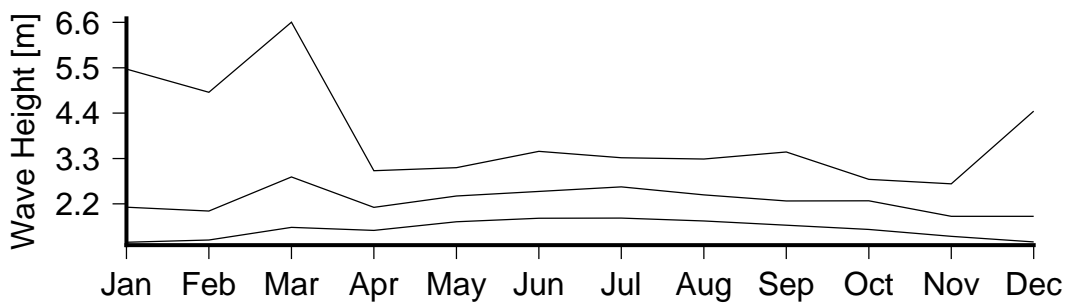
Figure 7 Monthly variation in large waves (90th percentile)(lower curve), severe waves (99th percentile) (middle curve) and the largest wave(upper curve) in Pipeline Reef.
