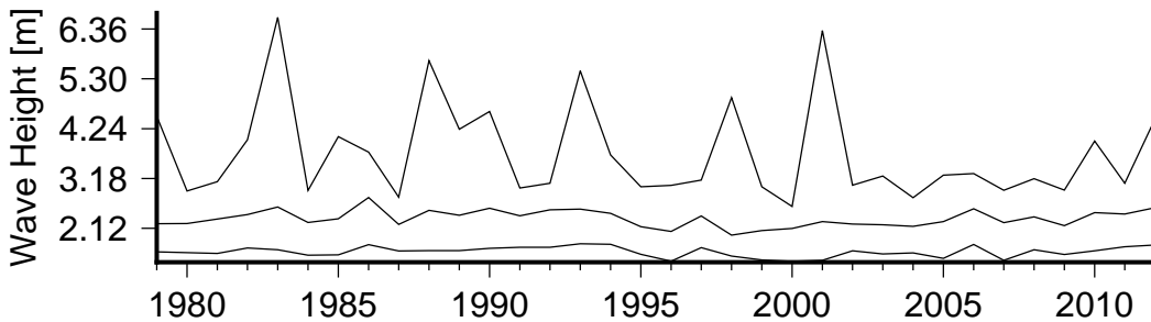
Figure 8 Annual variation in large waves (90th percentile)(lower curve), severe waves (99th percentile) (middle curve) and the largest wave(upper curve) in Pipeline Reef.
