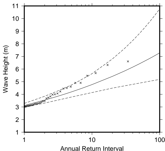
Figure 9 Extreme wave distribution for Pipeline Reef. The crosses represents the wave events that occurred since 1979. The plain line is the statistical distribution that best fit the past wave events. The dotted line show the upper and lower high confidence of the fit, there is a 95% chance that the fitted distribution lie between the two dashed lines.
