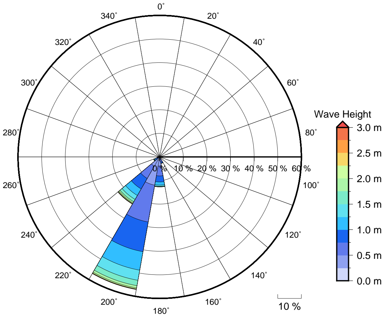
Figure 2 Annual wave rose for Pipeline Reef. Note that direction are where the wave are coming from .
