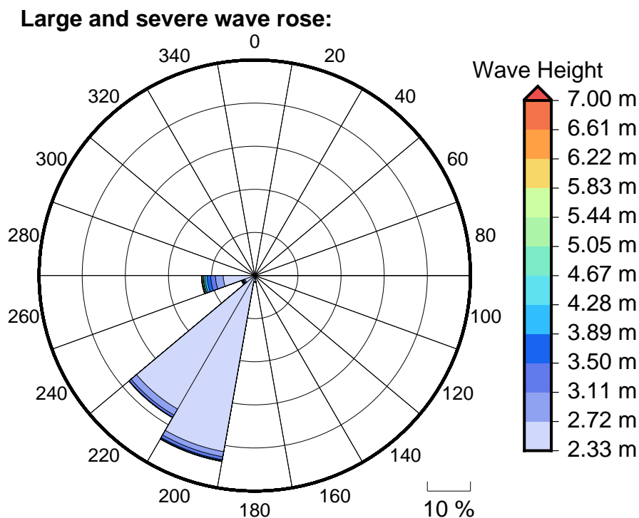
Figure 6 Large, severe and extreme wave roses for Pipeline Reef
