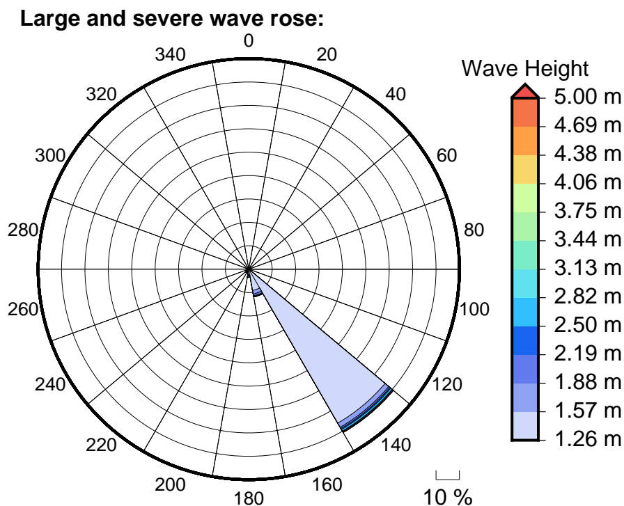
Figure 6 Large, severe and extreme wave roses for Pacific Harbour
