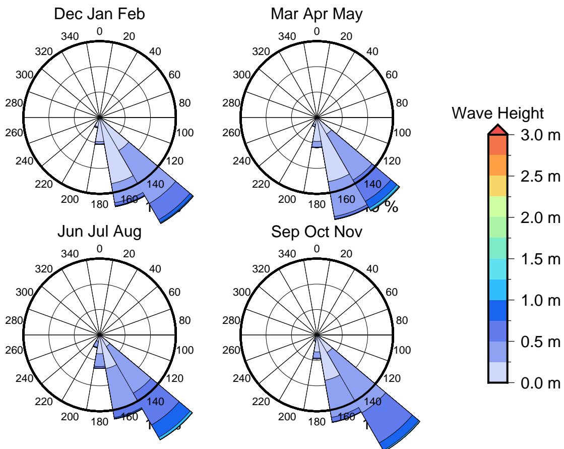
Figure 3 Seasonal wave roses for Pacific Harbour
