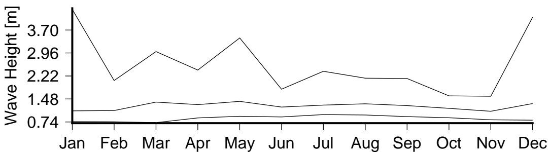
Figure 7 Monthly variation in large waves (90th percentile)(lower curve), severe waves (99th percentile) (middle curve) and the largest wave(upper curve) in Pacific Harbour.
