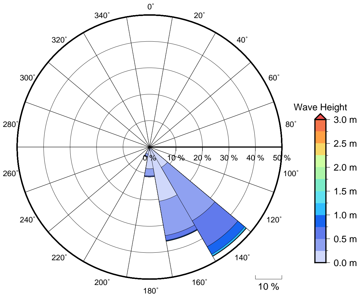
Figure 2 Annual wave rose for Pacific Harbour. Note that direction are where the wave are coming from .
