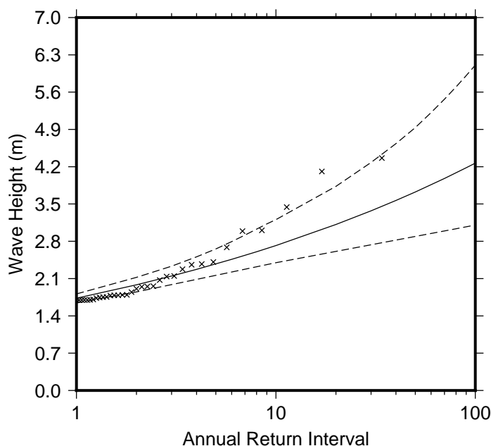
Figure 9 Extreme wave distribution for Pacific Harbour. The crosses represents the wave events that occurred since 1979. The plain line is the statistical distribution that best fit the past wave events. The dotted line show the upper and lower high confidence of the fit, there is a 95% chance that the fitted distribution lie between the two dashed lines.
