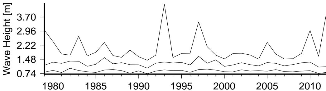
Figure 8 Annual variation in large waves (90th percentile)(lower curve), severe waves (99th percentile) (middle curve) and the largest wave(upper curve) in Pacific Harbour.
