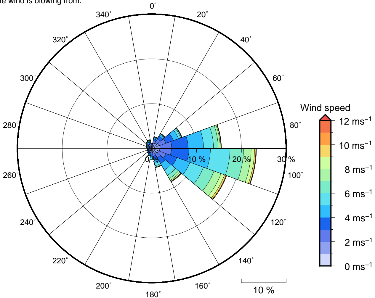
Figure 11 Annual wind rose for Pacific Harbour. Note that directions are where the wind is coming from.
