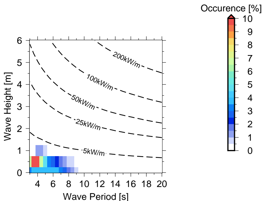
Figure 10 Occurrences of sea states in Pacific Harbour .
