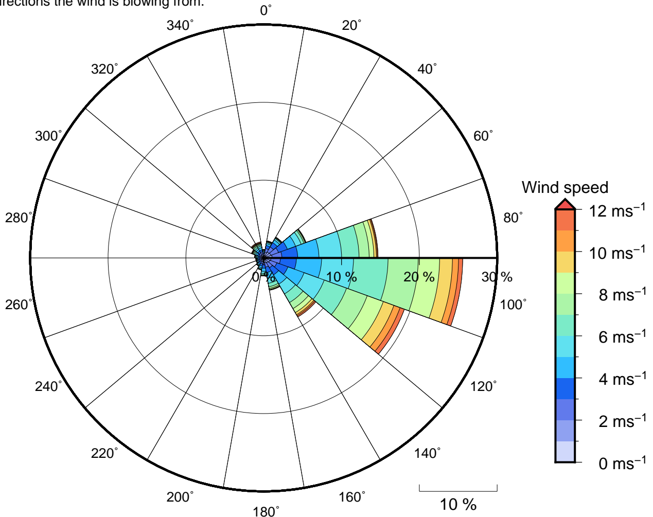
Figure 11 Annual wind rose for North Vatulele. Note that directions are where the wind is coming from.
