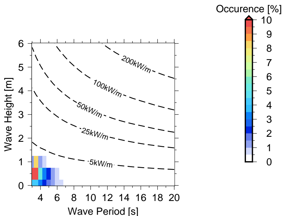
Figure 10 Occurrences of sea states in North Vatulele .
