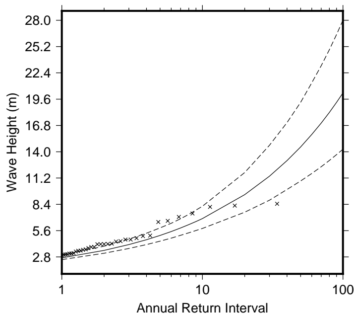
Figure 9 Extreme wave distribution for North Vatulele. The crosses represents the wave events that occurred since 1979. The plain line is the statistical distribution that best fit the past wave events. The dotted line show the upper and lower high confidence of the fit, there is a 95% chance that the fitted distribution lie between the two dashed lines.
