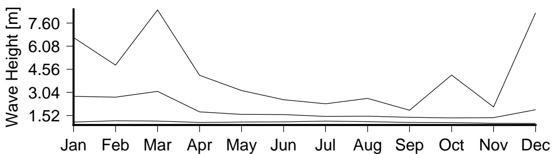
Figure 7 Monthly variation in large waves (90th percentile)(lower curve), severe waves (99th percentile) (middle curve) and the largest wave(upper curve) in North Vatulele.
