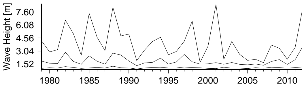
Figure 8 Annual variation in large waves (90th percentile)(lower curve), severe waves (99th percentile) (middle curve) and the largest wave(upper curve) in North Vatulele.
