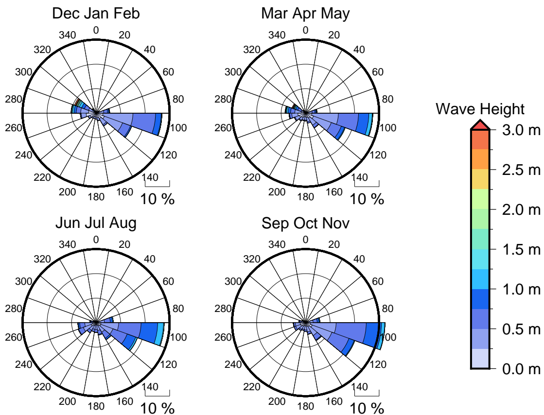
Figure 3 Seasonal wave roses for North Vatulele
