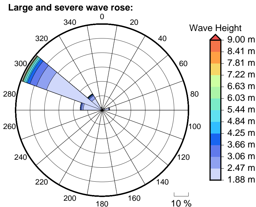
Figure 6 Large, severe and extreme wave roses for North Vatulele
