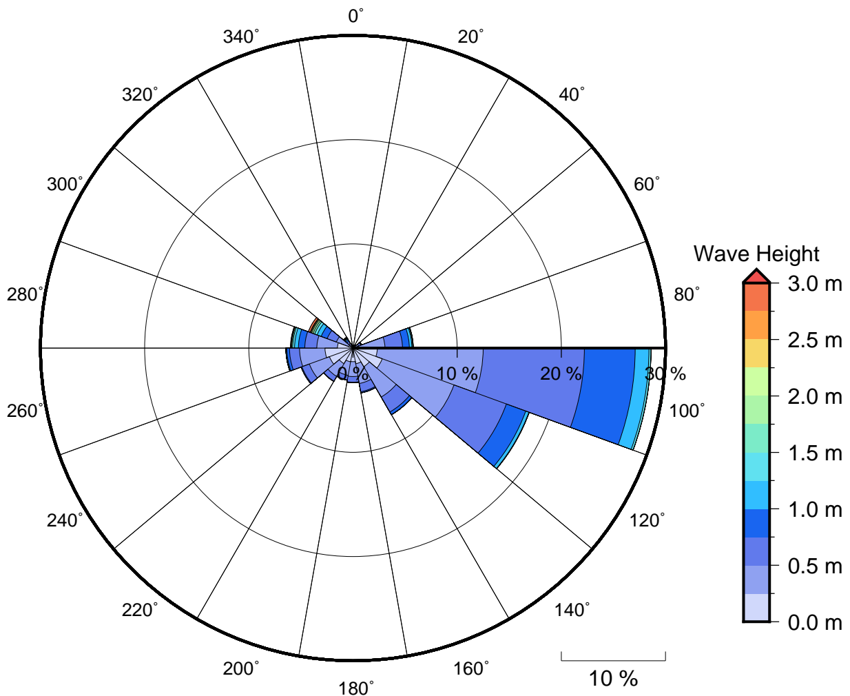
Figure 2 Annual wave rose for North Vatulele. Note that direction are where the wave are coming from .
