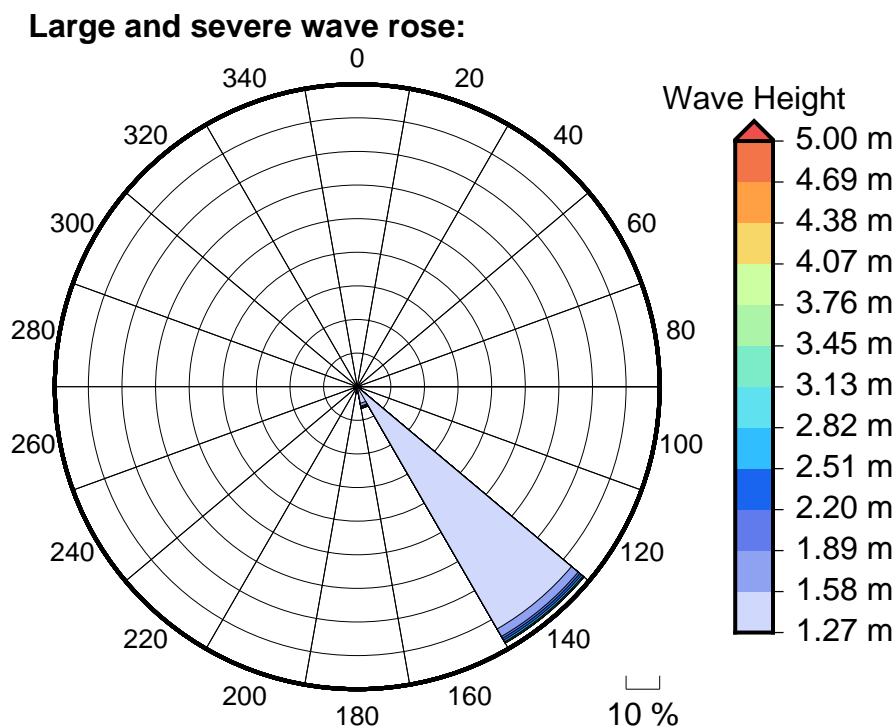
Figure 6 Large, severe and extreme wave roses for Navua River Mouth
