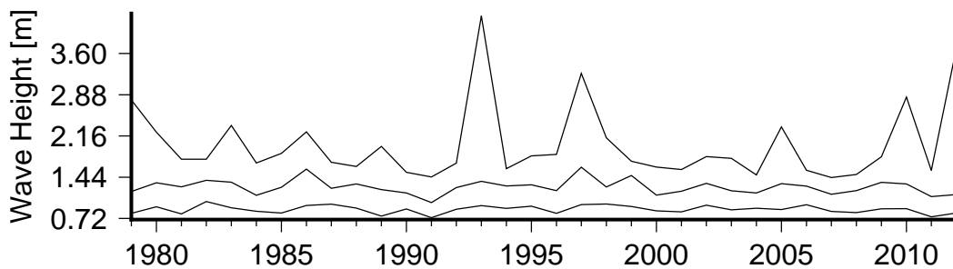
Figure 8 Annual variation in large waves (90th percentile)(lower curve), severe waves (99th percentile) (middle curve) and the largest wave(upper curve) in Navua River Mouth.
