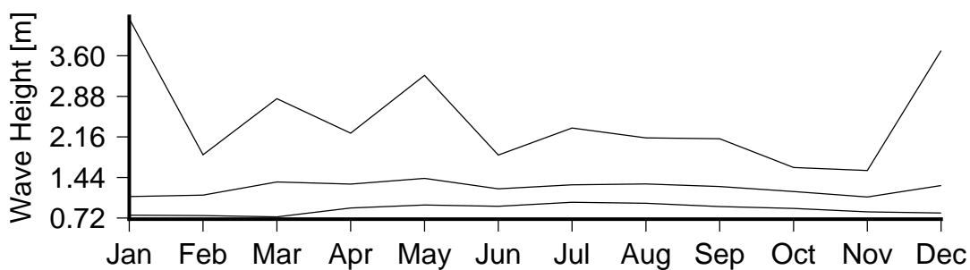
Figure 7 Monthly variation in large waves (90th percentile)(lower curve), severe waves (99th percentile) (middle curve) and the largest wave(upper curve) in Navua River Mouth.
