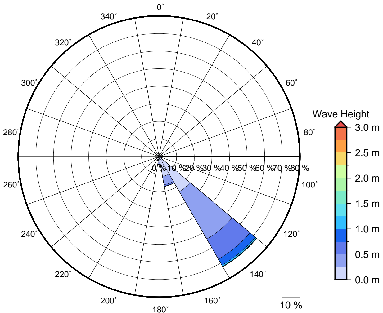
Figure 2 Annual wave rose for Navua River Mouth. Note that direction are where the wave are coming from.
