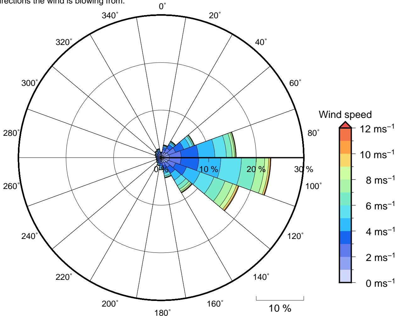
Figure 11 Annual wind rose for Navua River Mouth. Note that directions are where the wind is coming from.
