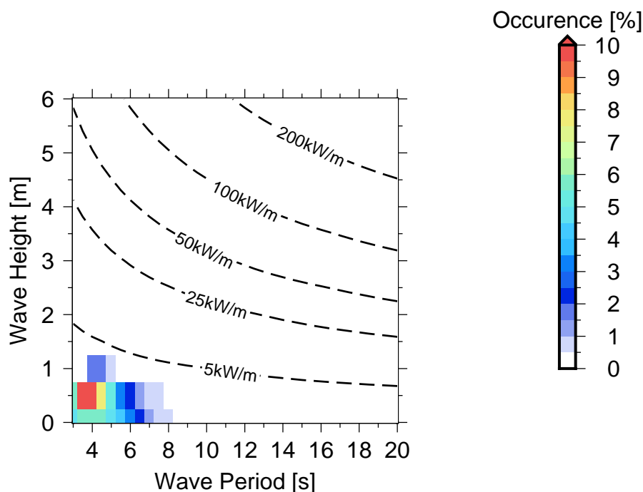
Figure 10 Occurrences of sea states in Navua River Mouth .
