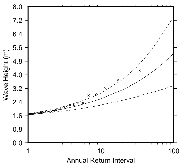
Figure 9 Extreme wave distribution for Navua River Mouth. The crosses represents the wave events that occurred since 1979. The plain line is the statistical distribution that best fit the past wave events. The dotted line show the upper and lower high confidence of the fit, there is a 95% chance that the fitted distribution lie between the two dashed lines.
