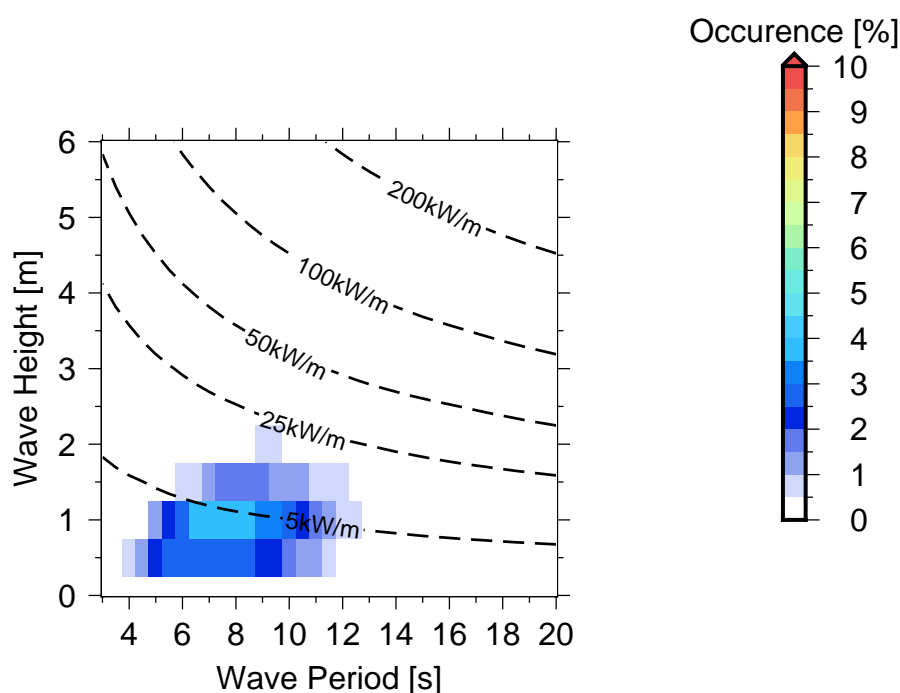
Figure 10 Occurences of sea states in Naviti Resort .
