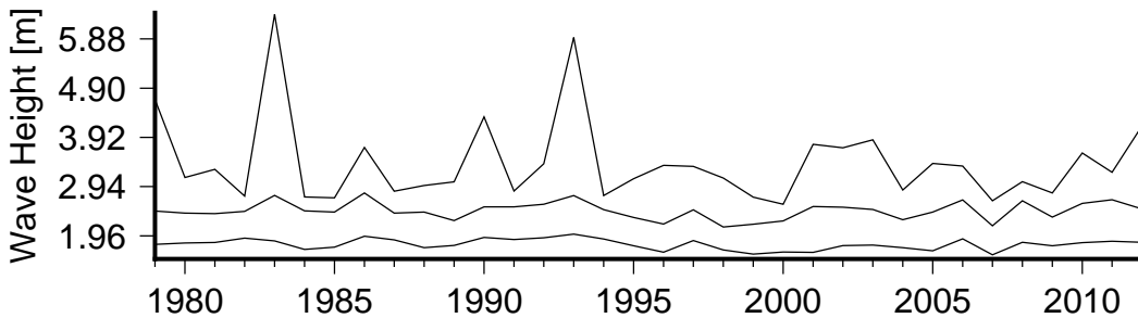
Figure 8 Annual variation in large waves (90th percentile)(lower curve), severe waves (99th percentile) (middle curve) and the largest wave(upper curve) in Naviti Resort.
