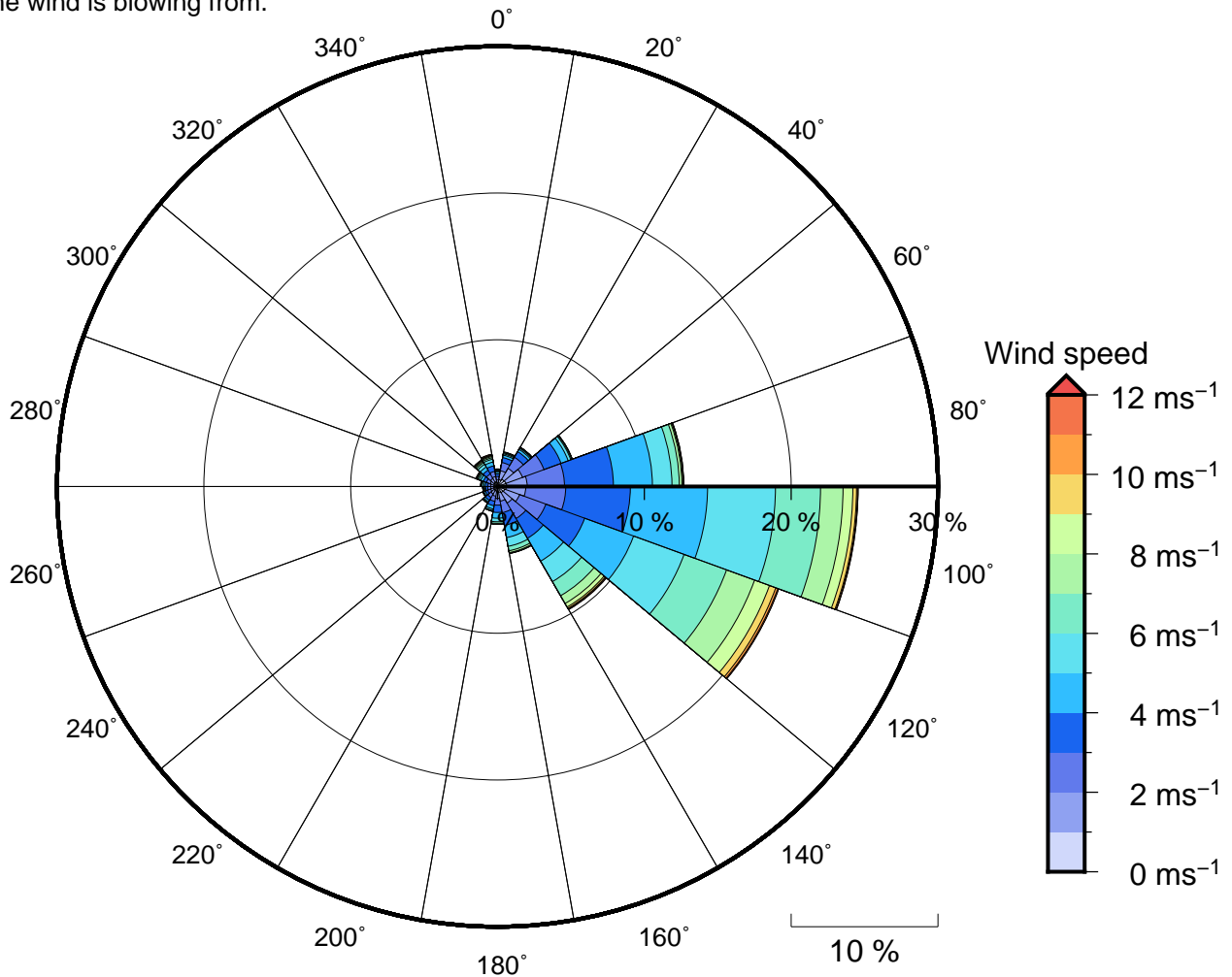
Figure 11 Annual wind rose for Naviti Resort. Note that directions are where the wind is coming from.
