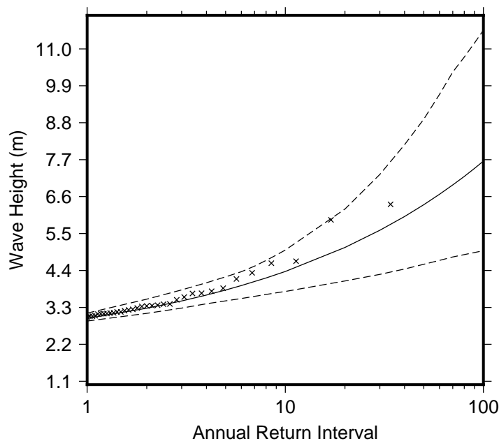
Figure 9 Extreme wave distribution for Naviti Resort. The crosses represents the wave events that occurred since 1979. The plain line is the statistical distribution that best fit the past wave events. The dotted line show the upper and lower high confidence of the fit, there is a 95% chance that the fitted distribution lie between the two dashed lines.
