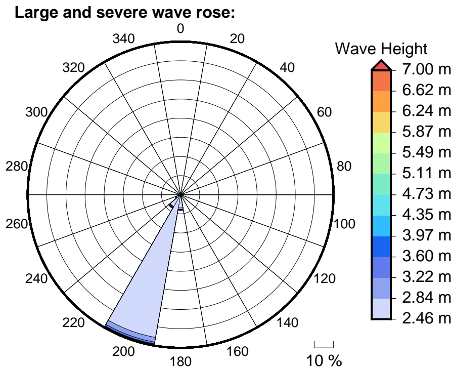
Figure 6 Large, severe and extreme wave roses for Naviti Resort
