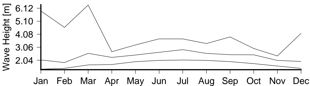
Figure 7 Monthly variation in large waves (90th percentile)(lower curve), severe waves (99th percentile) (middle curve) and the largest wave(upper curve) in Naviti Resort.
