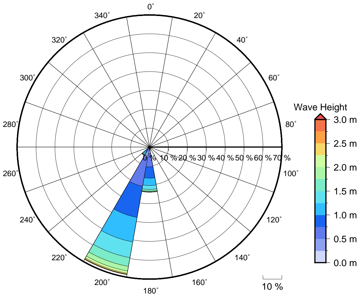
Figure 2 Annual wave rose for Naviti Resort. Note that direction are where the wave are coming from .
