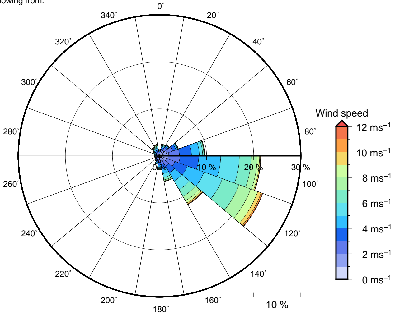
Figure 11 Annual wind rose for Natadola. Note that directions are where the wind is coming from.
