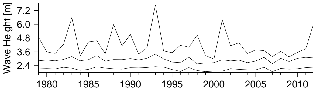
Figure 8 Annual variation in large waves (90th percentile)(lower curve), severe waves (99th percentile) (middle curve) and the largest wave(upper curve) in Natadola.
