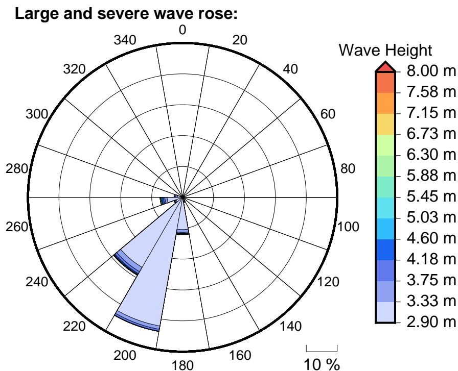
Figure 6 Large, severe and extreme wave roses for Natadola
