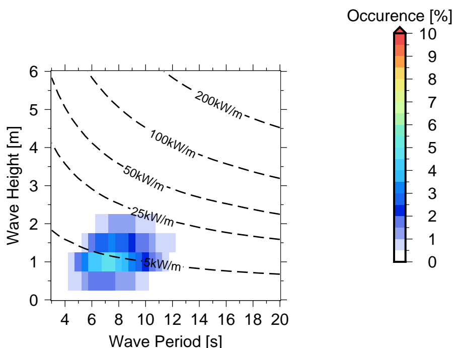
Figure 10 Occurrences of sea states in Natadola .
