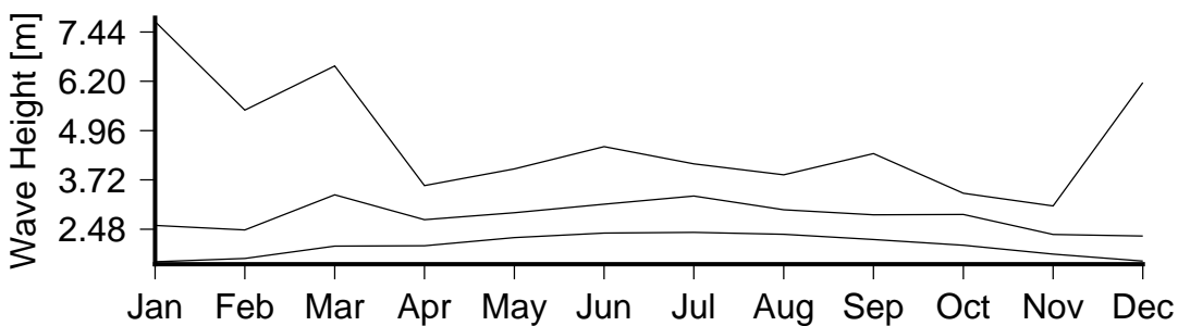
Figure 7 Monthly variation in large waves (90th percentile)(lower curve), severe waves (99th percentile) (middle curve) and the largest wave(upper curve) in Natadola.
