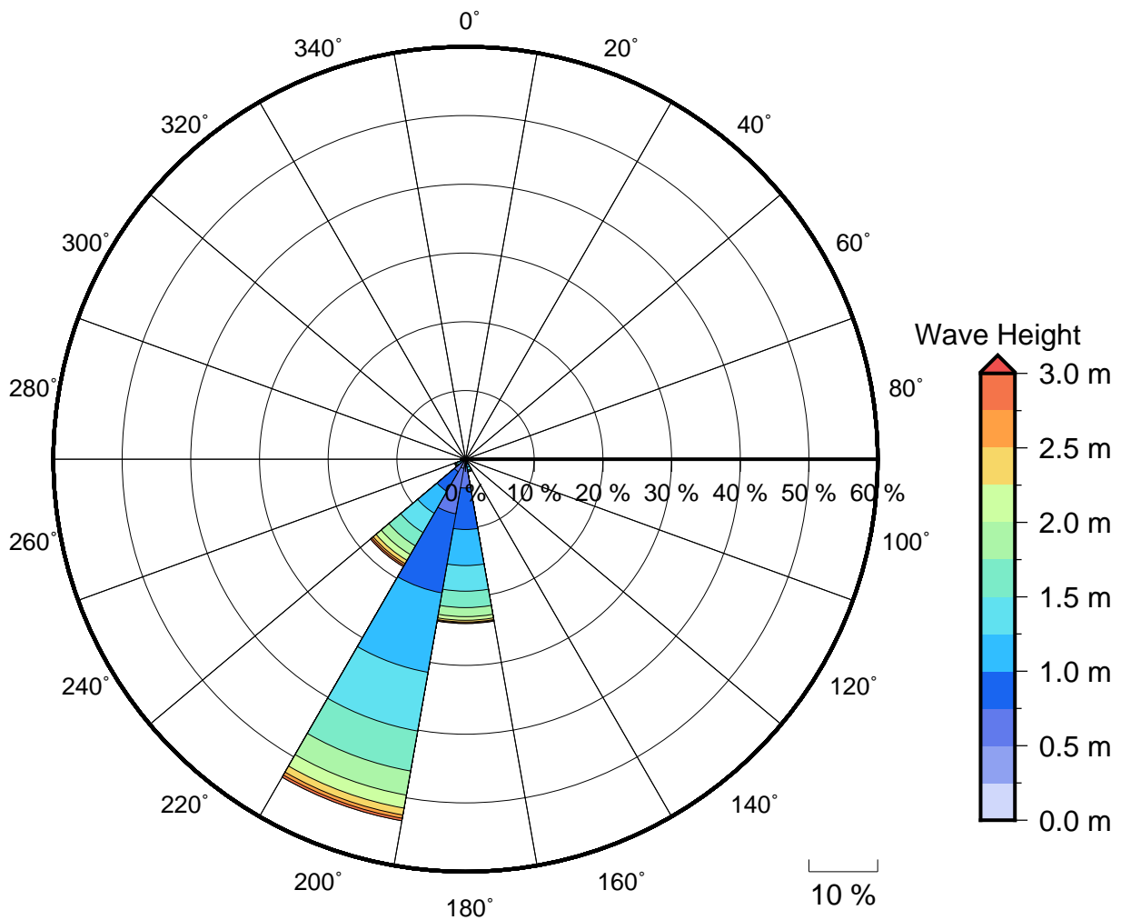
Figure 2 Annual wave rose for Natadola. Note that direction are where the wave are coming from.
