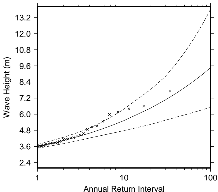
Figure 9 Extreme wave distribution for Natadola. The crosses represents the wave events that occurred since 1979. The plain line is the statistical distribution that best fit the past wave events. The dotted line show the upper and lower high confidence of the fit, there is a 95% chance that the fitted distribution lie between the two dashed lines.
