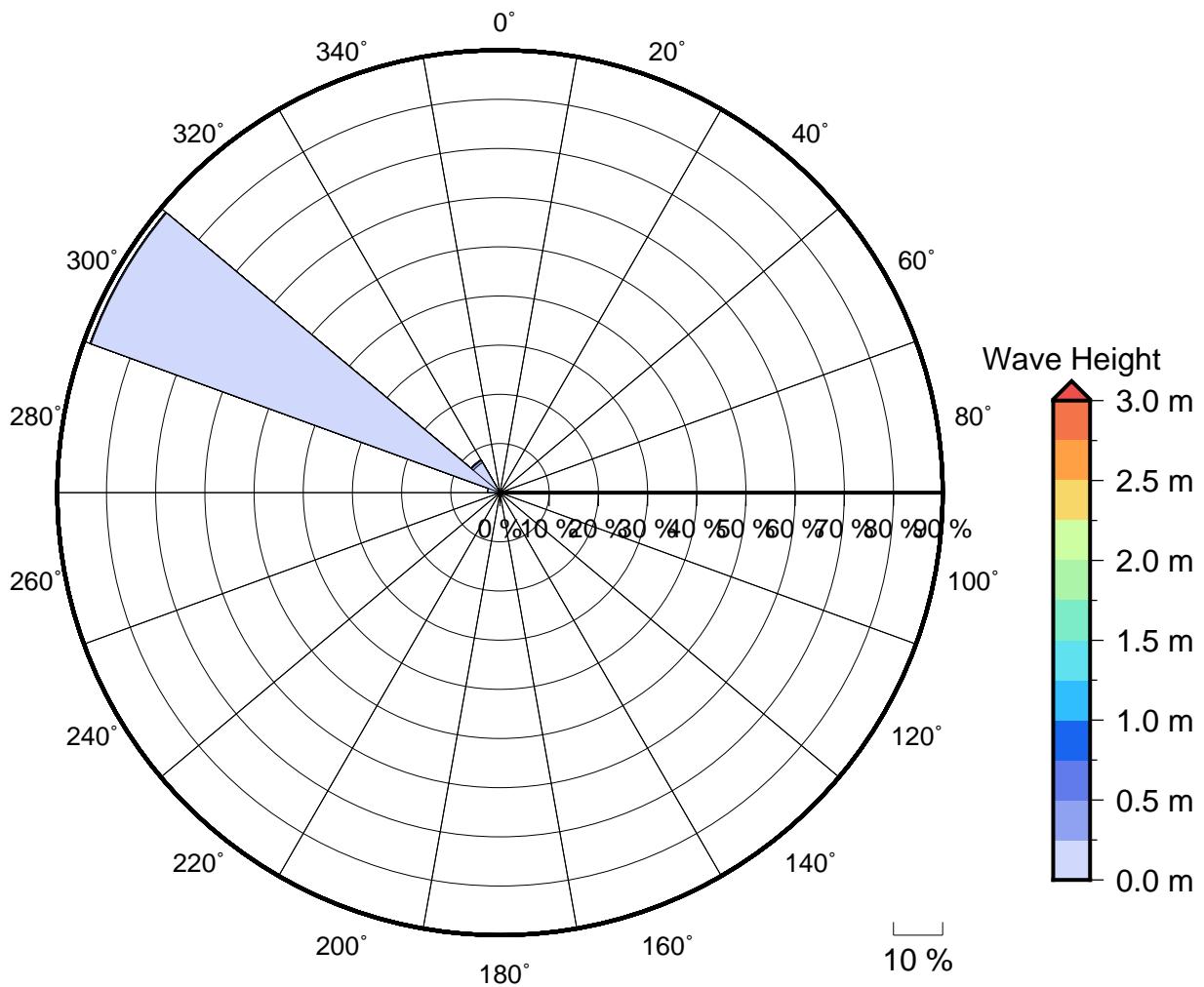
Figure 2 Annual wave rose for Nasoso. Note that direction are where the wave are coming from.
