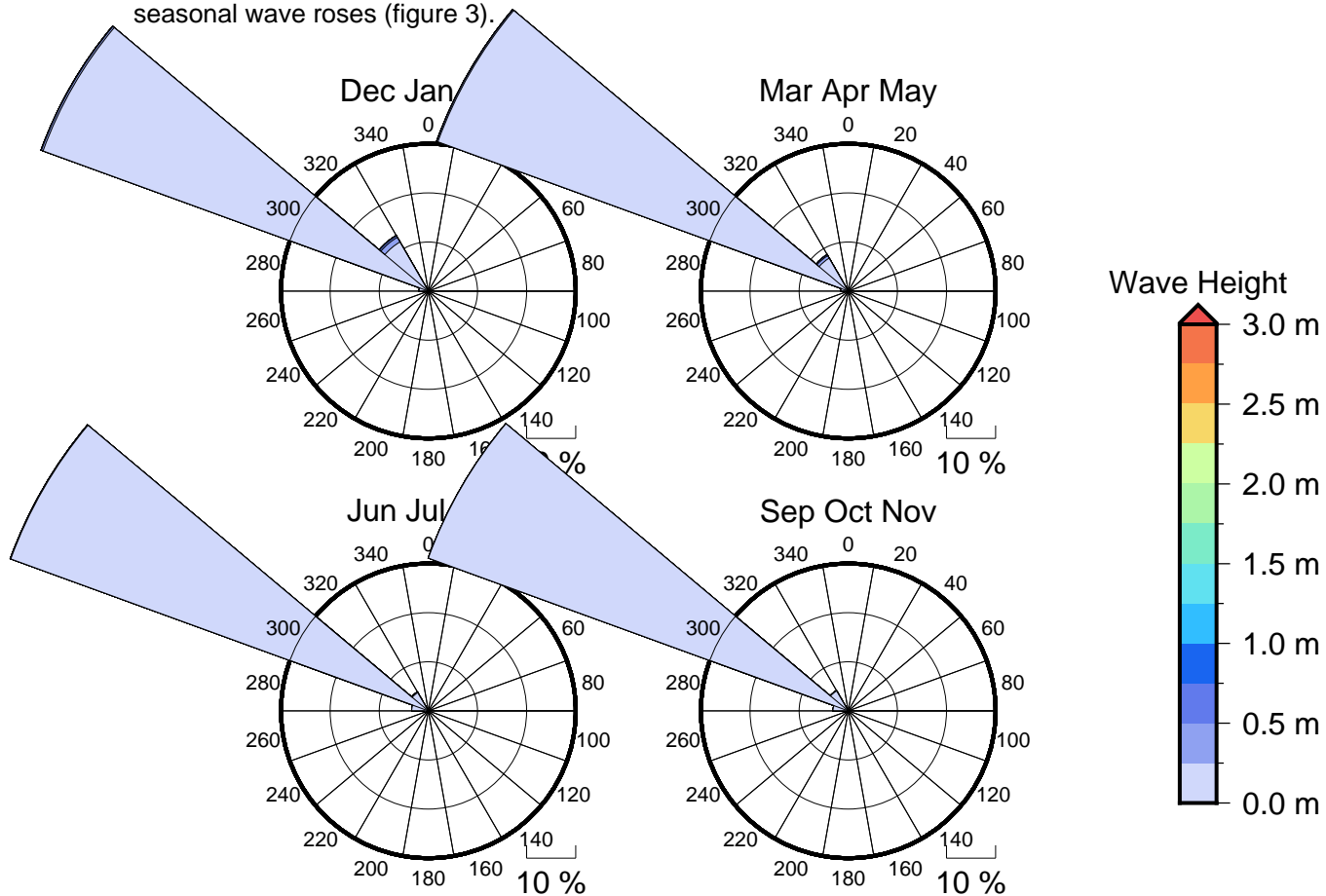
Figure 3 Seasonal wave roses for Nasoso
