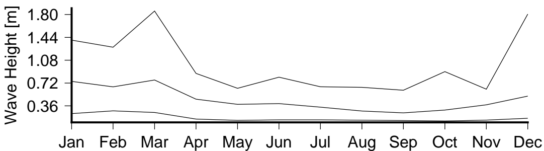
Figure 7 Monthly variation in large waves (90th percentile)(lower curve), severe waves (99th percentile) (middle curve) and the largest wave(upper curve) in Nasoso.
