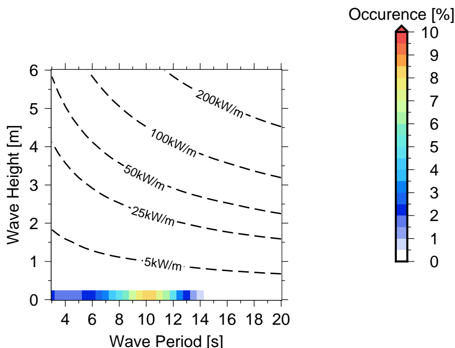
Figure 10 Occurrences of sea states in Nasoso .
