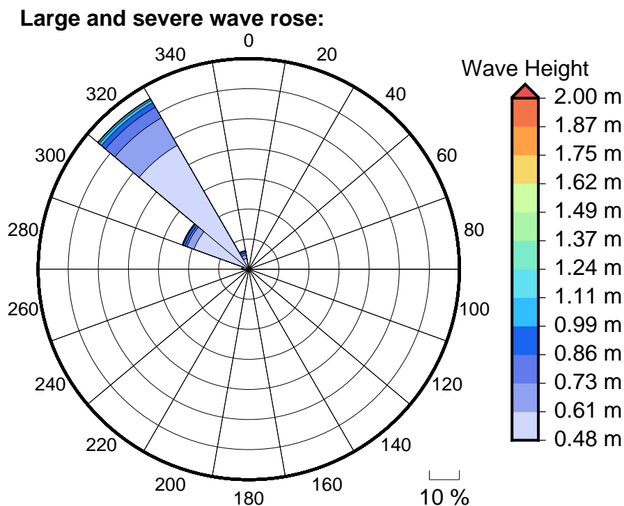
Figure 6 Large, severe and extreme wave roses for Nasoso
