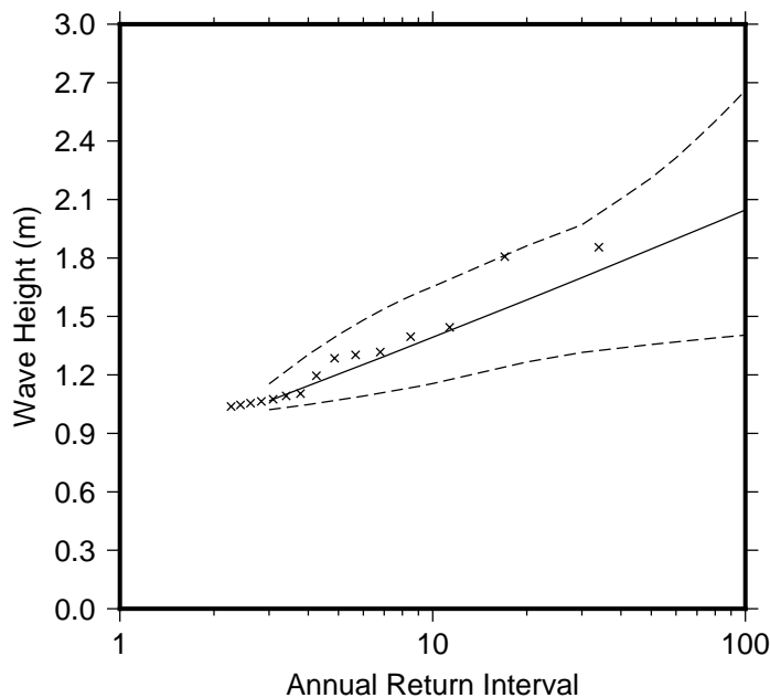
Figure 9 Extreme wave distribution for Nasoso. The crosses represents the wave events that occurred since 1979. The plain line is the statistical distribution that best fit the past wave events. The dotted line show the upper and lower high confidence of the fit, there is a 95% chance that the fitted distribution lie between the two dashed lines.
