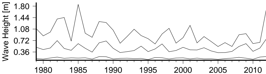
Figure 8 Annual variation in large waves (90th percentile)(lower curve), severe waves (99th percentile) (middle curve) and the largest wave(upper curve) in Nasoso.
