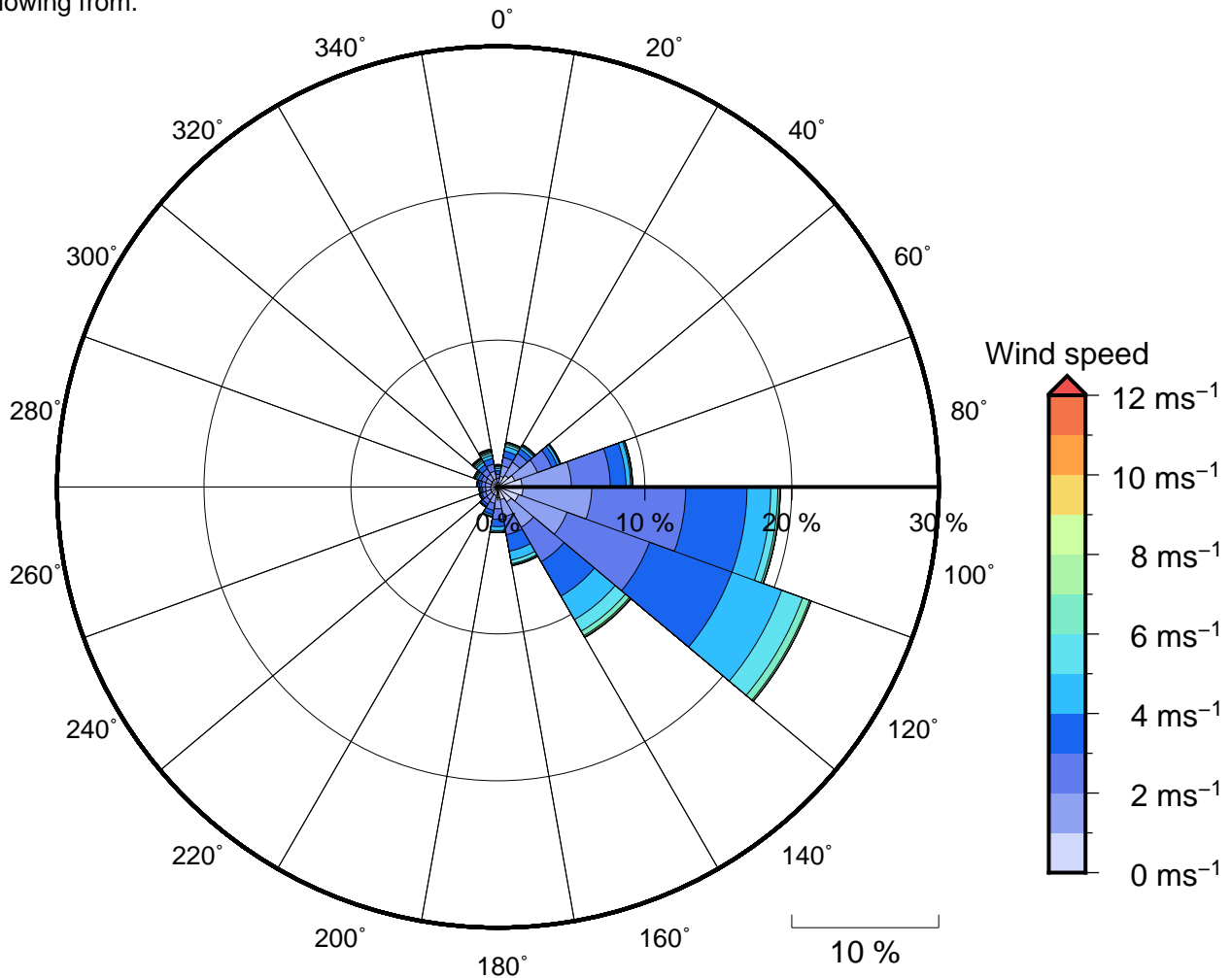
Figure 11 Annual wind rose for Nasoso. Note that directions are where the wind is coming from.
