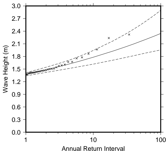
Figure 9 Extreme wave distribution for Narikoso. The crosses represents the wave events that occurred since 1979. The plain line is the statistical distribution that best fit the past wave events. The dotted line show the upper and lower high confidence of the fit, there is a 95% chance that the fitted distribution lie between the two dashed lines.
