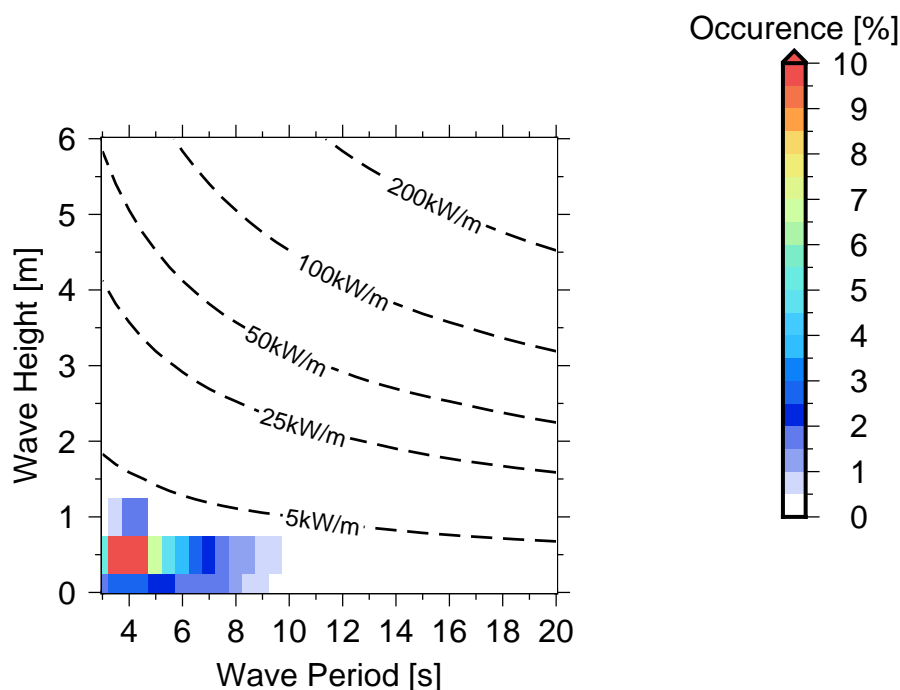
Figure 10 Occurrences of sea states in Narikoso .
