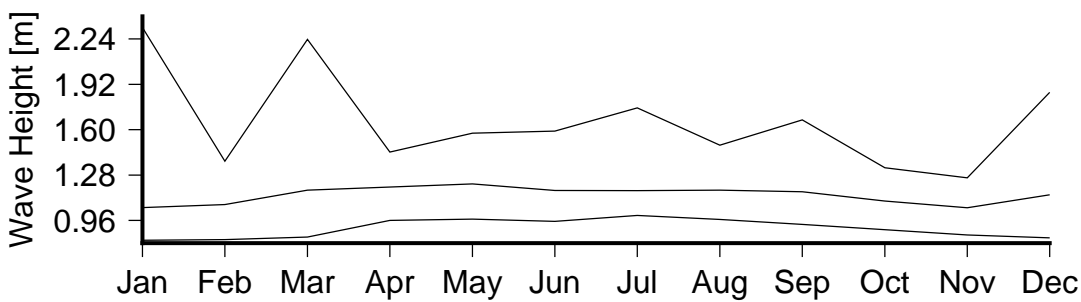
Figure 7 Monthly variation in large waves (90th percentile)(lower curve), severe waves (99th percentile) (middle curve) and the largest wave(upper curve) in Narikoso.
