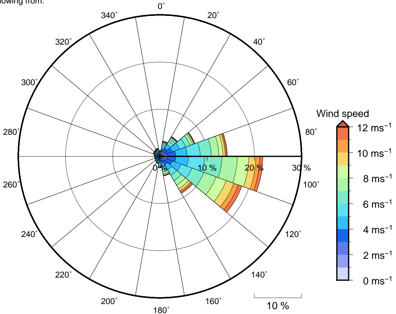
Figure 11 Annual wind rose for Narikoso. Note that directions are where the wind is coming from .
