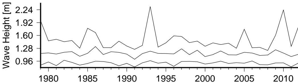
Figure 8 Annual variation in large waves (90th percentile)(lower curve), severe waves (99th percentile) (middle curve) and the largest wave(upper curve) in Narikoso.
