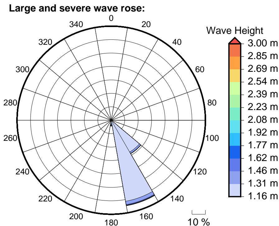
Figure 6 Large, severe and extreme wave roses for Narikoso
