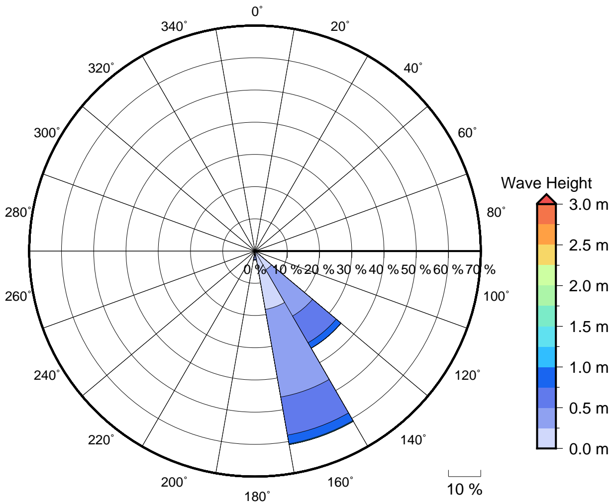
Figure 2 Annual wave rose for Narikoso. Note that direction are where the wave are coming from.
