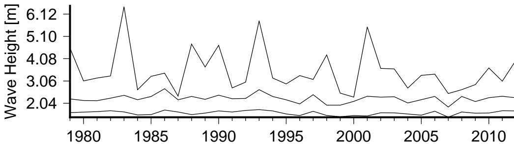
Figure 8 Annual variation in large waves (90th percentile)(lower curve), severe waves (99th percentile) (middle curve) and the largest wave(upper curve) in Namatakula.
