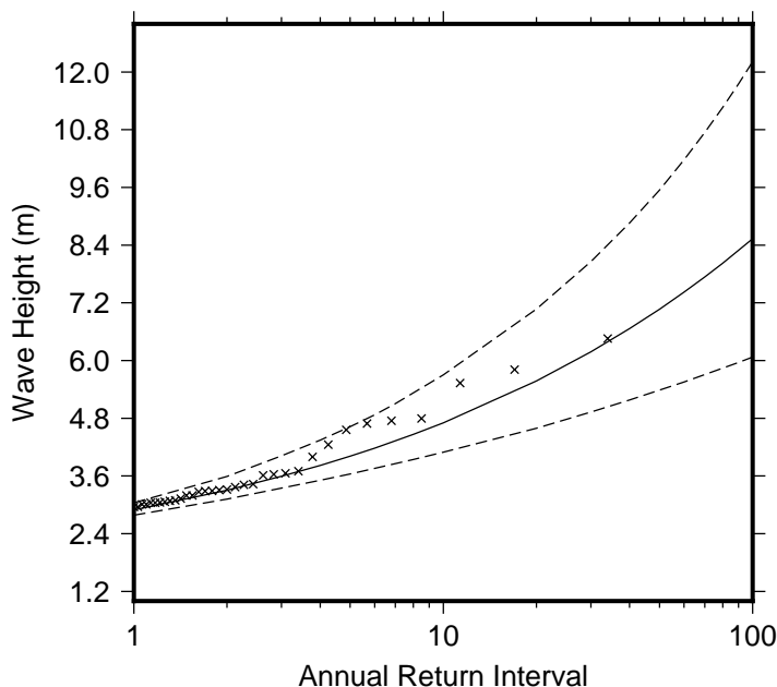
Figure 9 Extreme wave distribution for Namatakula. The crosses represents the wave events that occurred since 1979. The plain line is the statistical distribution that best fit the past wave events. The dotted line show the upper and lower high confidence of the fit, there is a 95% chance that the fitted distribution lie between the two dashed lines.
