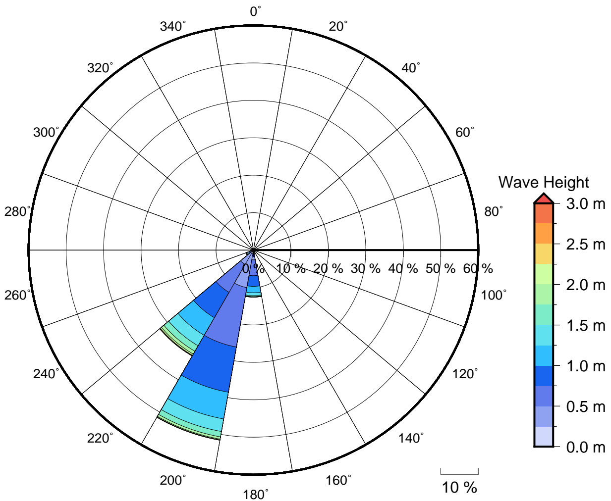
Figure 2 Annual wave rose for Namatakula. Note that direction are where the wave are coming from
