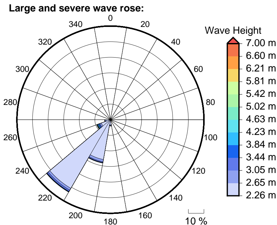
Figure 6 Large, severe and extreme wave roses for Namatakula
