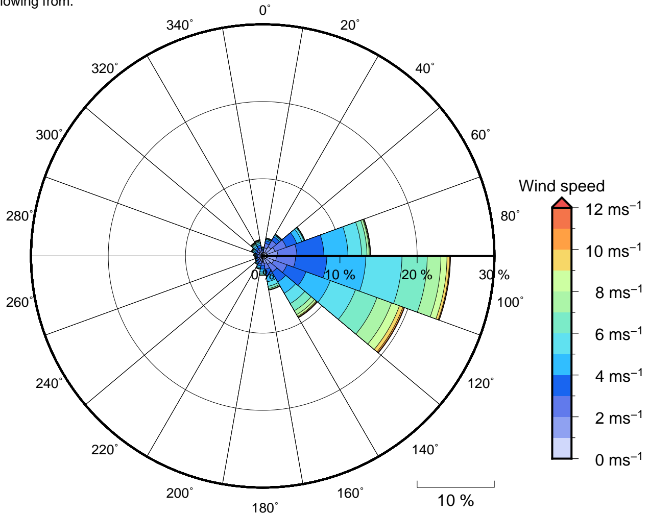
Figure 11 Annual wind rose for Namatakula. Note that directions are where the wind is coming from.
