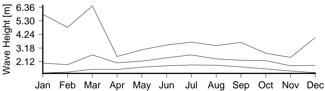
Figure 7 Monthly variation in large waves (90th percentile)(lower curve), severe waves (99th percentile) (middle curve) and the largest wave(upper curve) in Namatakula.
