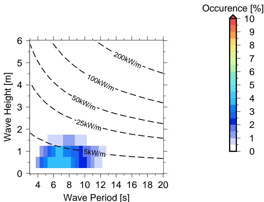
Figure 10 Occurrences of sea states in Namatakula .
