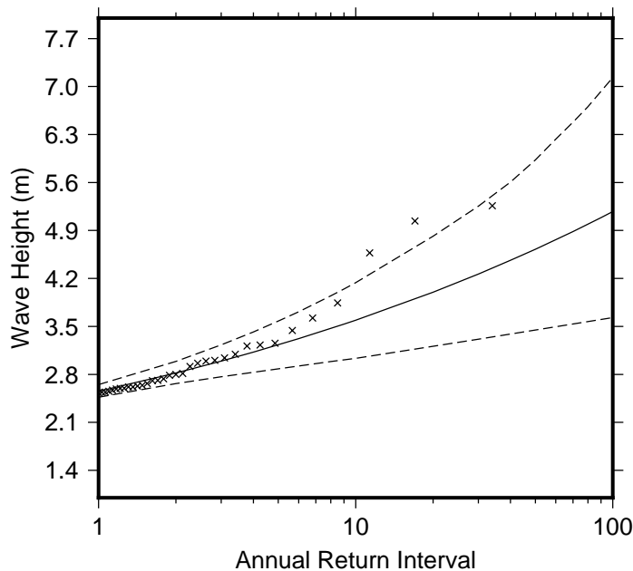
Figure 9 Extreme wave distribution for Maui Bay. The crosses represents the wave events that occurred since 1979. The plain line is the statistical distribution that best fit the past wave events. The dotted line show the upper and lower high confidence of the fit, there is a 95% chance that the fitted distribution lie between the two dashed lines.
