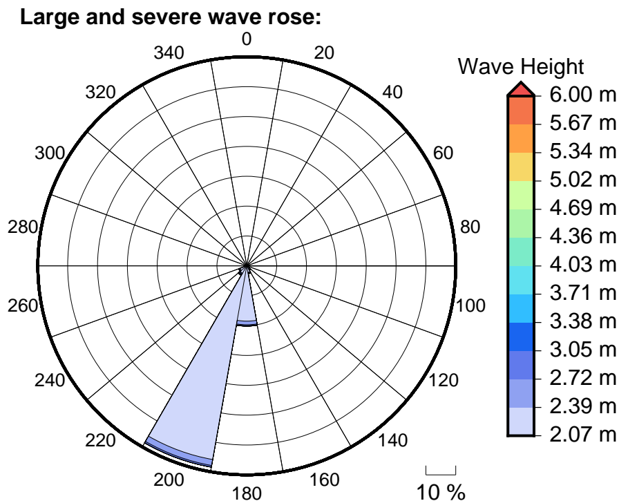
Figure 6 Large, severe and extreme wave roses for Maui Bay
