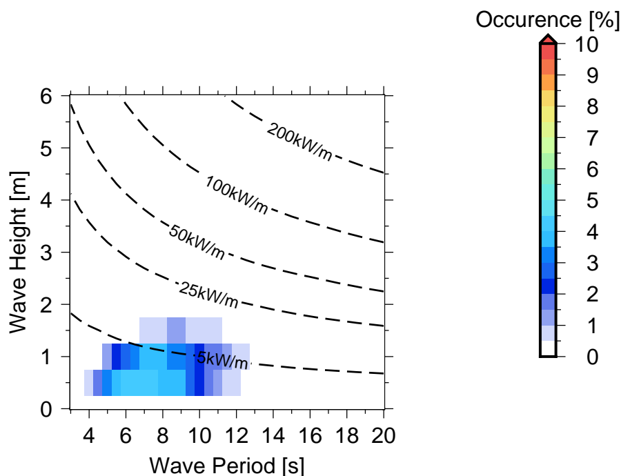
Figure 10 Occurences of sea states in Maui Bay .
