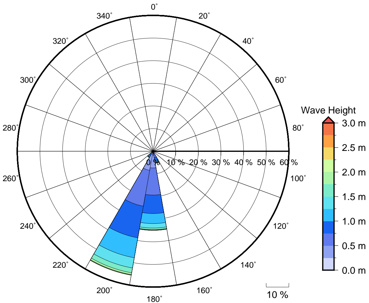
Figure 2 Annual wave rose for Maui Bay. Note that direction are where the wave are coming from.
