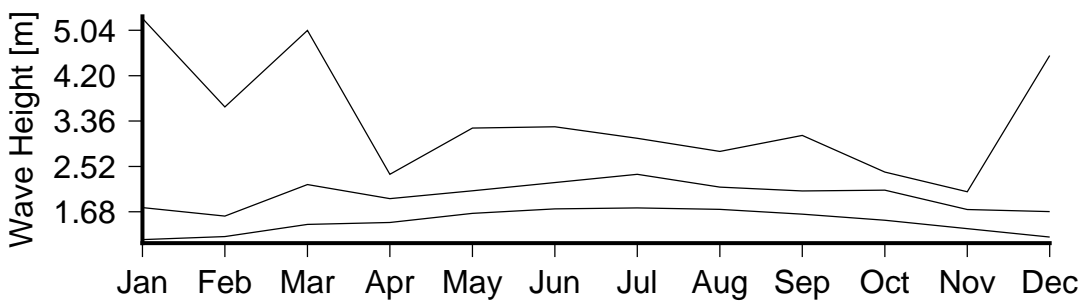
Figure 7 Monthly variation in large waves (90th percentile)(lower curve), severe waves (99th percentile) (middle curve) and the largest wave(upper curve) in Maui Bay.
