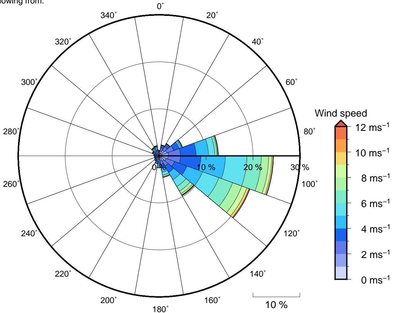
Figure 11 Annual wind rose for Maui Bay. Note that directions are where the wind is coming from.
