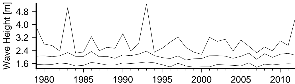
Figure 8 Annual variation in large waves (90th percentile)(lower curve), severe waves (99th percentile) (middle curve) and the largest wave(upper curve) in Maui Bay.
